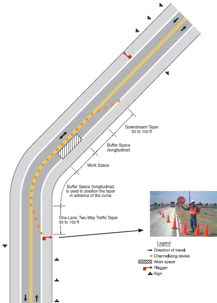
Figure 6C-3. Example of a One-Lane, Two-Way Traffic Taper
