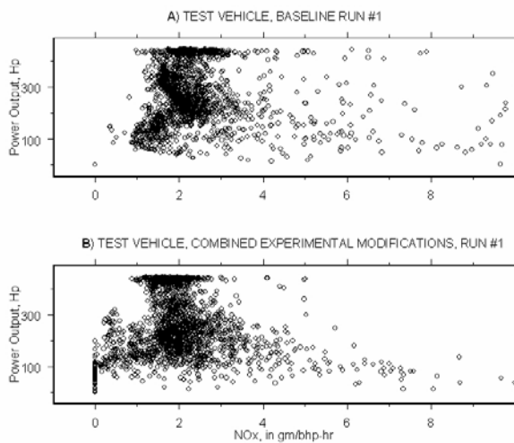
Figure 8: Comparison of NOx-power relationship of the test vehicles under (A) Baseline conditions (no experimental modifications) and (B) the combined experimental modifications (single wide tires and trailer aerodynamics).
