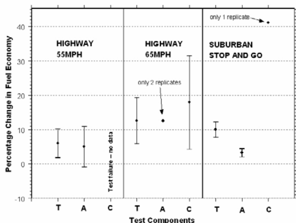
Figure 4: Percentage change in fuel economy (with 95 percent confidence intervals) as a result of the experimental modification, labeled as follows: T – single wide tires only; A – trailer aerodynamics (fairings) only; C – both single wide tires and trailer aerodynamics.
