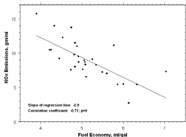
Figure 7: Relation between fuel economy and NOx emissions as measured in the test vehicle.
