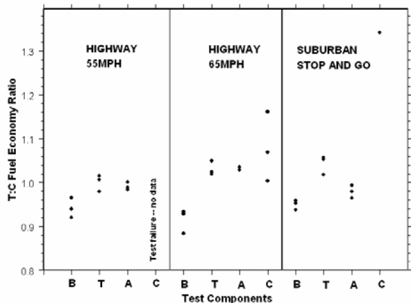
Figure 3: Fuel economy test results grouped by drive cycle and experimental modification, labeled as follows: B – baseline; T – single wide tires only; A – trailer aerodynamics (fairings) only; C – both single wide tires and trailer aerodynamics.
