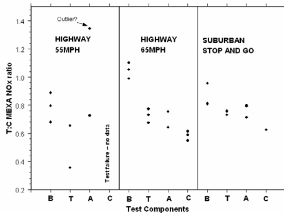
Figure 5: NOx test results grouped by drive cycle and experimental modifications, labeled as follows: B – baseline; T – single wide tires only; A – trailer aerodynamics (fairings) only; C – both single wide tires and trailer aerodynamics.
