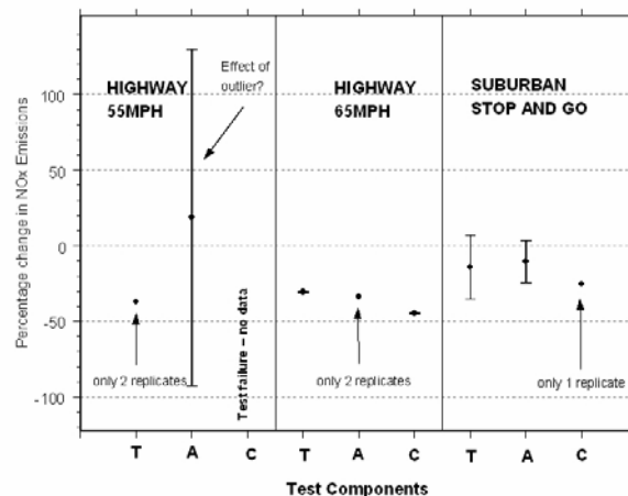
Figure 6: Percentage change in NOx emissions as a result of the experimental modifications, labeled as follows: T – single wide tires only; A – trailer aerodynamics (fairings) only; C – both single wide tires and trailer aerodynamics.
