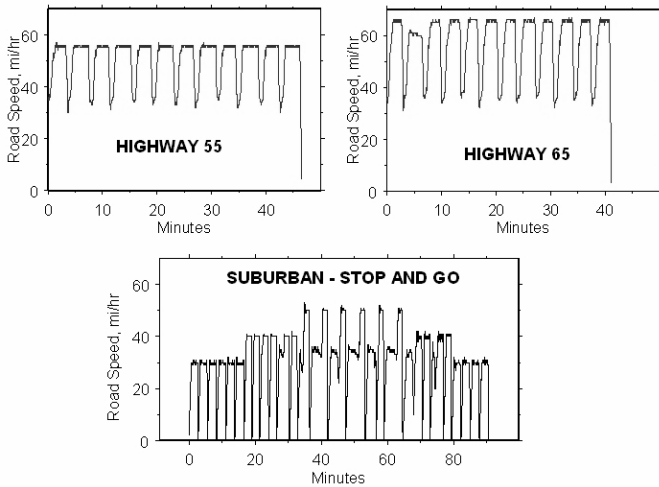
Figure 1: Speed traces of drive cycles tested
