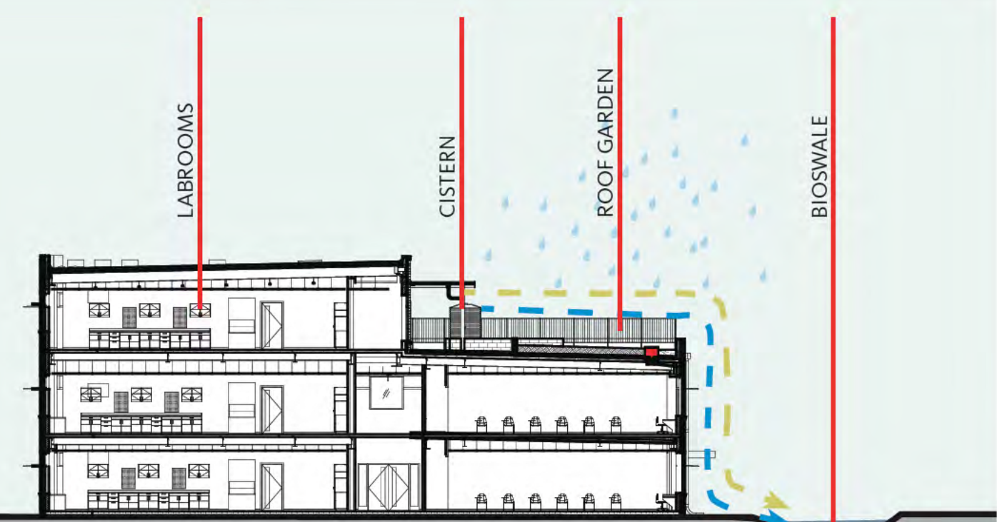
SECTION - RAINWATER CONCEPT
