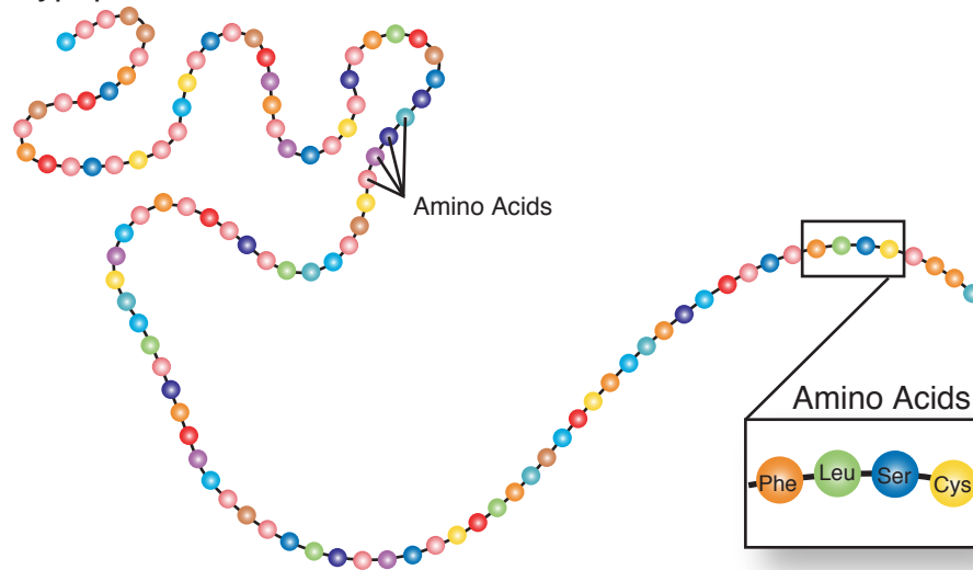
Polypeptide Chain
