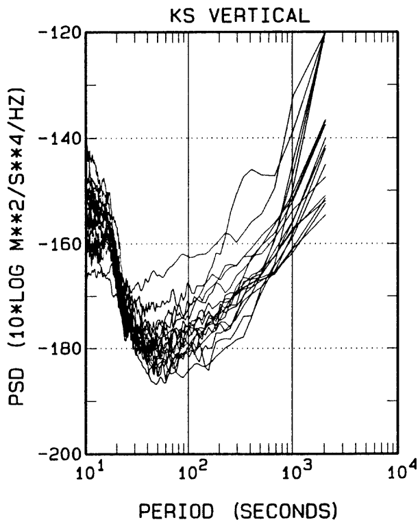
Figure 7. --Overlays of the STS and KS LP spectra. Vertical-component STS-1 spectra are in the upper left, horizontal STS-1 spectra in the upper right, vertical-component KS spectra in the lower left, and KS horizontal spectra in the lower right. The data were recorded during quiet, relatively wind-free periods.
