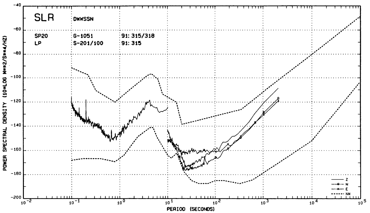
Figure A73.--Noise spectra from the Silverton, South Africa DWWSSN station.
