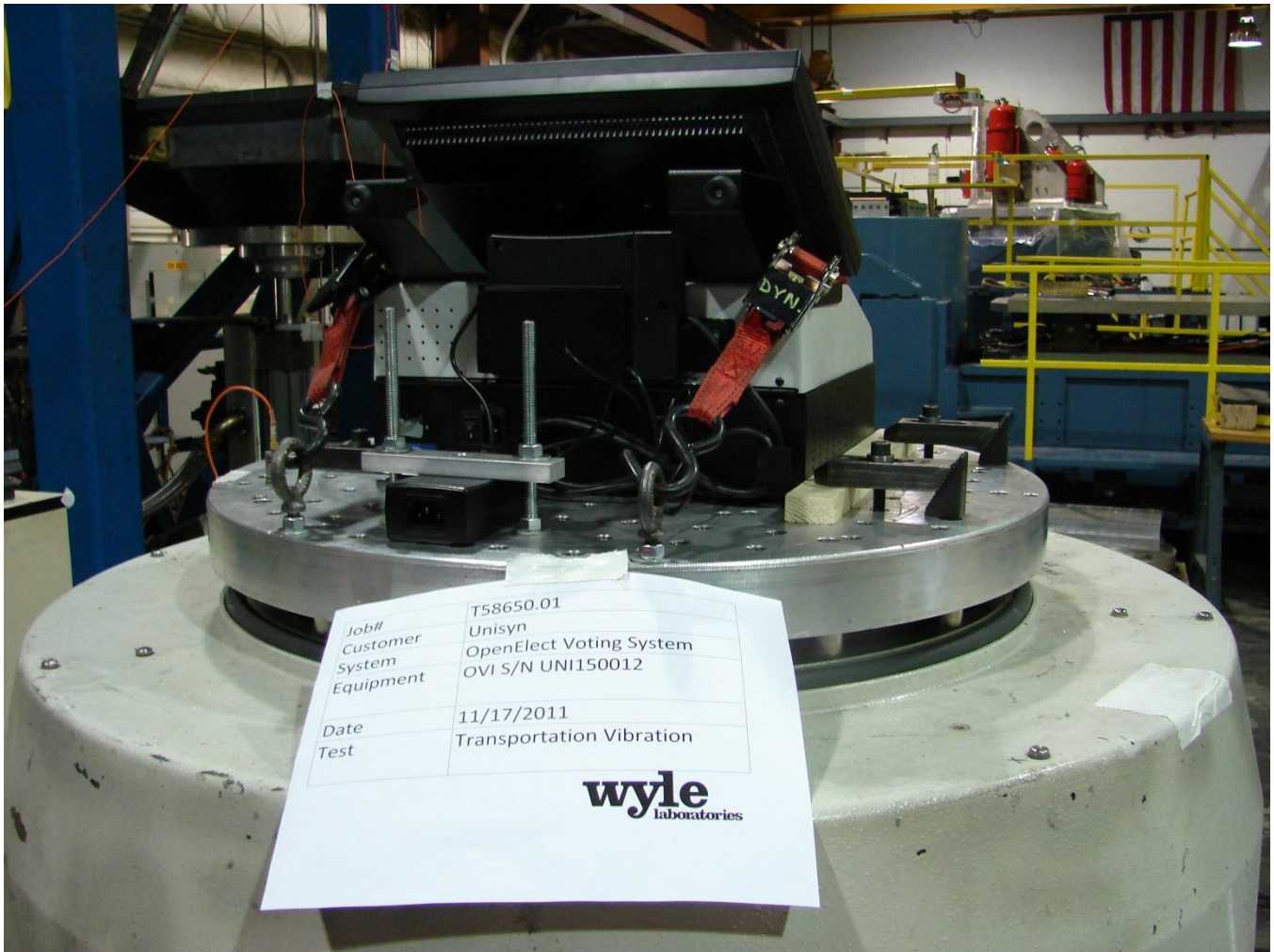
Photograph No. 82 OpenElect Voting System OVI S/N UNI150012
