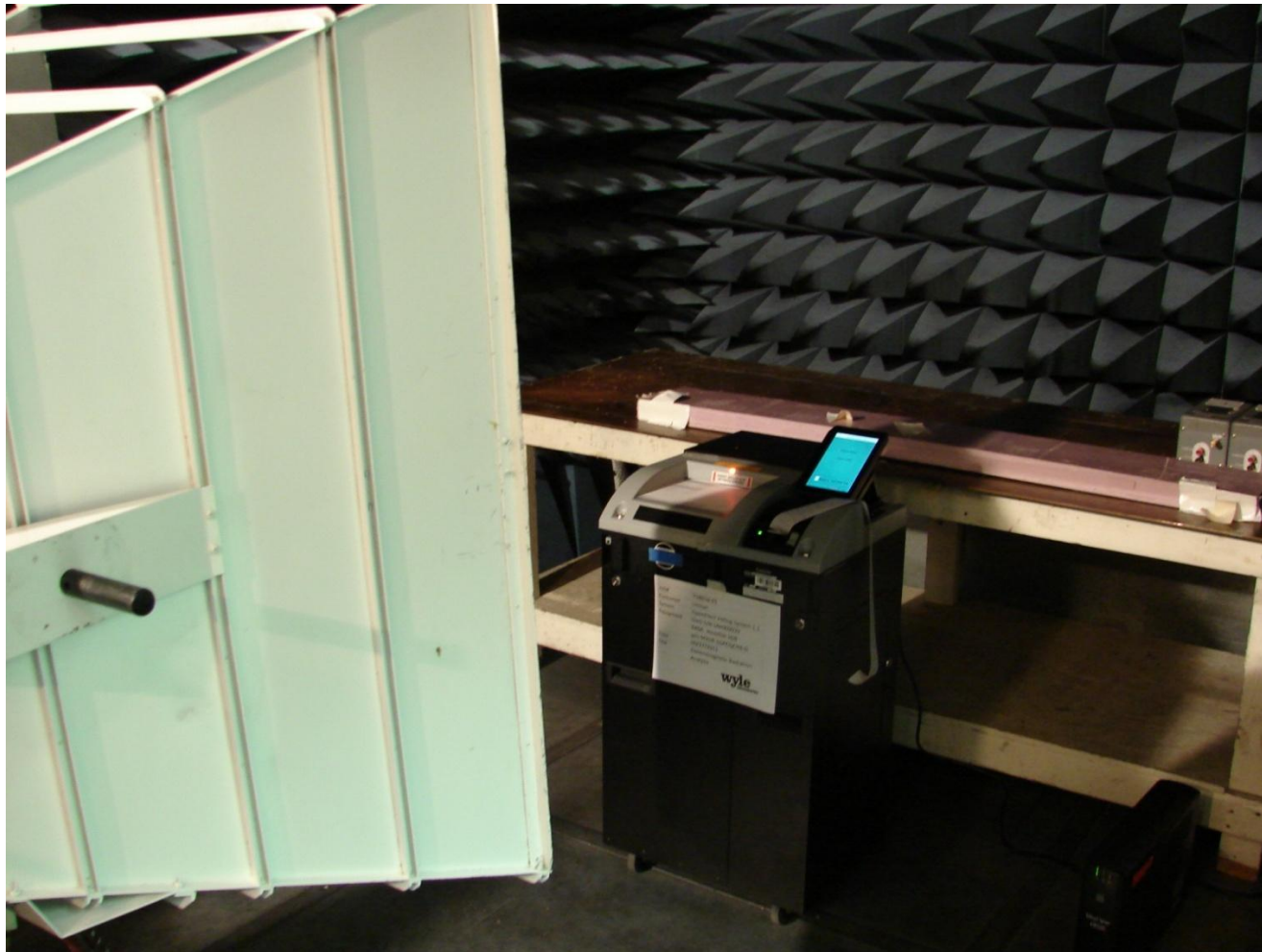
Photograph No. 13 Electromagnetic Radiation Analysis - 3
