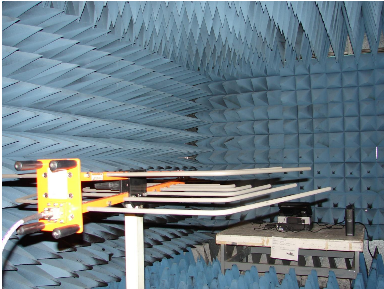
Photograph No. 15 Electromagnetic Susceptibility - 1
