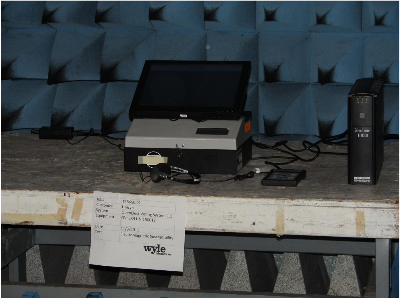
Photograph No. 18 Electromagnetic Susceptibility – 4
