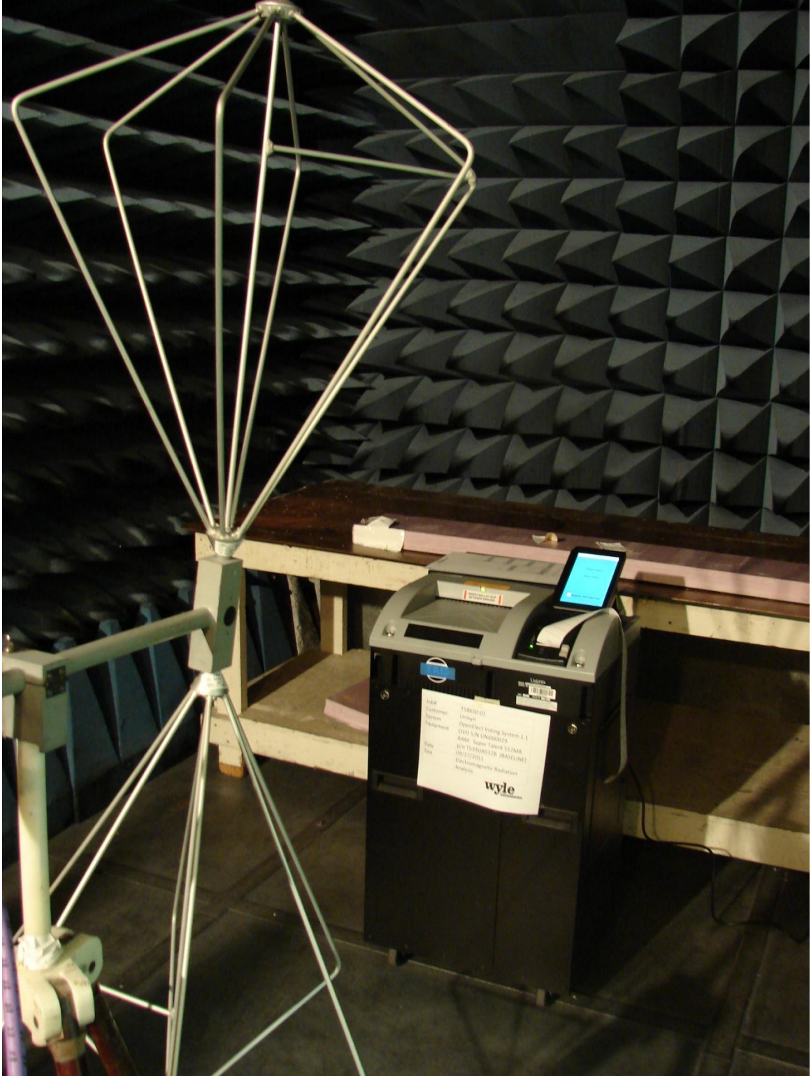
Photograph No. 14 Electromagnetic Radiation Analysis – 4
