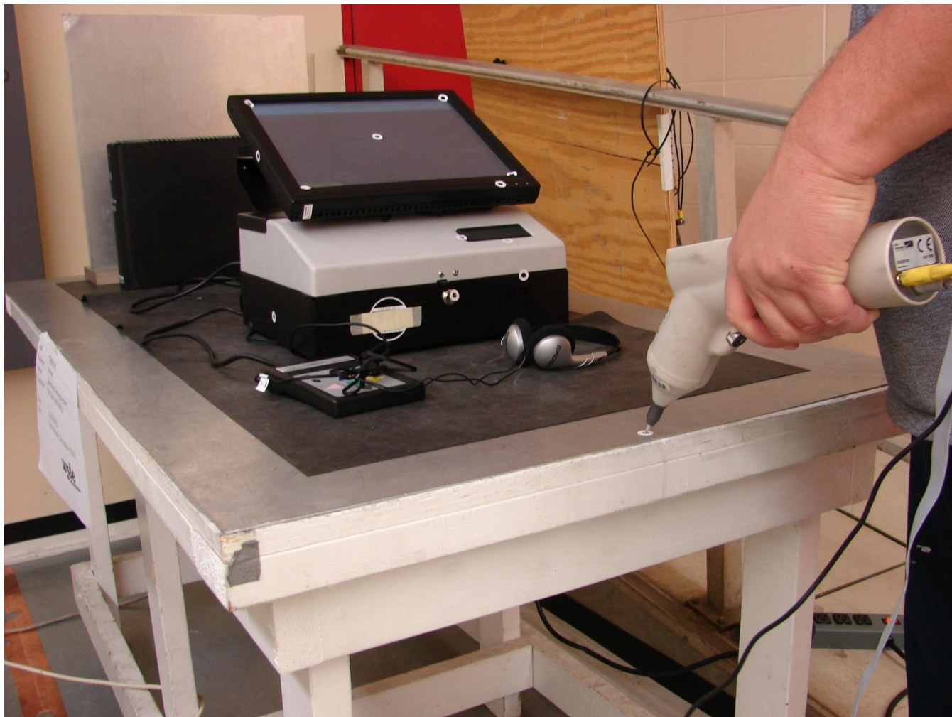
Photograph No. 24 ESD-5
