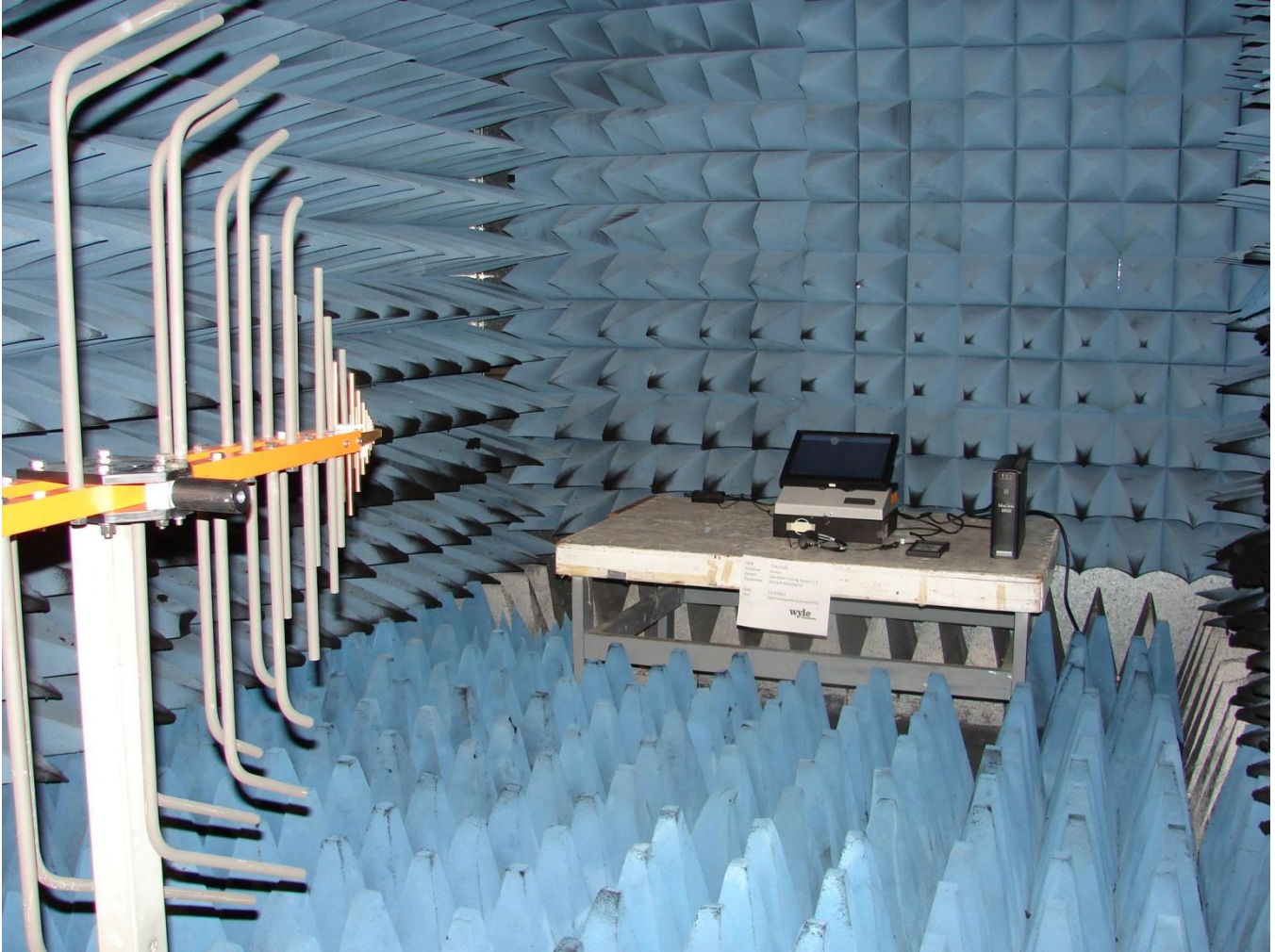
Photograph No. 17 Electromagnetic Susceptibility - 3
