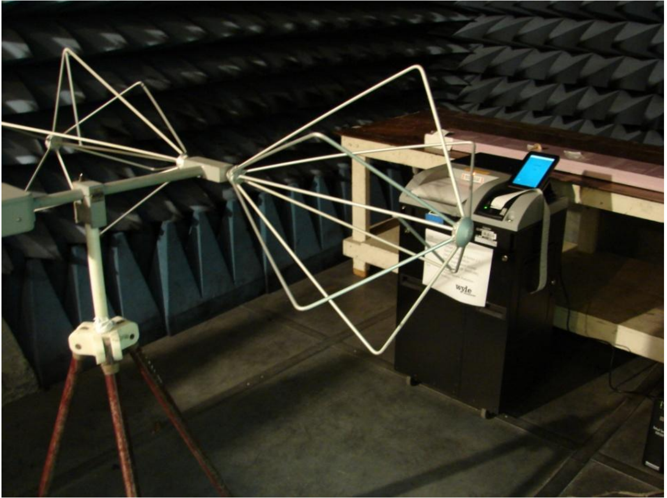
Photograph No. 11 Electromagnetic Radiation Analysis – 1
