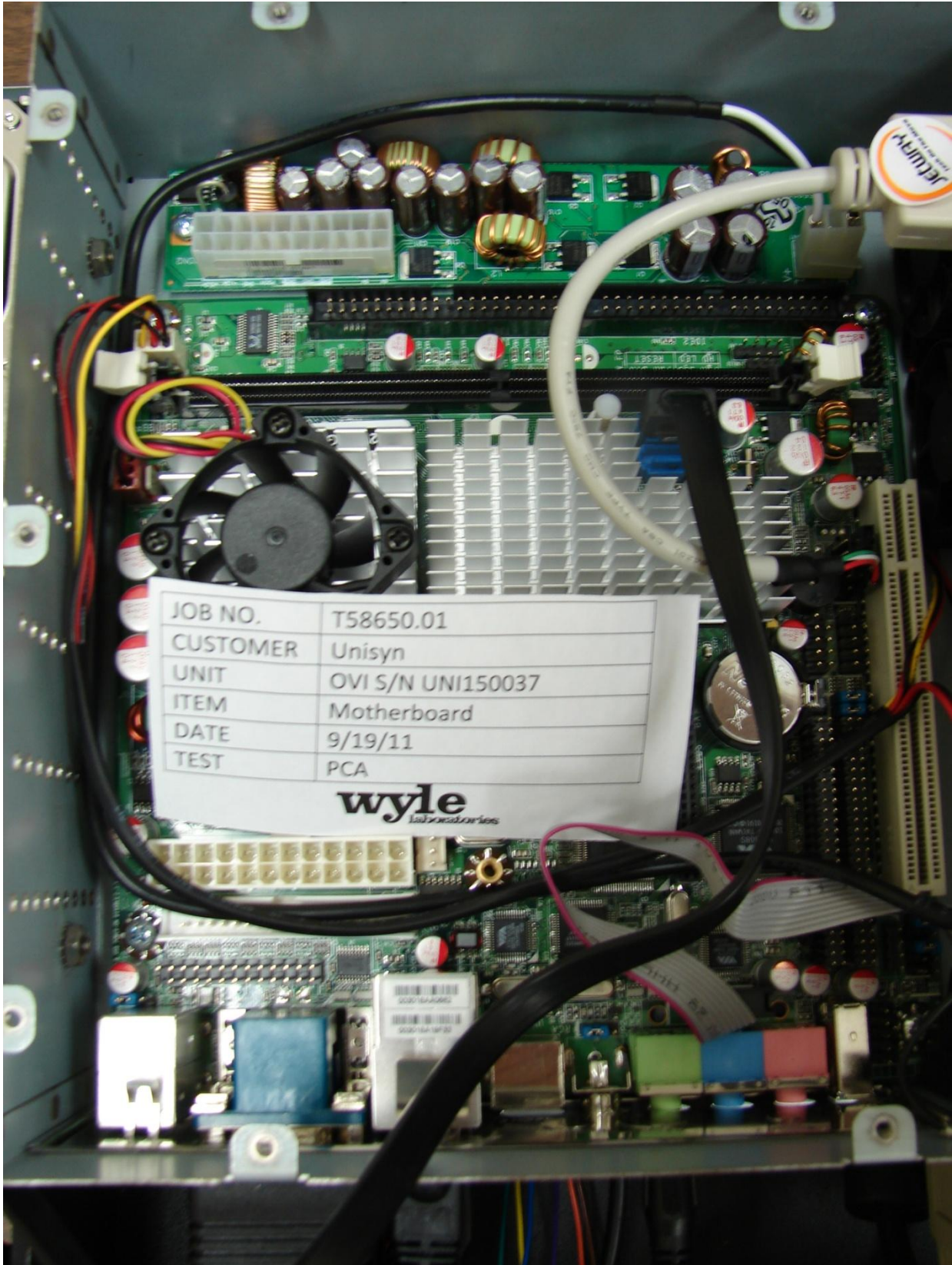
Photograph No. 73 OVI S/N UNI150037 - Motherboard
