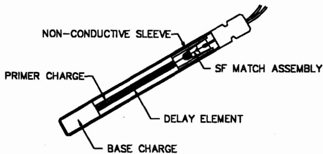
Figure 4.2 Delay Electric Blasting Caps
