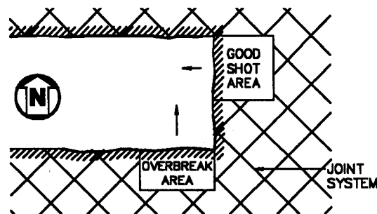
Figure 9.1 Regional Jointing Pattern
