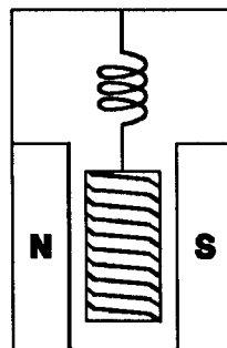
Figure 10.7 Sensor Mechanism
