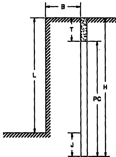
Figure 6.1 Symbols for Blast Design
