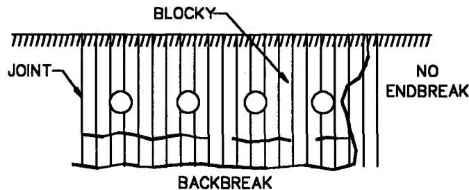
Figure 9.3 Dominant Joints Perpendicular to the Face
