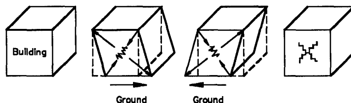
Figure 10.23 Vibration X - Crack Pattern
