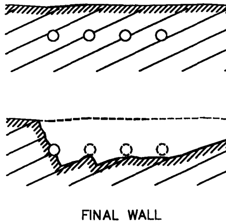
Figure 9.5 Dominant Joints at Acute Angles
