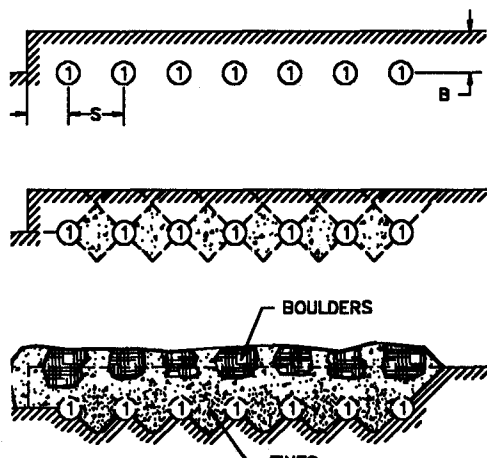
Figure 7.11 Single Row Alternating Delays, S = 1.4 B
