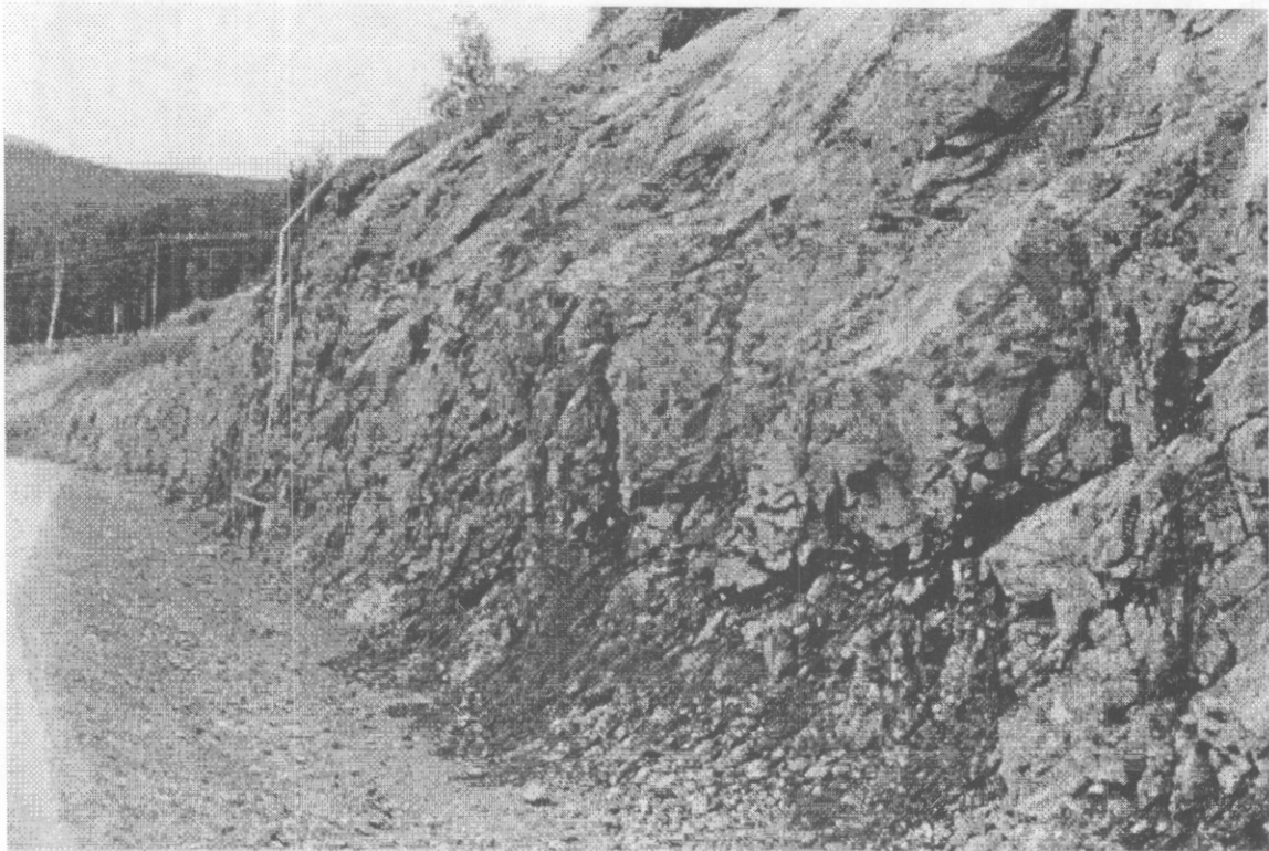
Figure 11.4A Blast Without Presplit (Siltstone, Alaska)
