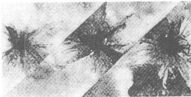
Figure 8.10 Presplit in Plexiglass with Joints at Angle with Face (after Worsey)
