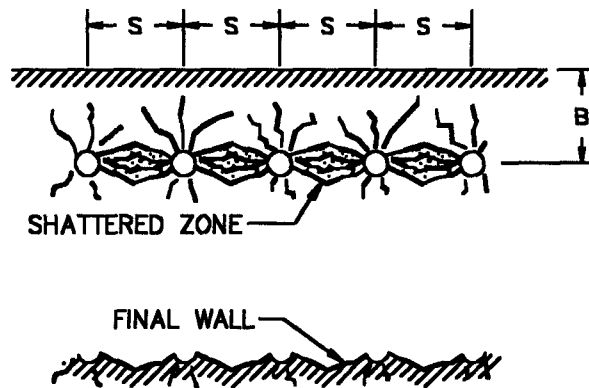
Figure 7.1 Shattered Zone from Close Spacing
