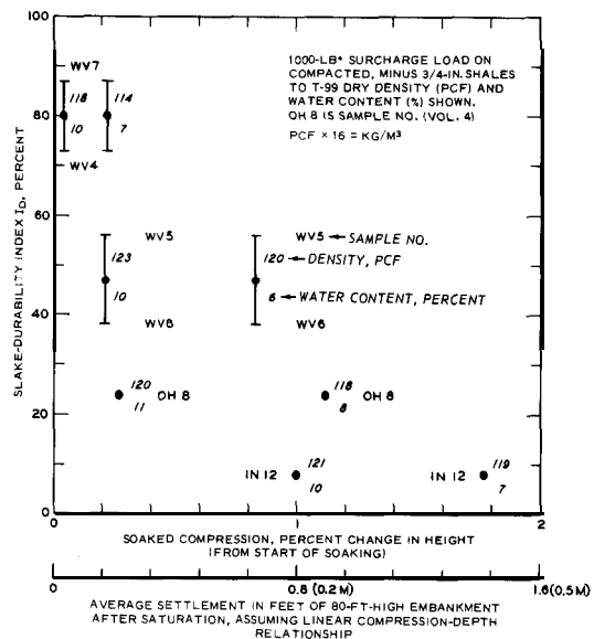
Figure 8. Soaked Compression of Minus 3/4-in. Compacted Shale Samples Related to Slake-Durability Index.
