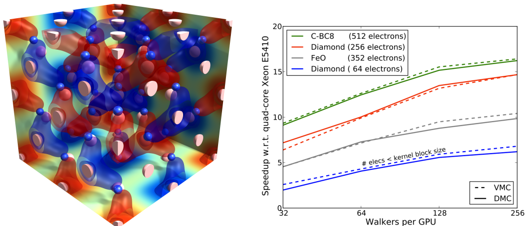
Figure 10-4. Left: Super cell of cubic boron nitride that can now be studied with QMC. Right: The code QMCPACK shows excellent scaling on a GPU and runs 10-15 times faster than on a quad-core Xeon processor using all four cores. (From K.P. Esler, J. Kim, D. M. Ceperley, “Fully accelerating quantum Monte Carlo simulations of real materials on GPUs”, GP-GPU conference).
