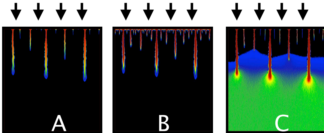
Figure 8-2. Concentration (A), aperture (B) and flow fields (C) in a narrow fracture.
