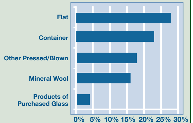
Estimated Energy Share of Direct Production Costs by Glass Sector, 2006
