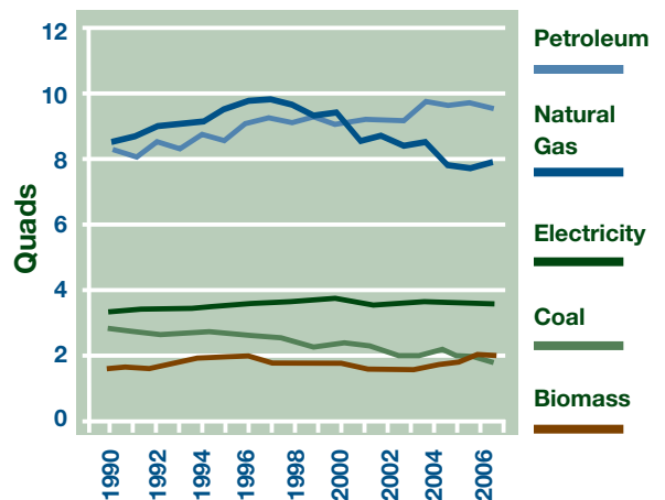
INDUSTRIAL ENERGY CONSUMPTION BY SOURCE, 1990-2007
