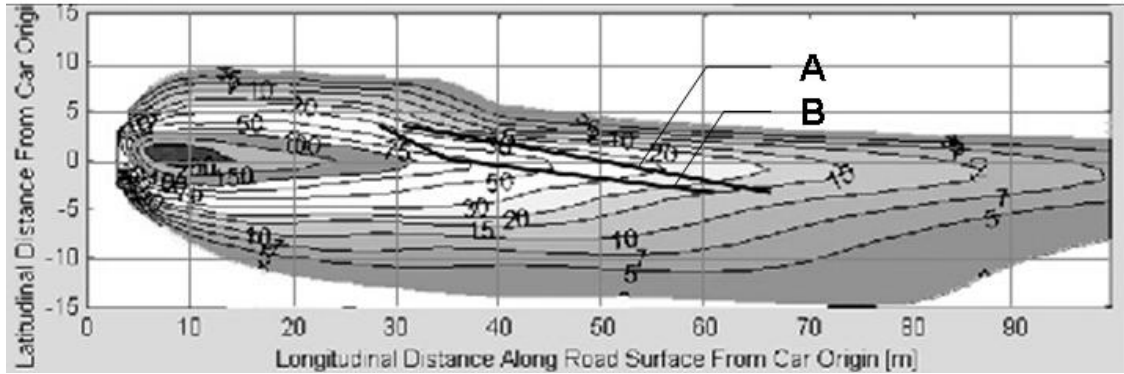
(a) HID headlamp system B
