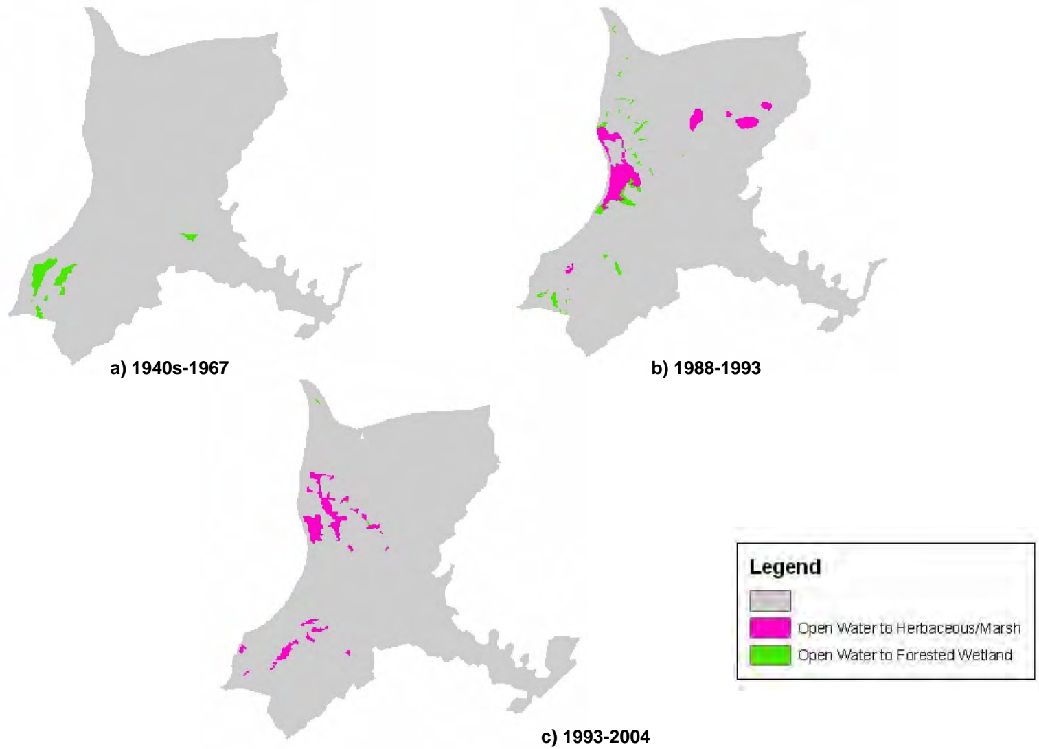
Figure 14(a-c). Change in open water within Rat Bay and surrounding areas from a) 1940s-1967, b) 1988-1993 and c) 1993-2004.
