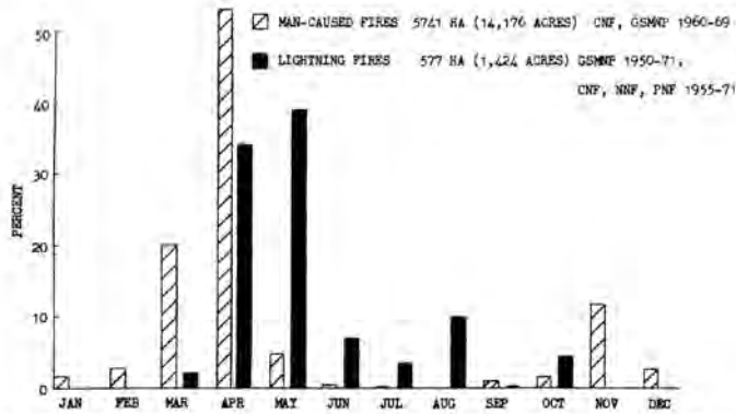
FIG. 2. Incidence of wildfires in the Appalachians of Tennessee and North Carolina
