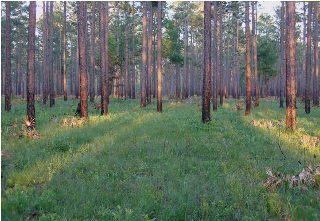
Figure 22. Annually burned Mascotte series at Fort Stewart. Dominant grass at this location is Muhlenbergia expansa .
