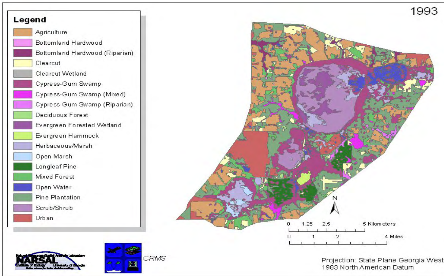
Figure 2e. Grand Bay-Banks Lake (GBBL) ecosystem land cover: 1993.
