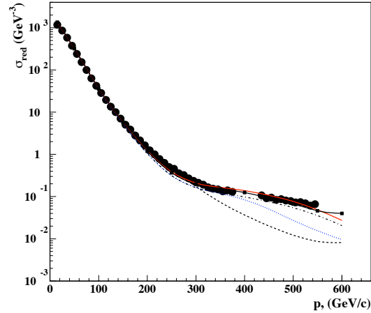
Figure 1: The reduced cross section for a beam energy of 3.1095 GeV, Q^2 = 0.665 (GeV/c) ^2 , x_{Bj} = 0.964 , and \phi_p = 180^\circ . The data are from [11].
