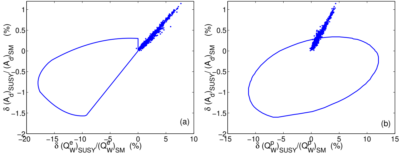
FIG. 4: 95 % CL allowed region for RPV contribution to A_{PV}^{eD, \text{DIS}}(y = 1, Q^2 = 3.7 \text{ GeV}^2) vs. electron weak charge (left) and proton weak charge (right). The dots indicate the SUSY loop corrections.
