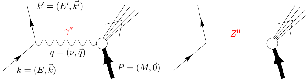
FIG. 3: Tree-level Feynman diagrams for electron scattering. The electron interacts with the target by exchanging either a virtual photon (left) or a Z^0 boson (right).
