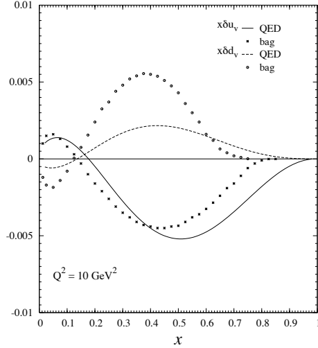
FIG. 8: Charge symmetry violating terms in valence parton distributions from QED splitting alone (solid, dashed) or from QCD effects (circle, square) calculated with a Bag Model. Each of these 4 curves will contribute, additively and with the same sign, to the numerator of R_{CSV} 39.
