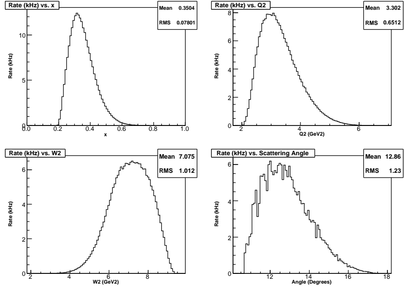
FIG. 6: Rate distribution plotted versus kinematic variables x , Q^2 , W^2 , and lab scattering angle for the assumed acceptance of the HMS spectrometer with central angle 13.5^\circ and central momentum 6.0 GeV.
