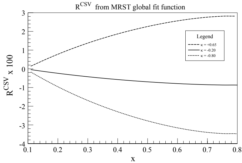
FIG. 10: Fractional change in A_d due to CSV in the MRST global fit [61]. The central value of the fit (CSV parameter \kappa = -0.2 ) suggests effects comparable to the proposed experimental uncertainties, but the 90% allowed region ( -0.8 < \kappa < +0.65 ) contains contributions 3-4 times larger.
