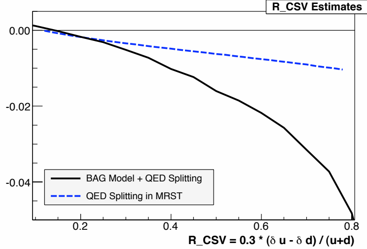
FIG. 9: Predictions for the fractional change in the parity-violating asymmetry \Delta A_d/A_d , plotted against x , for the proposed measurement. The MRST prediction [73] includes only QED splitting effects, while the Bag Model + QED splitting prediction [75] includes effects from both quark mass and charge differences.
