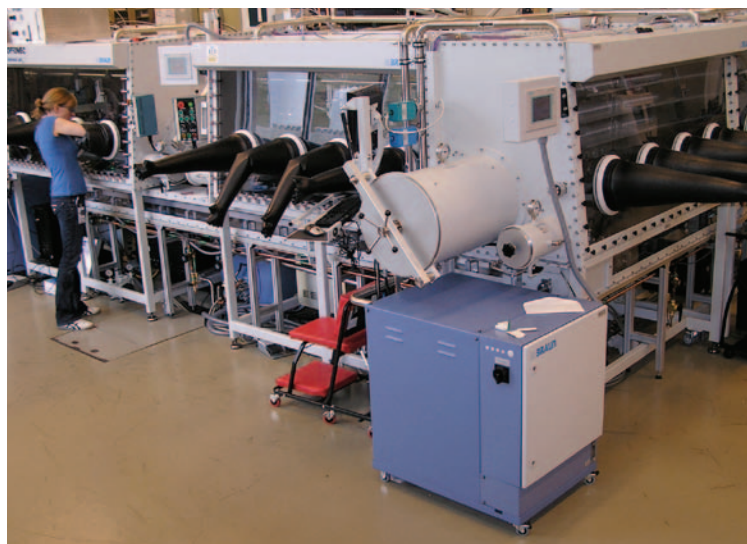
Part of NREL's Atmospheric Processing Platform, showing the spray deposition and inkjet printing units to the left and sample preparation and rapid thermal processing units to the right.
