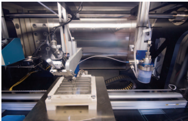
Close-up view of the inside of the inkjet printing unit.
