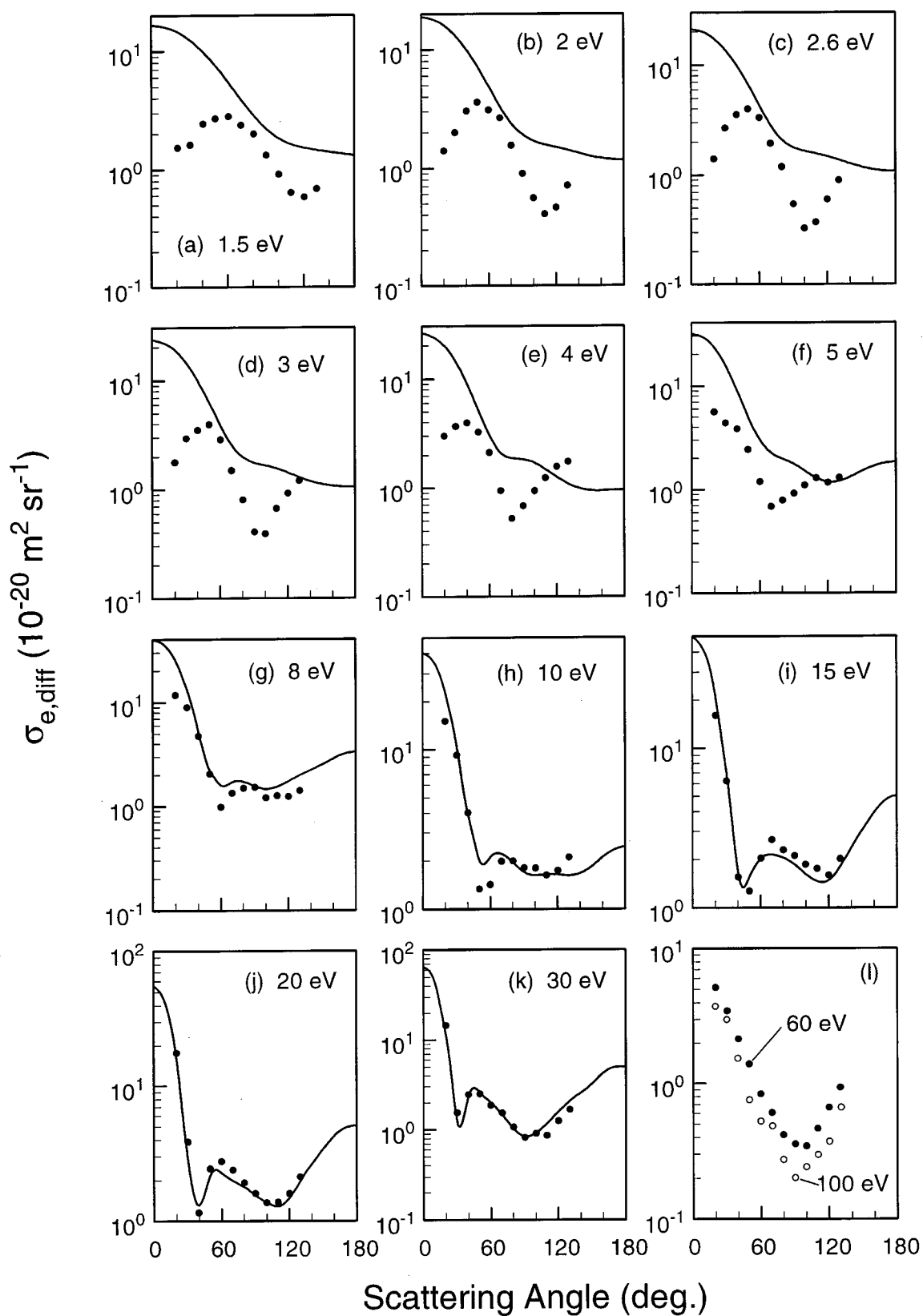
FIG. 3. Differential elastic electron scattering cross sections, \sigma_{e,diff} , for c -C 4 F 8 : (●,○) data of Tanaka and co-workers 60, 61 ; (—) calculations of McKoy et al. 62
