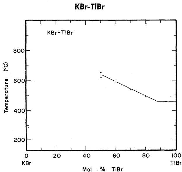
FIGURE 33. Temperature-composition phase diagram for KBr-TlBr.
