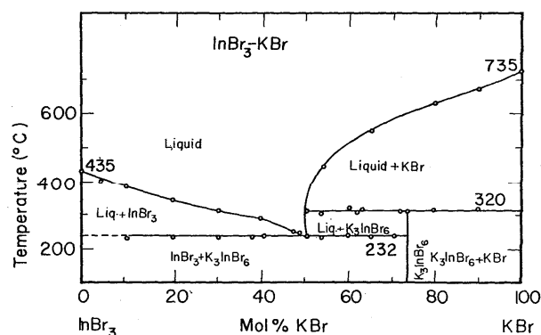
FIGURE 26. Temperature-composition phase diagram for InBr 3 -KBr.
