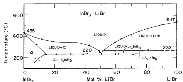
FIGURE 27. Temperature-composition phase diagram for InBr 3 -LiBr.
