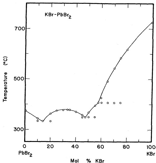
FIGURE 30. Temperature-composition phase diagram for KBr-PbBr 2 .
