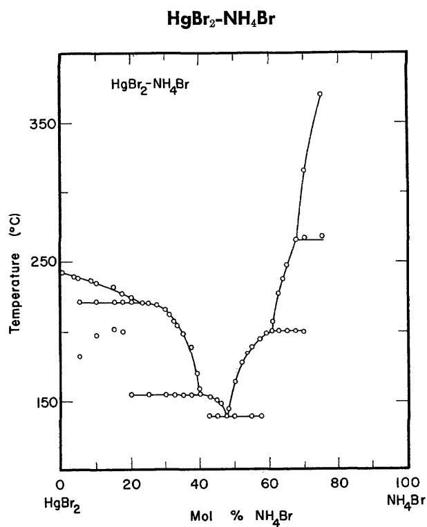
FIGURE 24. Temperature-composition phase diagram for \text{HgBr}_2\text{-NH}_4\text{Br} .
