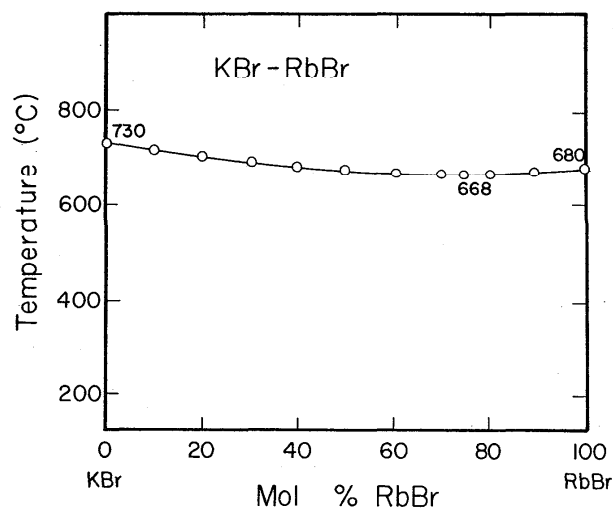
FIGURE 31. Temperature-composition phase diagram for KBr-RbBr.
