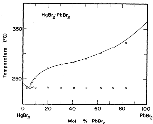
FIGURE 25. Temperature-composition phase diagram for HgBr 2 -PbBr 2 .
