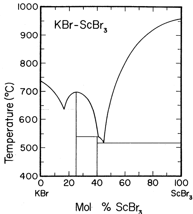
FIGURE 32. Temperature-composition phase diagram for KBr-ScBr 3 .
