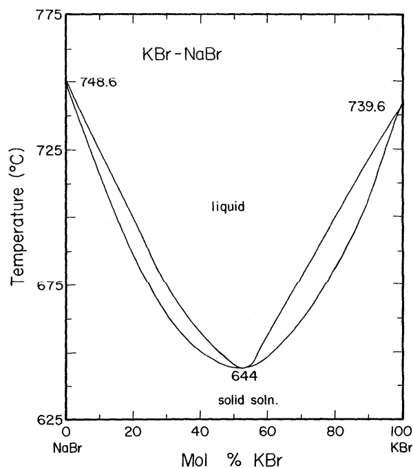
FIGURE 29. Temperature-composition phase diagram for KBr-NaBr.
