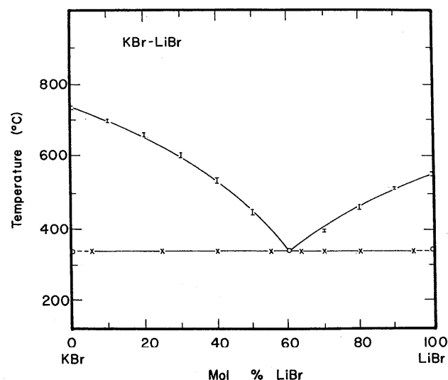
FIGURE 28. Temperature-composition phase diagram for KBr-LiBr.
