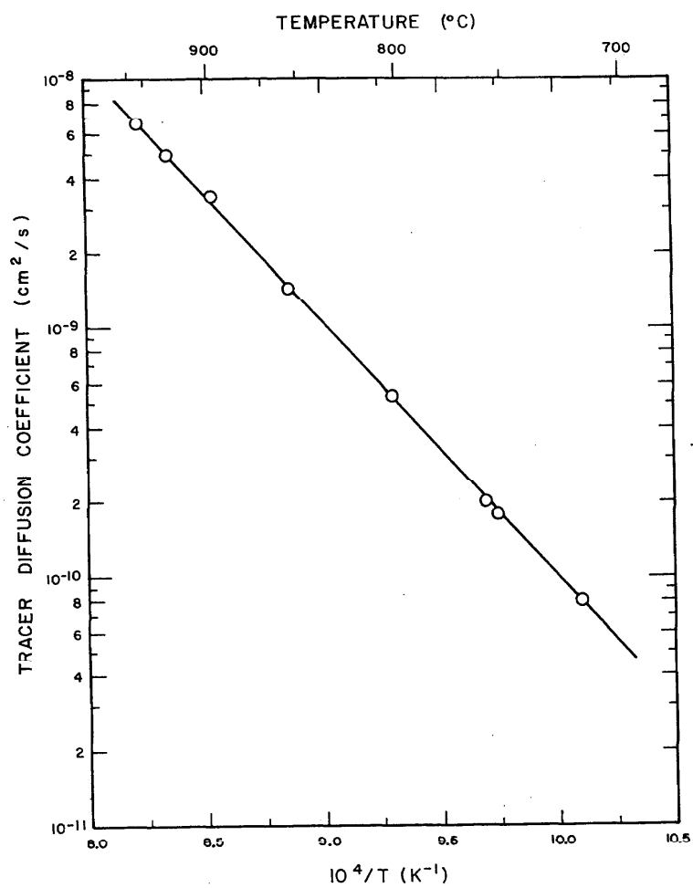
FIGURE 4. Copper tracer diffusion coefficients in silver as a function of reciprocal absolute temperature.
