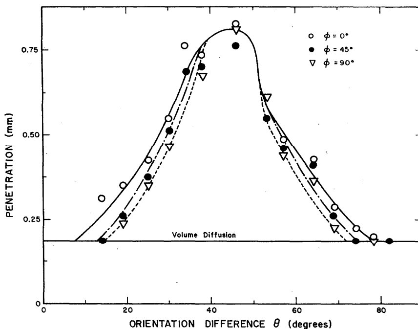
FIGURE 22. Grain boundary penetration of silver in copper as a function of orientation difference ( \theta ) measured for three different values of \phi (where \phi is the orientation of specimens with respect to the common [100] direction and the plane of the grain boundary).
