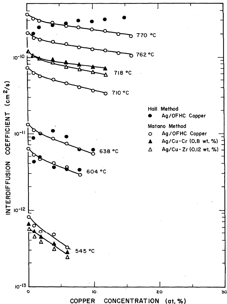
FIGURE 11. Interdiffusion coefficients as a function of composition. Pure silver was bonded to OFHC copper and copper containing chromium or zirconium.
