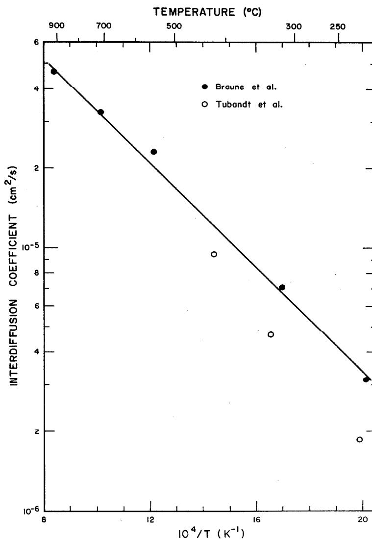
FIGURE 17. Average interdiffusion coefficients for the interdiffusion of silver in copper sulfide ( \text{Cu}_2\text{S} ) as a function of reciprocal absolute temperature.
