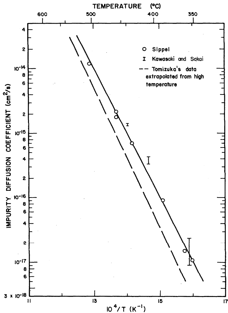
FIGURE 32. Impurity and tracer diffusion coefficients of gold in pure copper (at low temperatures, 500 to 350 °C) as a function of reciprocal absolute temperature.
