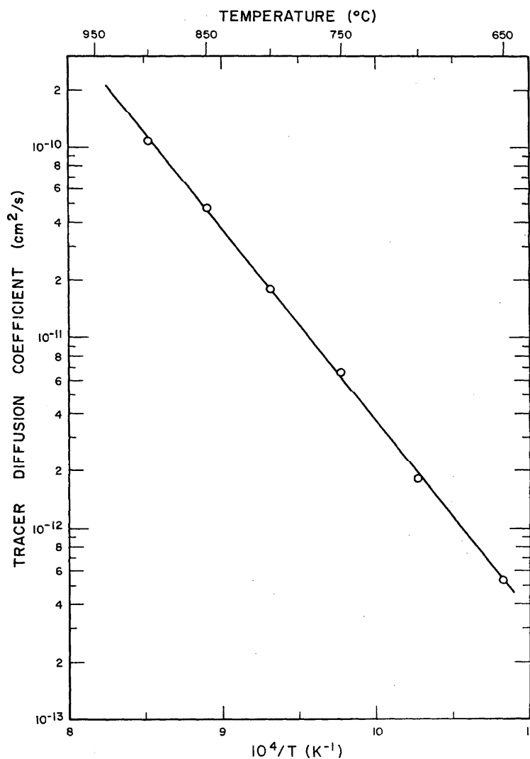
FIGURE 43. Cobalt-57 tracer diffusion coefficients in a \text{Cu}_3\text{Au} alloy as a function of reciprocal absolute temperature.
