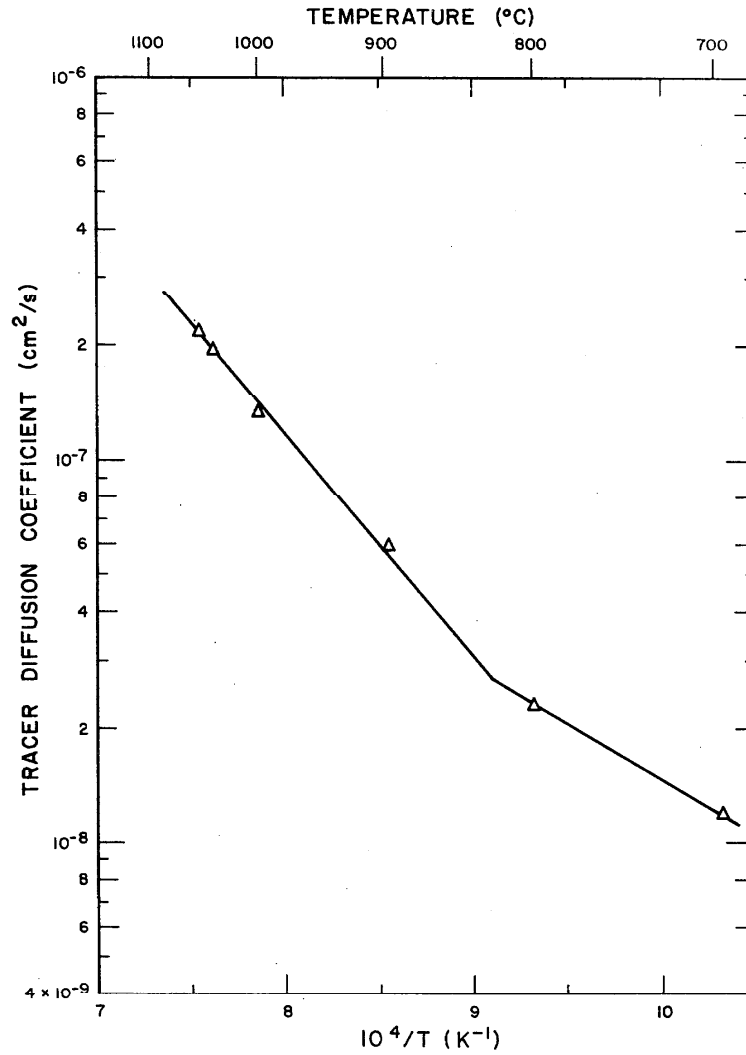
FIGURE 15. The tracer diffusion coefficient of silver-110 into polycrystalline \text{Cu}_2\text{O} as a function of reciprocal absolute temperature.
