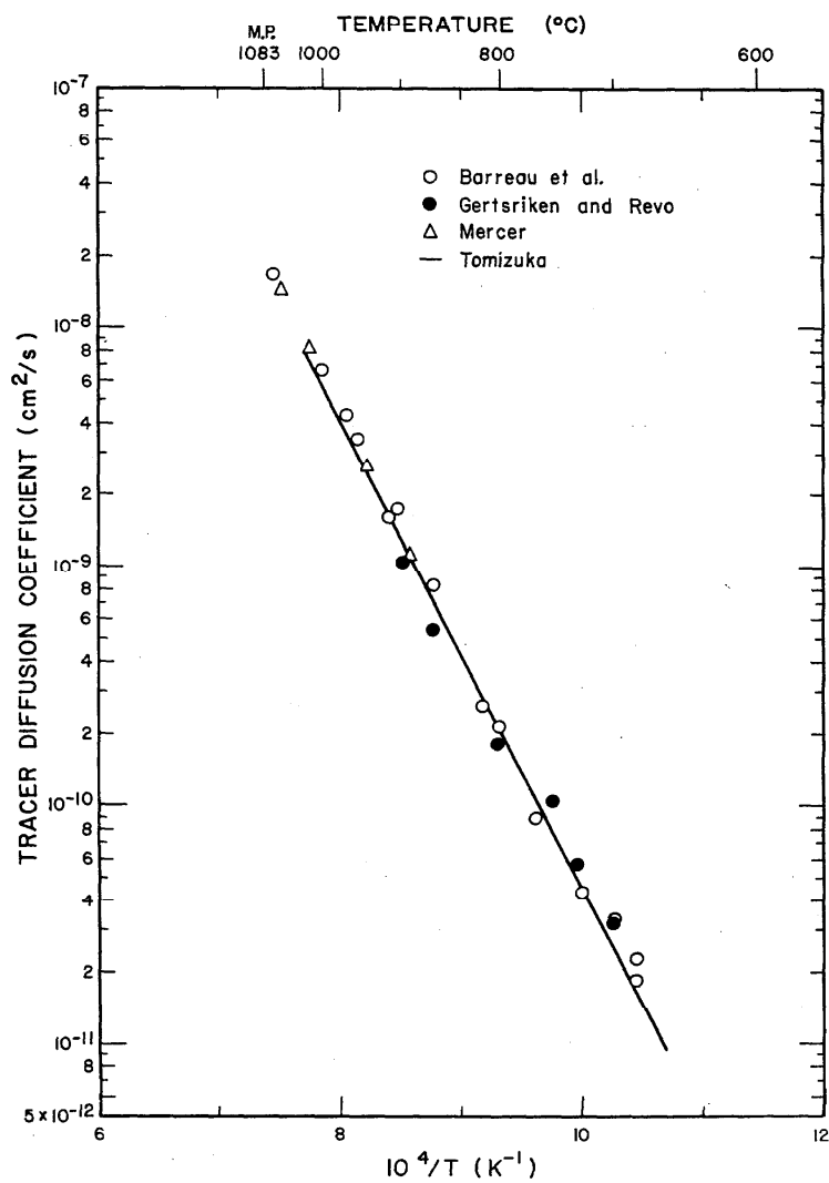
FIGURE 1. Tracer diffusion coefficients of silver in pure copper as a function of the reciprocal absolute temperature.
