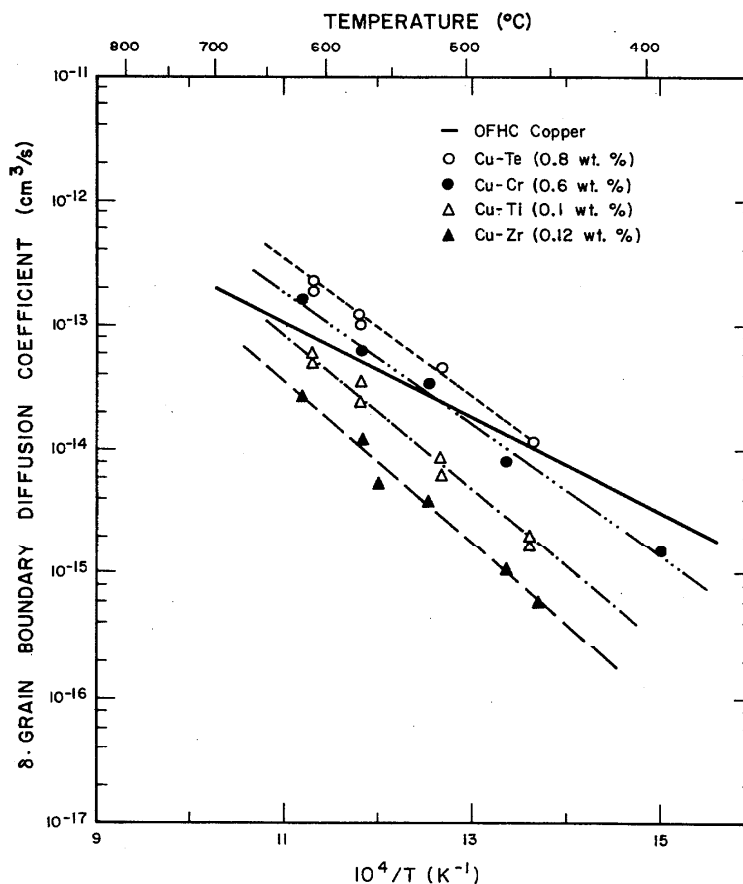
FIGURE 26. The product [\delta \cdot D_{gb}] (where \delta is the mean grain boundary thickness and D_{gb} is the grain boundary diffusion coefficient of silver) as a function of reciprocal absolute temperature for silver diffusion in the grain boundary of pure (OFHC) copper, and some dilute copper alloys of (Cu-Cr, Cu-Te, Cu-Ti, and Cu-Zr).
