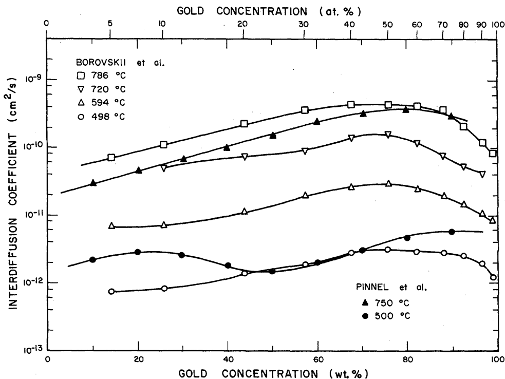
FIGURE 39. Values of the interdiffusion coefficient in the copper-gold alloy system as a function of gold concentration.
