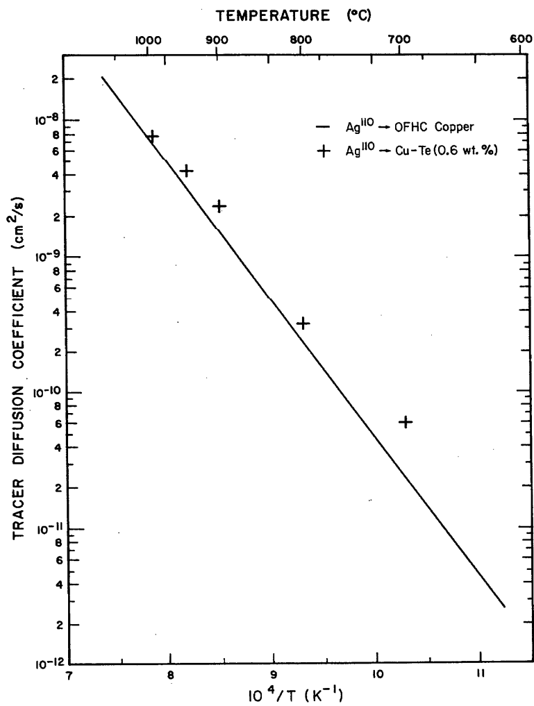
FIGURE 18. Tracer diffusion coefficients of silver-110 in copper (OFHC) and a copper-tellurium alloy (0.6 wt % Te) as a function of reciprocal absolute temperature.
