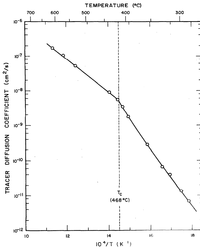
FIGURE 20. Tracer diffusion coefficients of silver-110 in ordered and disordered polycrystalline \beta -brass (47.2 at. % Zn) as a function of reciprocal absolute temperature.
