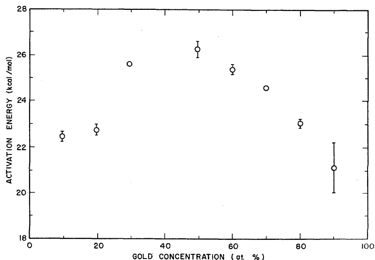
FIGURE 37. Activation energy for interdiffusion in the copper-gold alloy system as a function of gold concentration as determined by Borovskii and co-workers [246].
