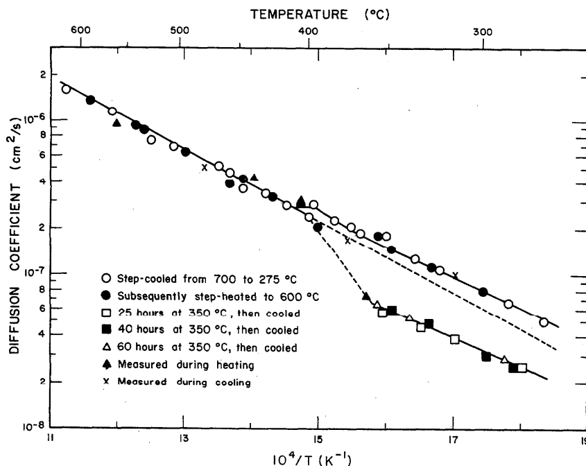
FIGURE 44. The diffusion of hydrogen through a thin alloy membrane of \text{Cu}_3\text{Au} alloy as a function of reciprocal absolute temperature.
