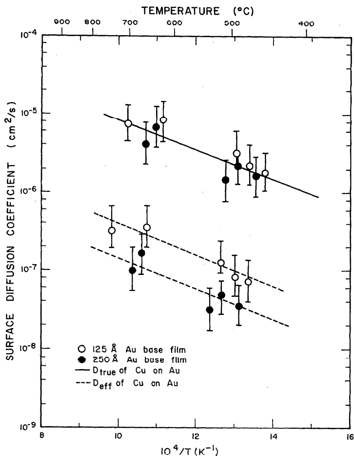
FIGURE 50. Surface diffusion coefficients of copper on gold as a function of reciprocal absolute temperature.
