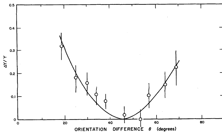
FIGURE 23. Relative grain boundary diffusion anisotropy, defined as \frac{\Delta y}{y} = \frac{y(0^\circ) - y(90^\circ)}{y(0^\circ)} where y = penetration depth, as a function of orientation difference ( \theta ).
