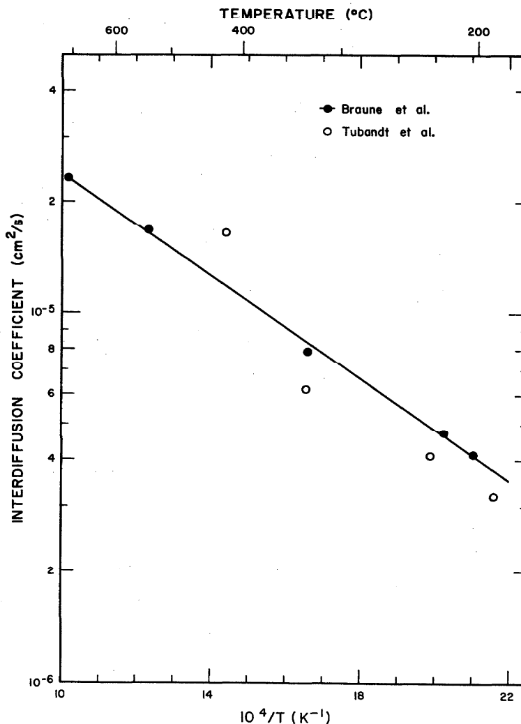
FIGURE 16. Average interdiffusion coefficients for the interdiffusion of copper in silver sulfide (Ag 2 S) as a function of reciprocal absolute temperature.
