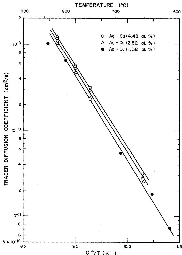
FIGURE 8. Silver tracer diffusion coefficients in several silver-copper alloys (1.38, 2.52, 4.43 at. % Cu) as a function of reciprocal absolute temperature.
