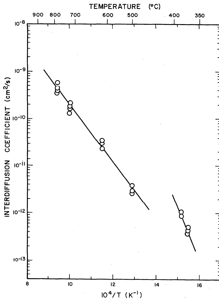
FIGURE 38. The interdiffusion coefficient, measured at the composition 50 at.% copper-50 at.% gold, as a function of reciprocal absolute temperature.
