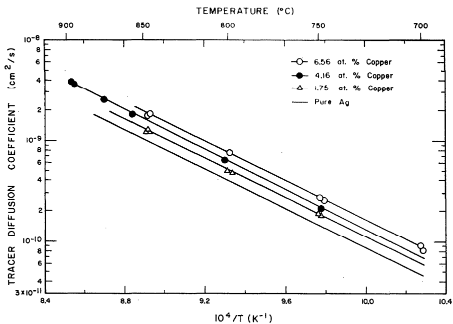
FIGURE 5. Silver tracer diffusion coefficients in several silver-copper alloys (1.75, 4.16, and 6.56 at. % Cu) as a function of reciprocal absolute temperature.
