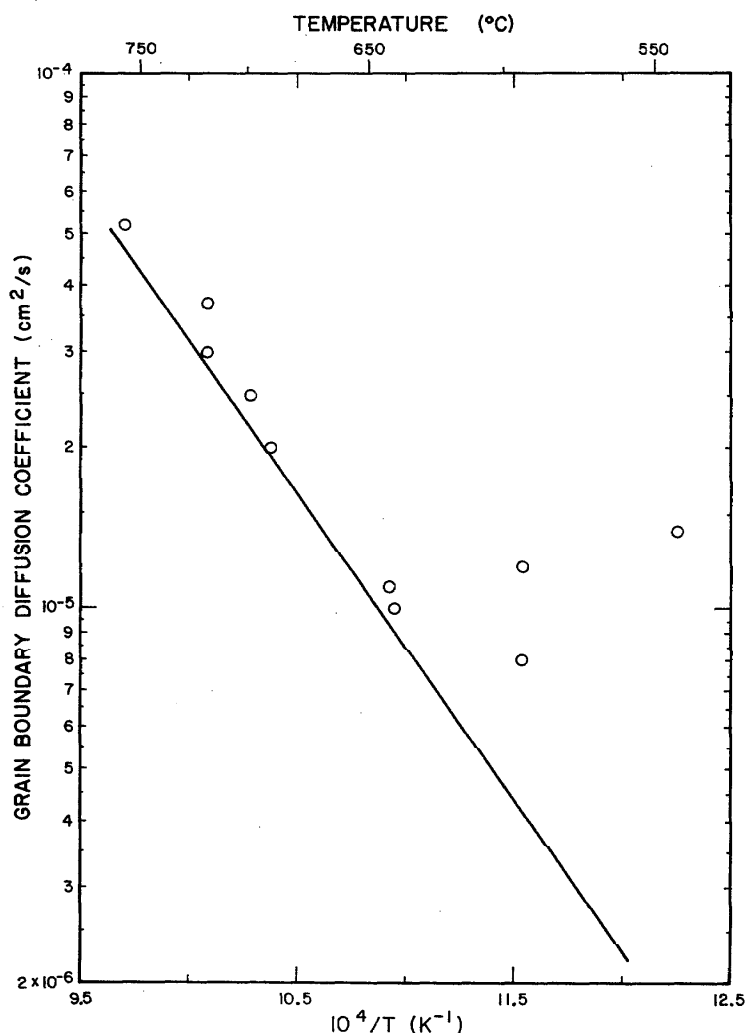
FIGURE 28. Grain boundary diffusion coefficients of silver-110 in the grain boundaries of copper bicrystals (misoriented at 45°) as a function of reciprocal absolute temperature.
