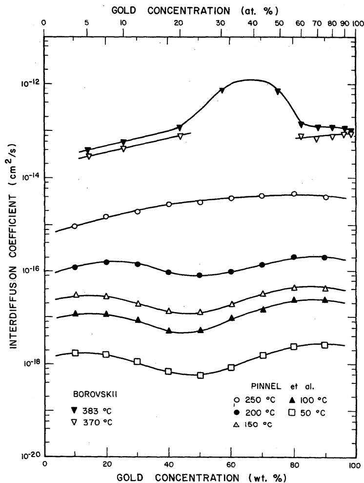
FIGURE 40. Interdiffusion coefficient in the copper-gold alloy system as a function of gold composition.
