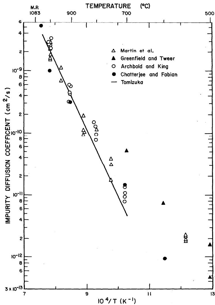
FIGURE 31. Impurity and tracer diffusion coefficients of gold in pure copper in the temperature range 1070 to 500 °C.
