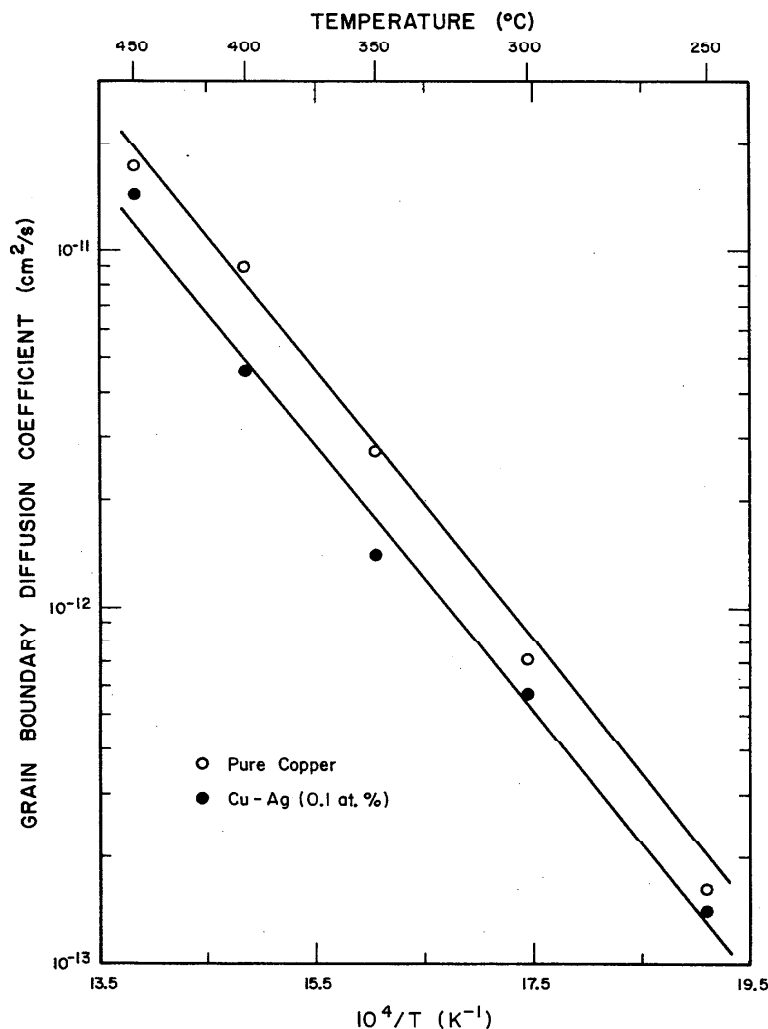
FIGURE 24. Average grain boundary diffusion coefficients of silver in pure copper and a copper-silver alloy (0.1 at. % Ag) as a function of reciprocal absolute temperature.
