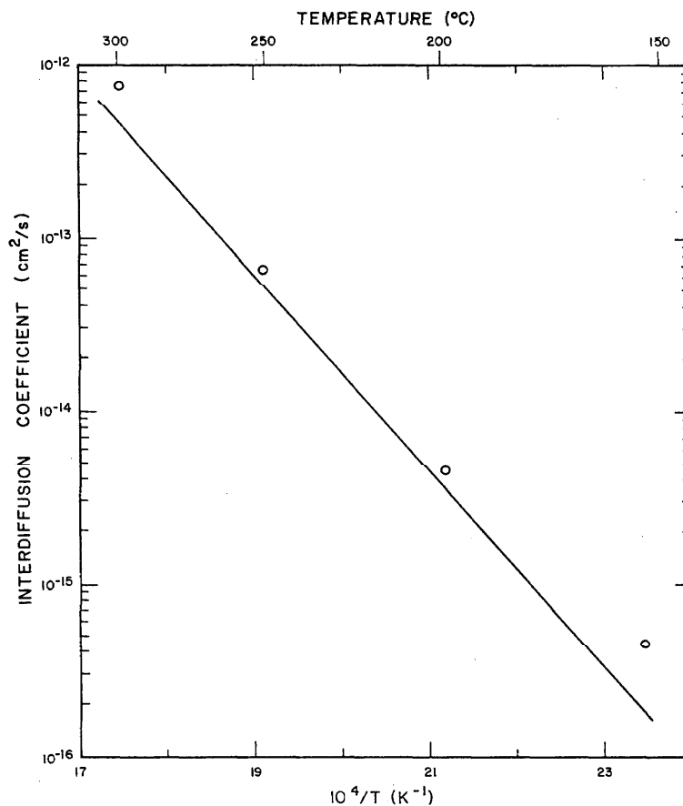
FIGURE 41. Values of an average interdiffusion coefficient (determined near the 50-50 at.% composition) as a function of reciprocal absolute temperature.
