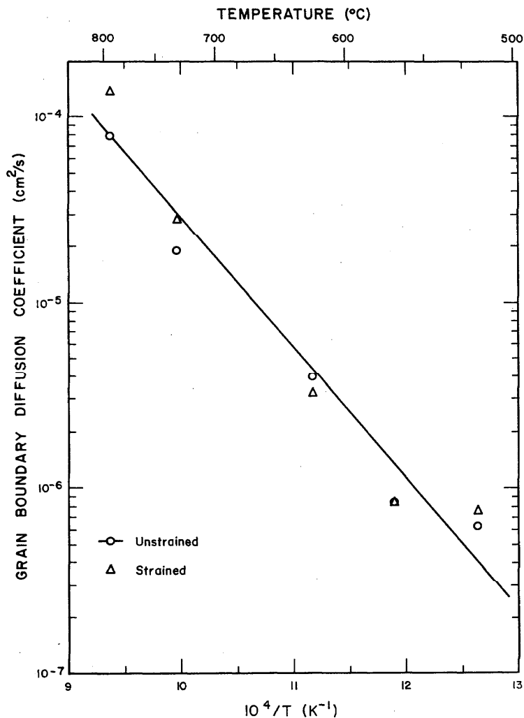
FIGURE 27. Grain boundary diffusion coefficients of silver in static and moving grain boundaries of copper as a function of reciprocal absolute temperature.
