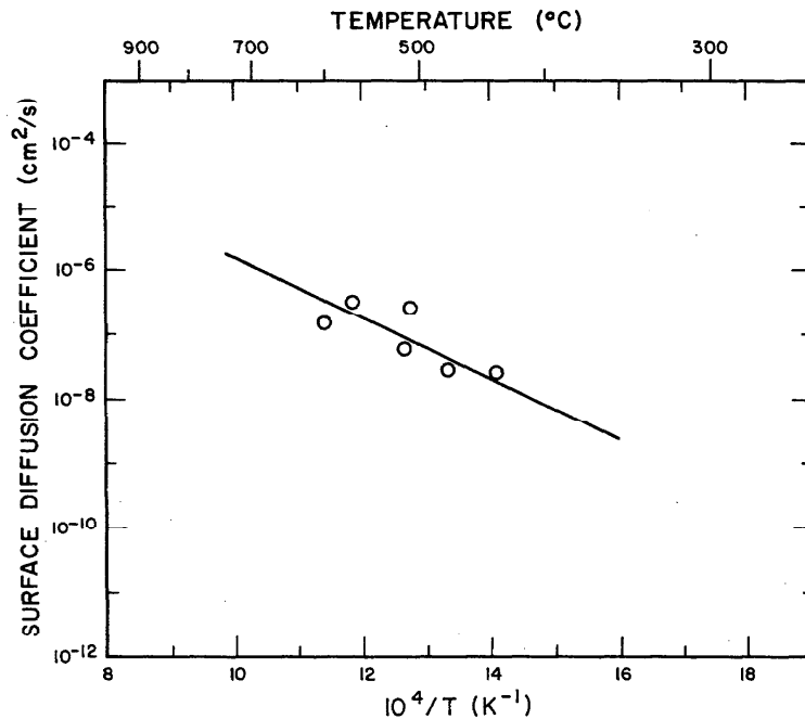
FIGURE 30. The "apparent surface diffusion coefficients" of silver on a copper surface as a function of reciprocal absolute temperature.
