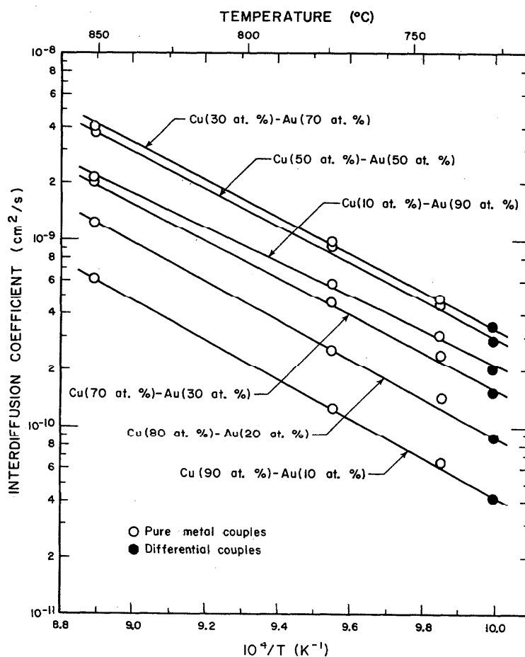
FIGURE 36. Interdiffusion coefficient as a function of reciprocal absolute temperature in the copper-gold alloy system.
