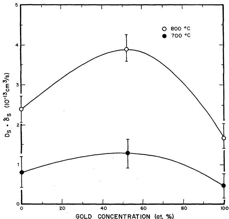
FIGURE 52. Product of an "average atom surface self-diffusion coefficient" and the depth of a subsurface layer as a function of composition.
