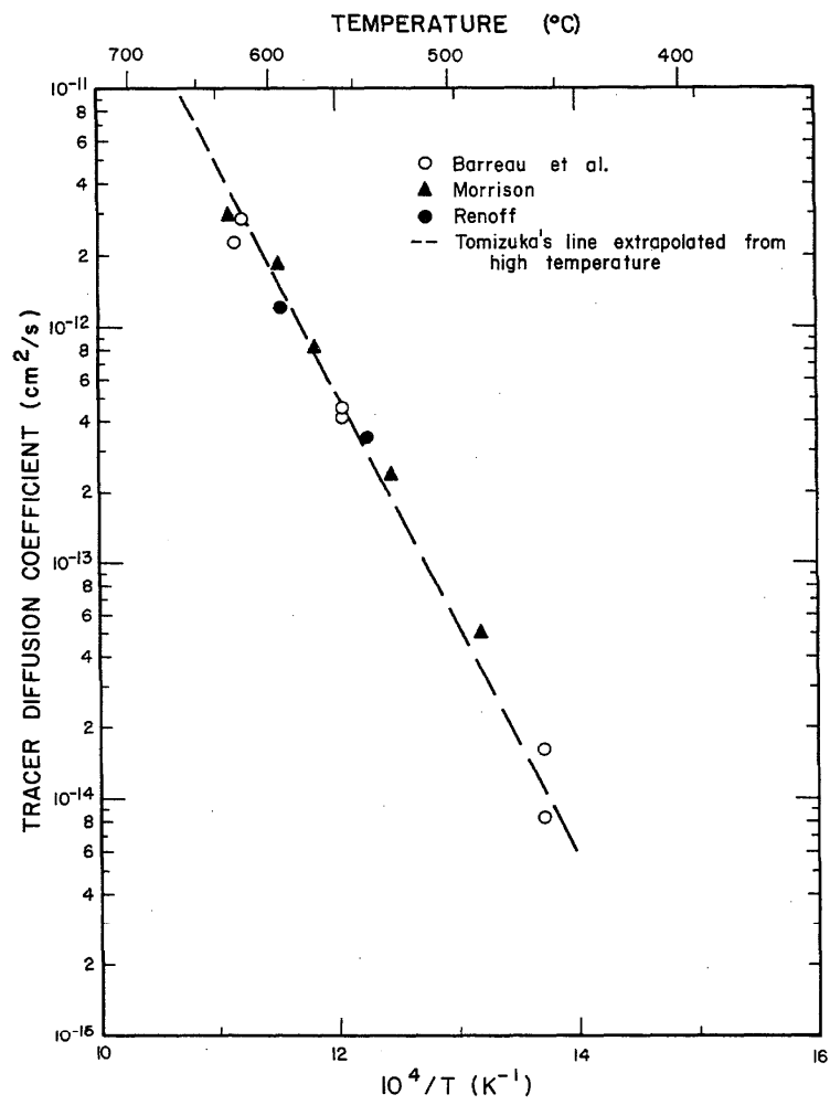
FIGURE 2. Tracer diffusion coefficients of silver in pure copper as a function of the reciprocal absolute temperature.
