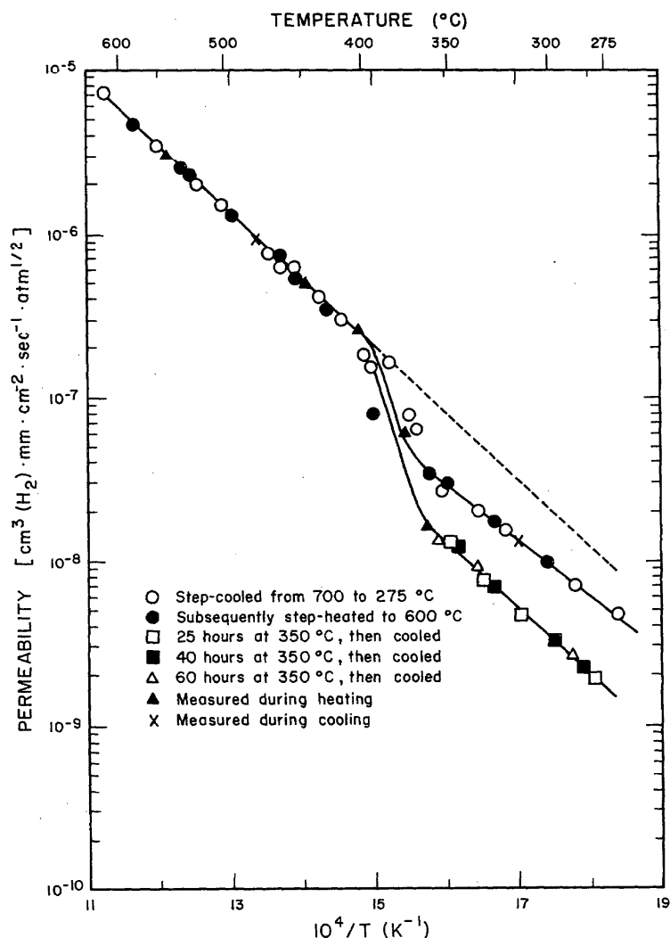
FIGURE 45. The permeability of hydrogen through a thin alloy membrane of \text{Cu}_3\text{Au} as a function of reciprocal absolute temperature.
