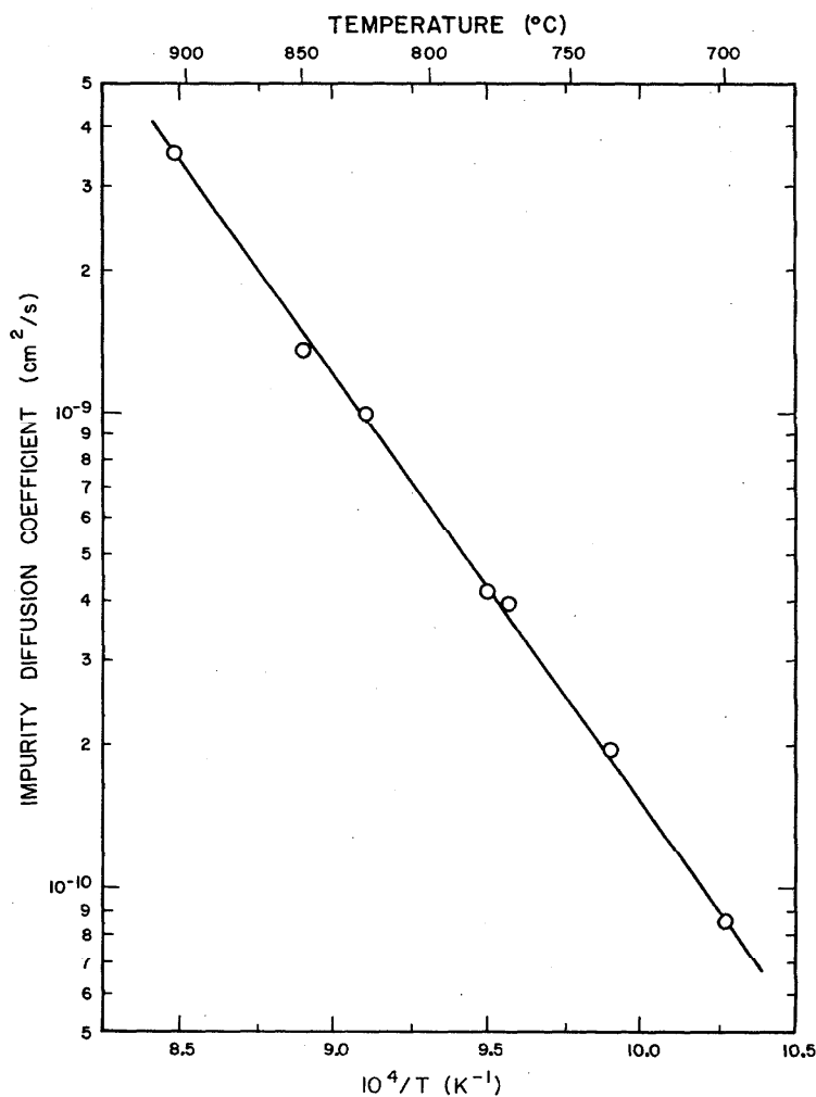
FIGURE 33. Copper impurity diffusion coefficients in gold as a function of reciprocal absolute temperature.
