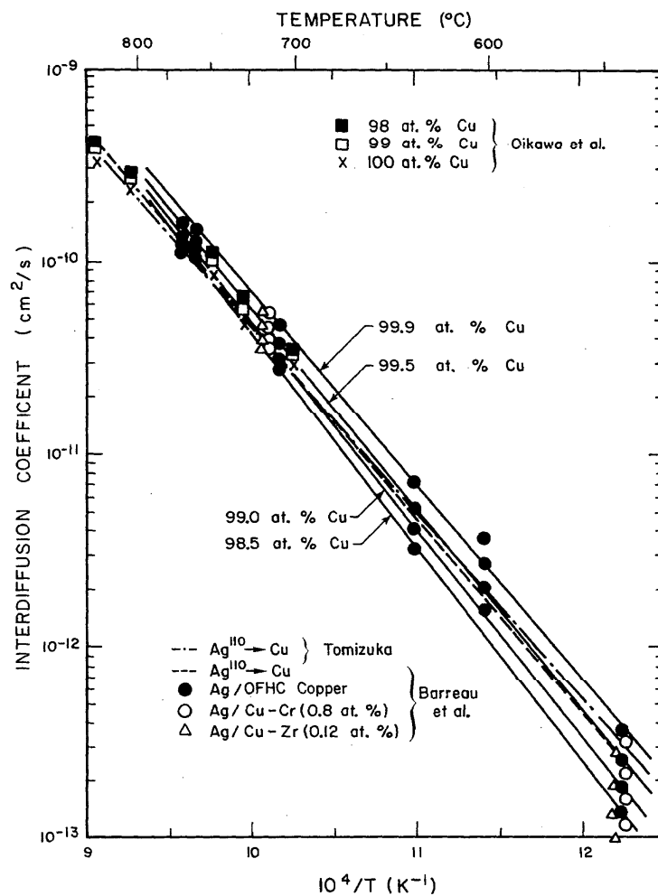
FIGURE 10. Interdiffusion coefficients as a function of reciprocal absolute temperature. The interdiffusion coefficients between silver and some copper-rich alloys (as determined by Barreau et al. [16] and copper-rich solid solutions by Oikawa et al. [58]) are compared to the silver tracer diffusion coefficient in pure copper (as determined by Barreau et al. [15, 16], and by Tomizuka [27]).
