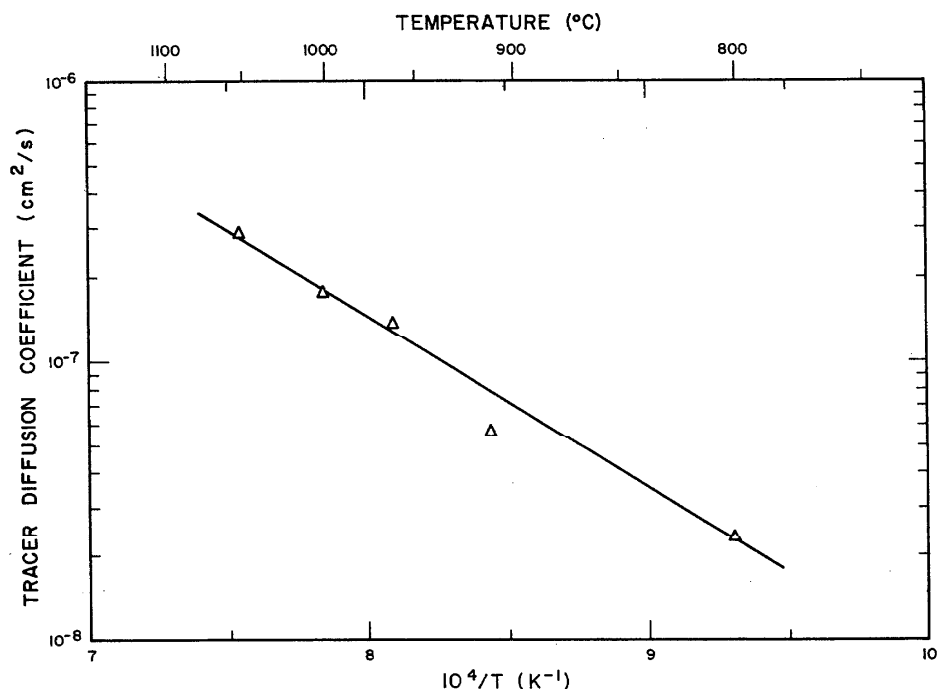
FIGURE 14. The tracer diffusion coefficients of silver-110 into single crystals of \text{Cu}_2\text{O} as a function of reciprocal absolute temperature.
