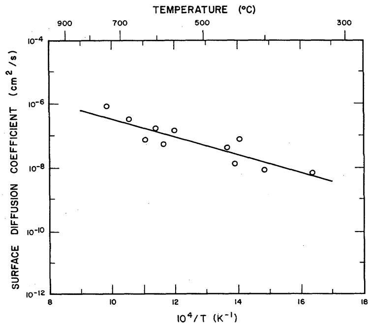
FIGURE 29. The "apparent surface diffusion coefficients" of copper on a silver surface as a function of reciprocal absolute temperature.
