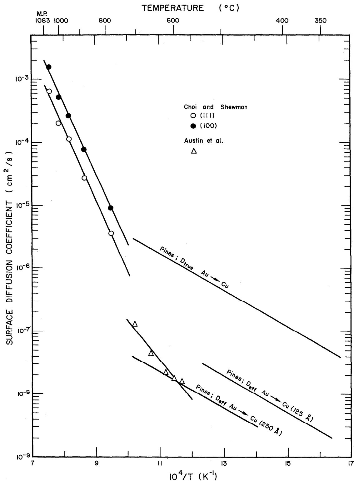
FIGURE 49. The surface diffusion coefficients of gold on copper as a function of reciprocal absolute temperature.
