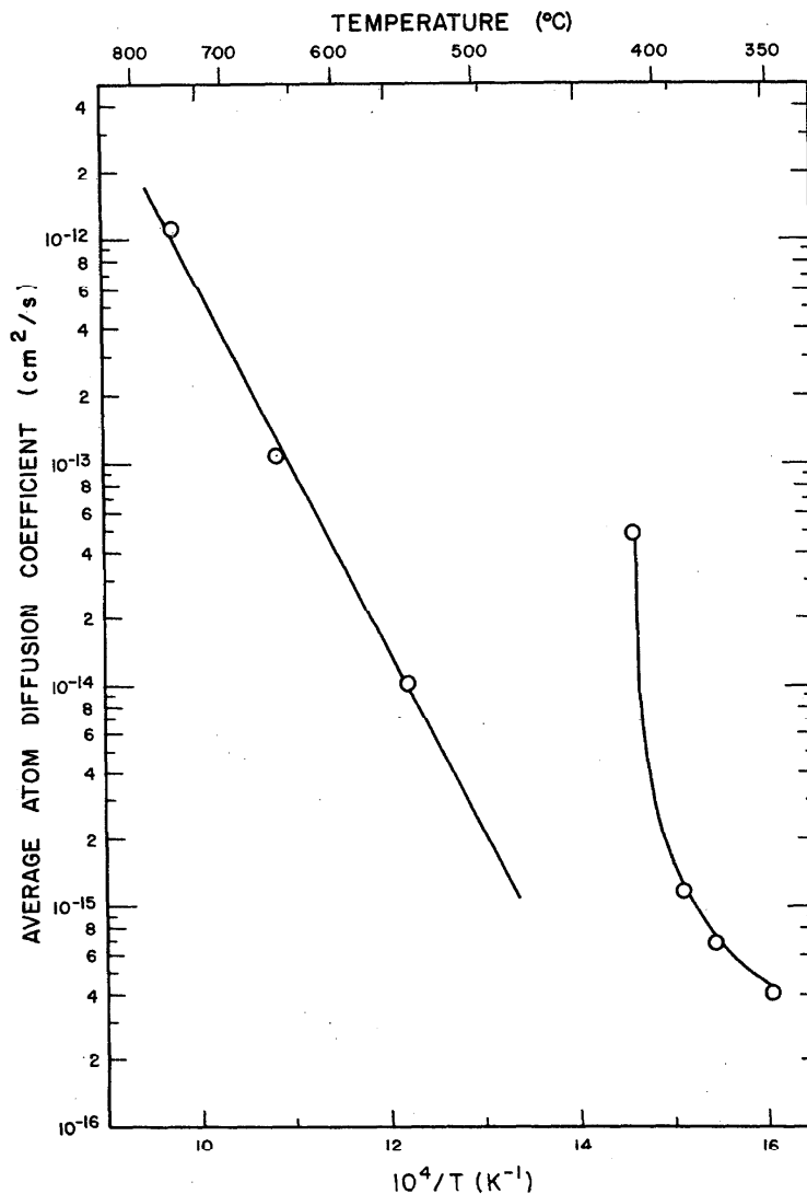
FIGURE 42. "Average atomic diffusion coefficient" as determined from neck width measurements of sintered alloy (50 at.% Au-50 at.% Cu) wires by Tournon and Kuczynski [264].
