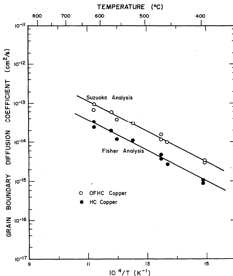
FIGURE 25. Grain boundary diffusion coefficients of silver-110 in relatively pure copper (OFHC and HC) as a function of reciprocal absolute temperature.
