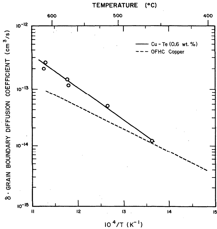
FIGURE 19. The product of the grain boundary diffusion coefficient of silver-110 in a copper-tellurium alloy times the grain boundary thickness as a function of reciprocal absolute temperature.
