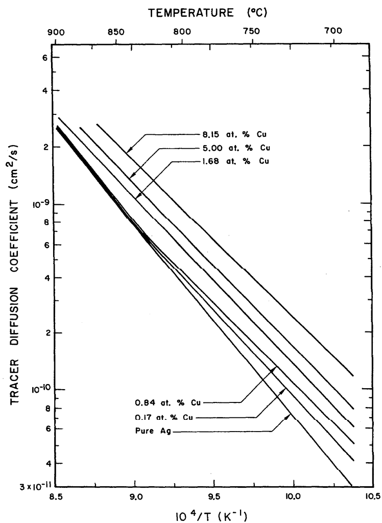
FIGURE 7. Silver tracer diffusion coefficients in silver-copper alloys (0.17, 0.84, 1.68, 5.00, 8.15 at. % Cu) as a function of reciprocal absolute temperature.
