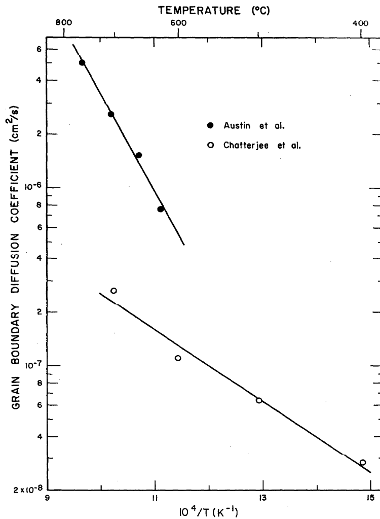
FIGURE 48. The grain boundary diffusion of gold in copper as a function of reciprocal absolute temperature.
