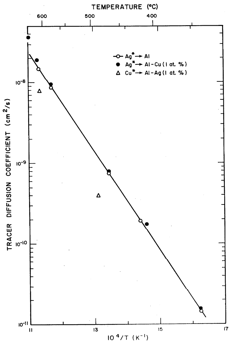
FIGURE 13. Tracer diffusion coefficients of Ag-110 and Cu-64 in aluminum and dilute aluminum alloys as a function of reciprocal absolute temperature.
