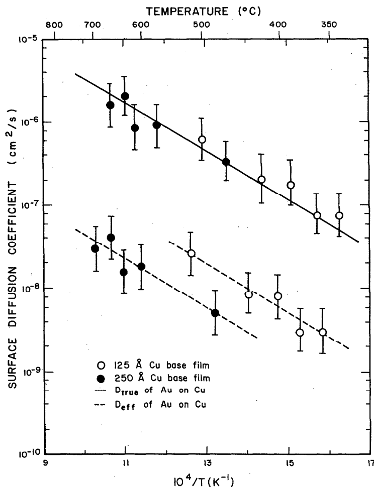
FIGURE 51. Surface diffusion coefficients of gold on copper as a function of reciprocal absolute temperature.
