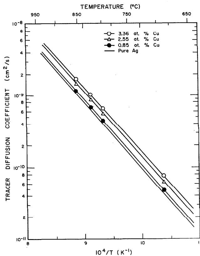
FIGURE 6. Silver tracer diffusion coefficients in several silver-copper alloys (0.85, 2.55, and 3.36 at. % Cu) as a function of reciprocal absolute temperature.
