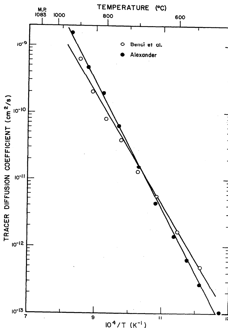
FIGURE 34. The tracer diffusion coefficient of Au-195 in the disordered alloy \text{Cu}_3\text{Au} as a function of reciprocal absolute temperature.
