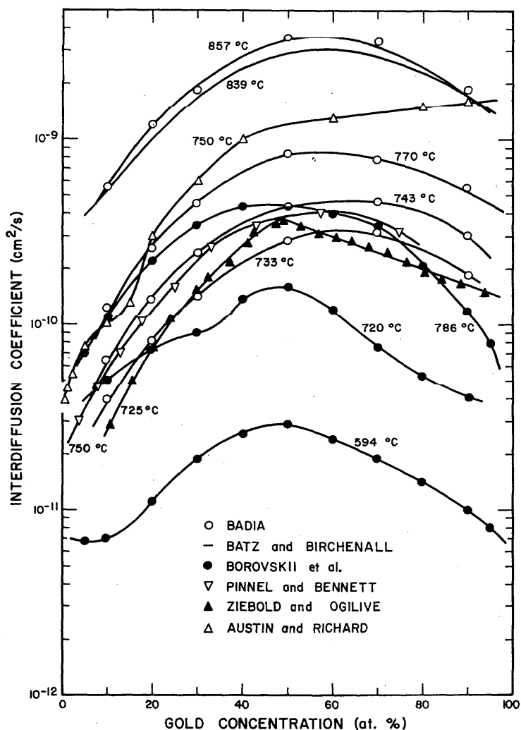
FIGURE 35. Interdiffusion coefficients in the copper-gold system as a function of composition at temperatures ranging from 600 to 860 °C.
