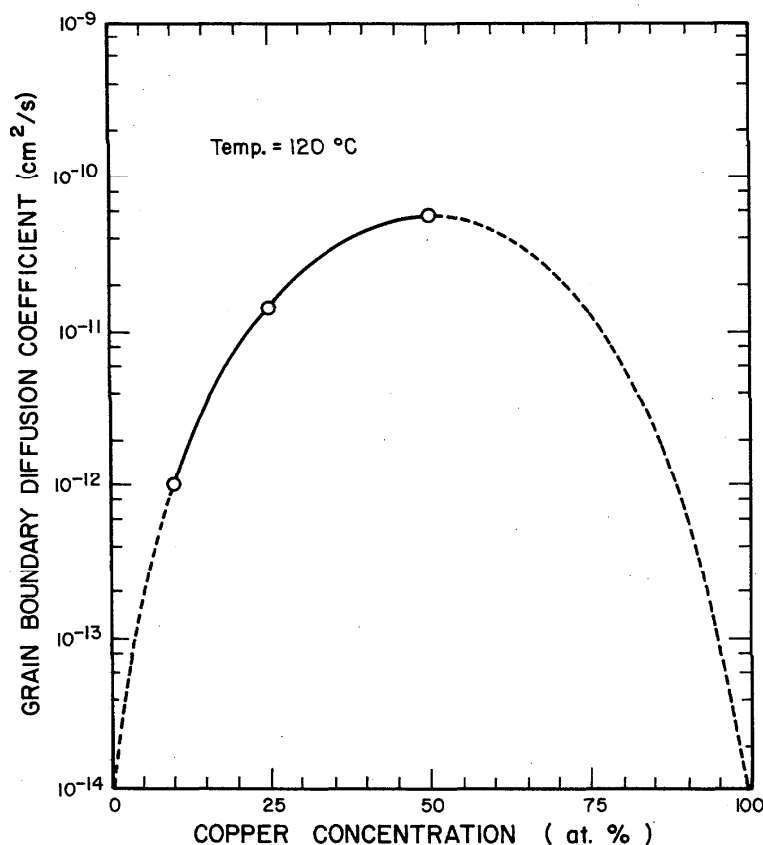
FIGURE 46. The grain boundary diffusion coefficient for mercury into copper-gold alloys as a function of composition at 120 °C.
