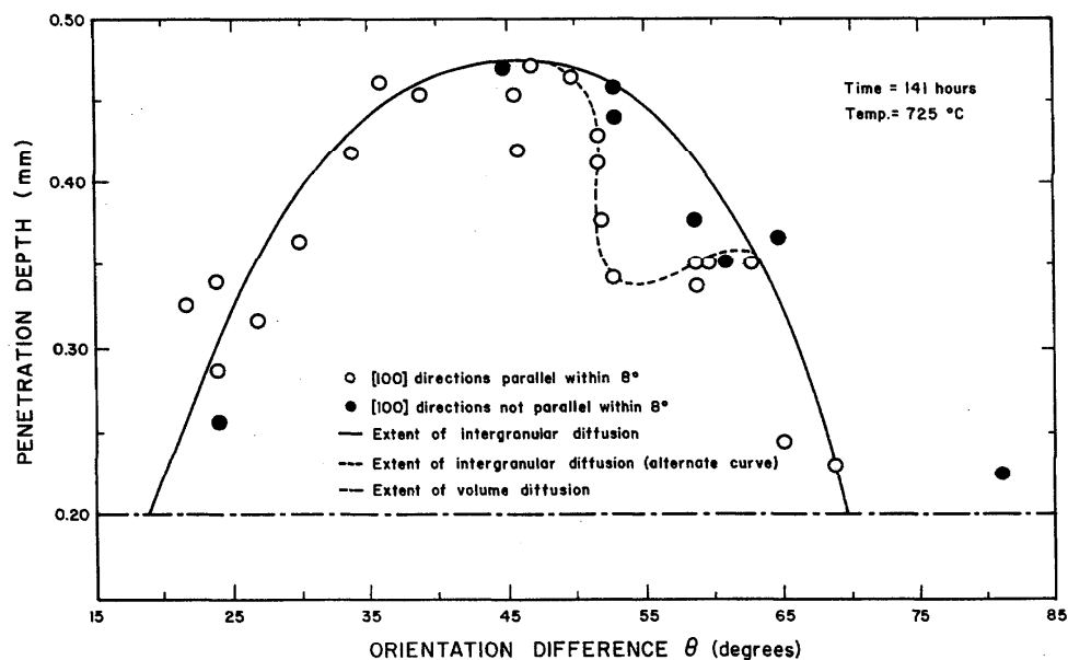
FIGURE 21. Grain boundary penetration of silver as a function of orientation difference ( \theta ) of two columnar grains of copper after 141 hours of diffusion annealing at 725 °C.
