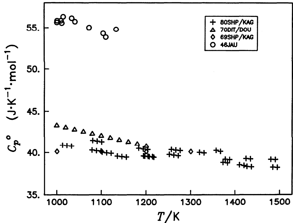
FIG. 6-5. Heat Capacity of solid and liquid Ba at 1000-1500 K.
