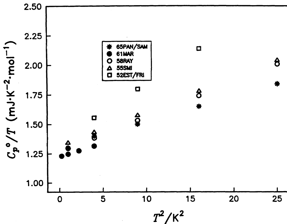
FIG. 3-1. C_p^\circ/T versus T^2 for Mg below 5 K.
