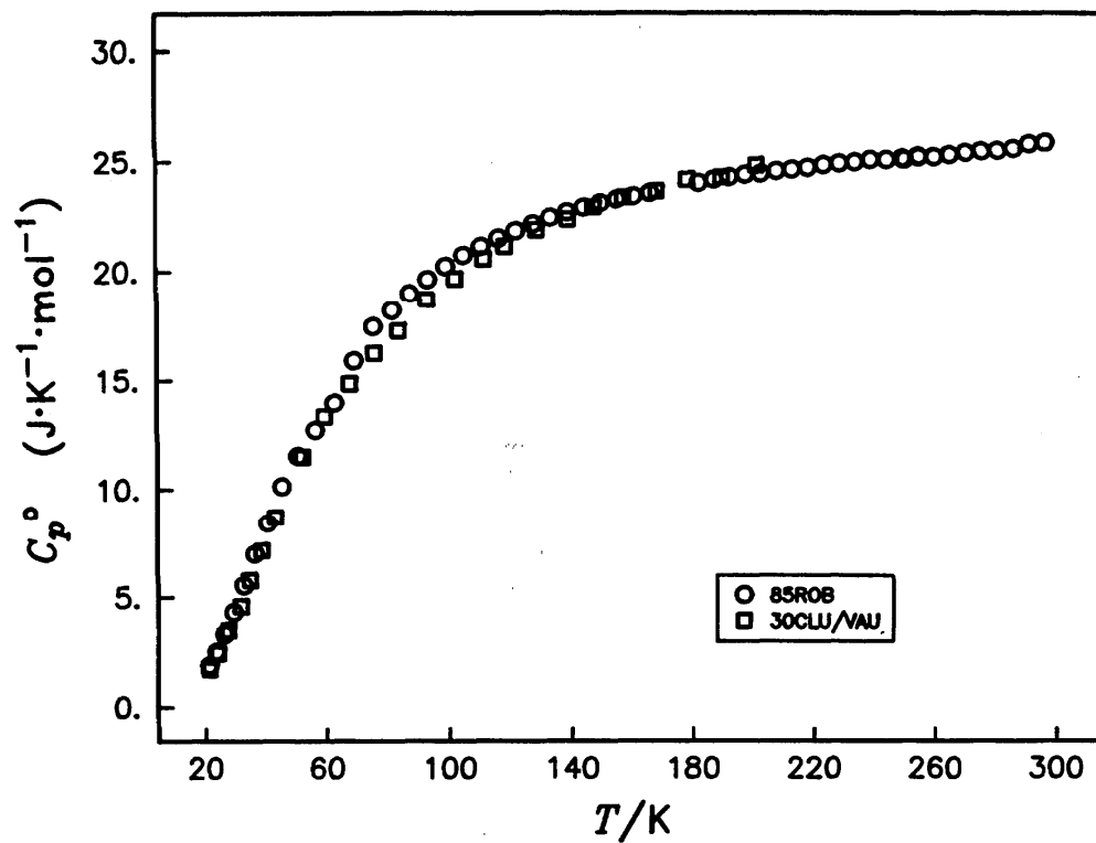
FIG. 4-3. Heat Capacity of Ca at 20–300 K.
