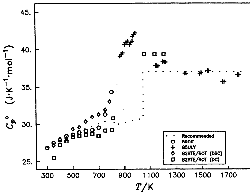
FIG. 5-4. Heat Capacity of Sr at 300-1800 K.
