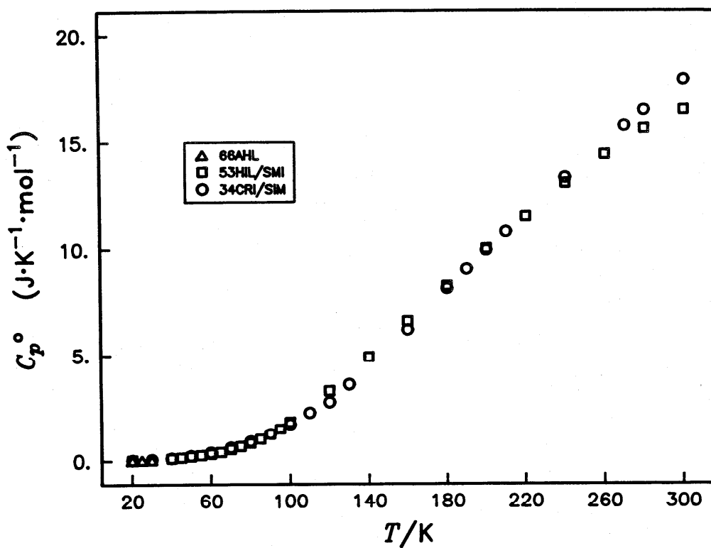
FIG. 2-3. Heat Capacity of Be at 20-300 K.
