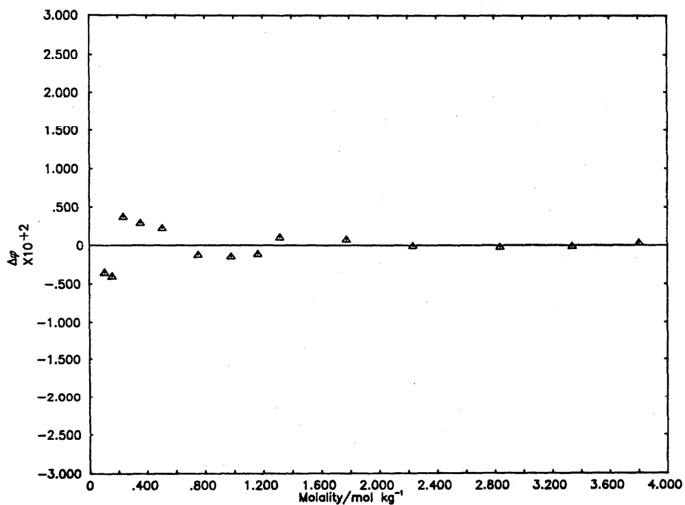
Deviation Plot for (\text{NH}_4)_2\text{B}_{10}\text{H}_{10} : \Delta\delta vs molality
