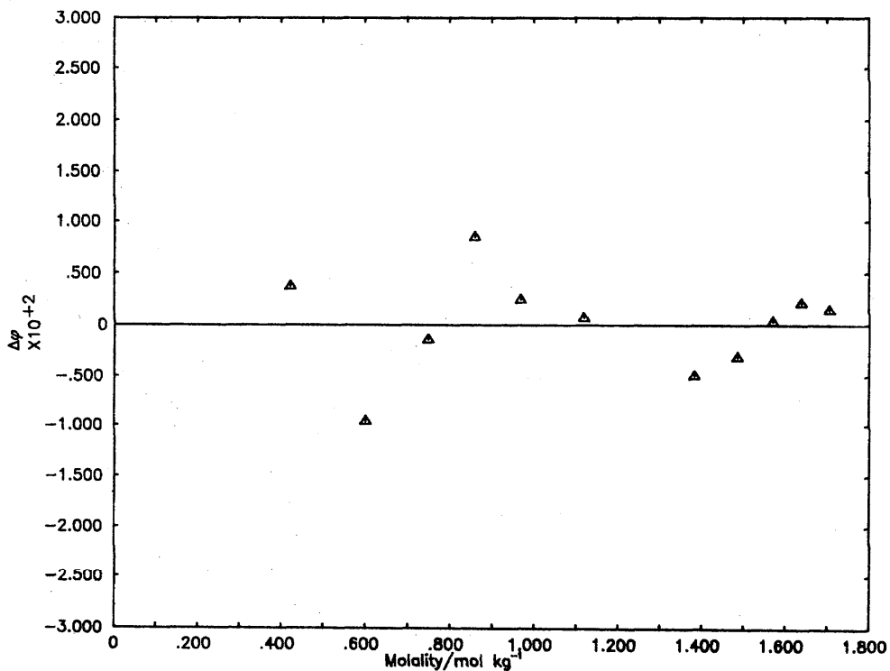
Deviation Plot for \text{Rb}_2\text{SO}_4 : \Delta\phi vs molality
