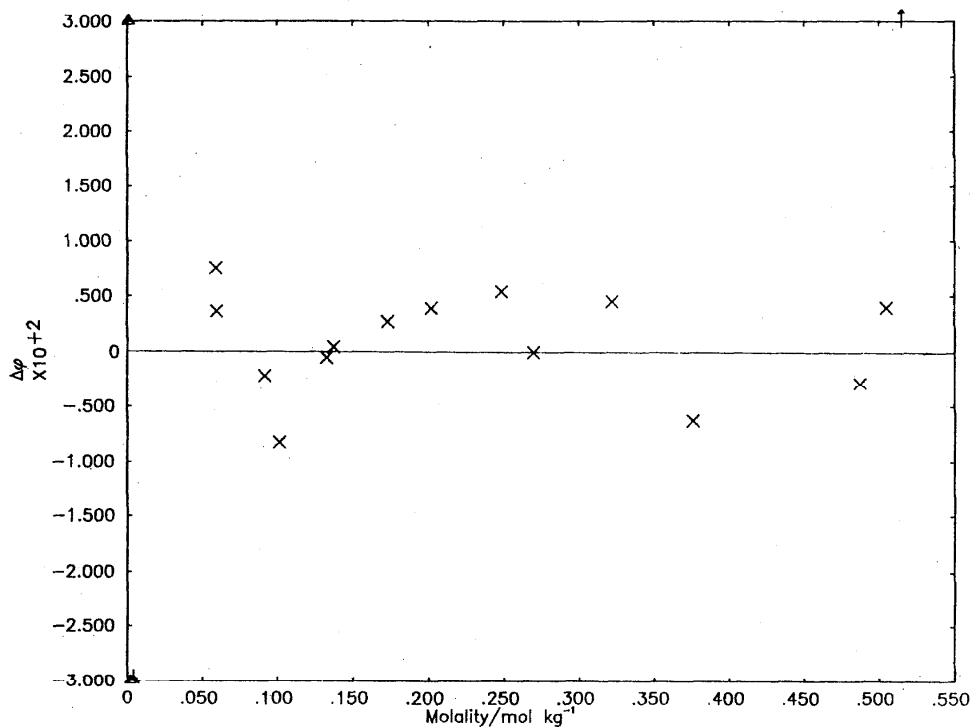
Deviation Plot for K_2Cr_2O_7 : \Delta\phi vs molality
