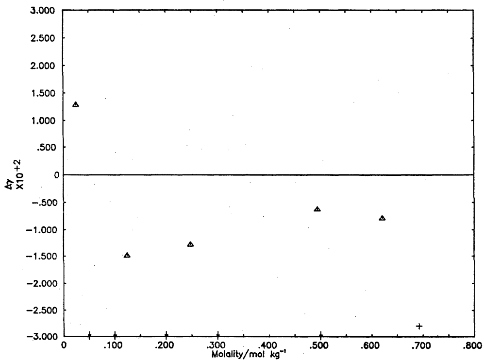
Deviation Plot for K_2SO_4 ; \Delta\gamma vs molality
