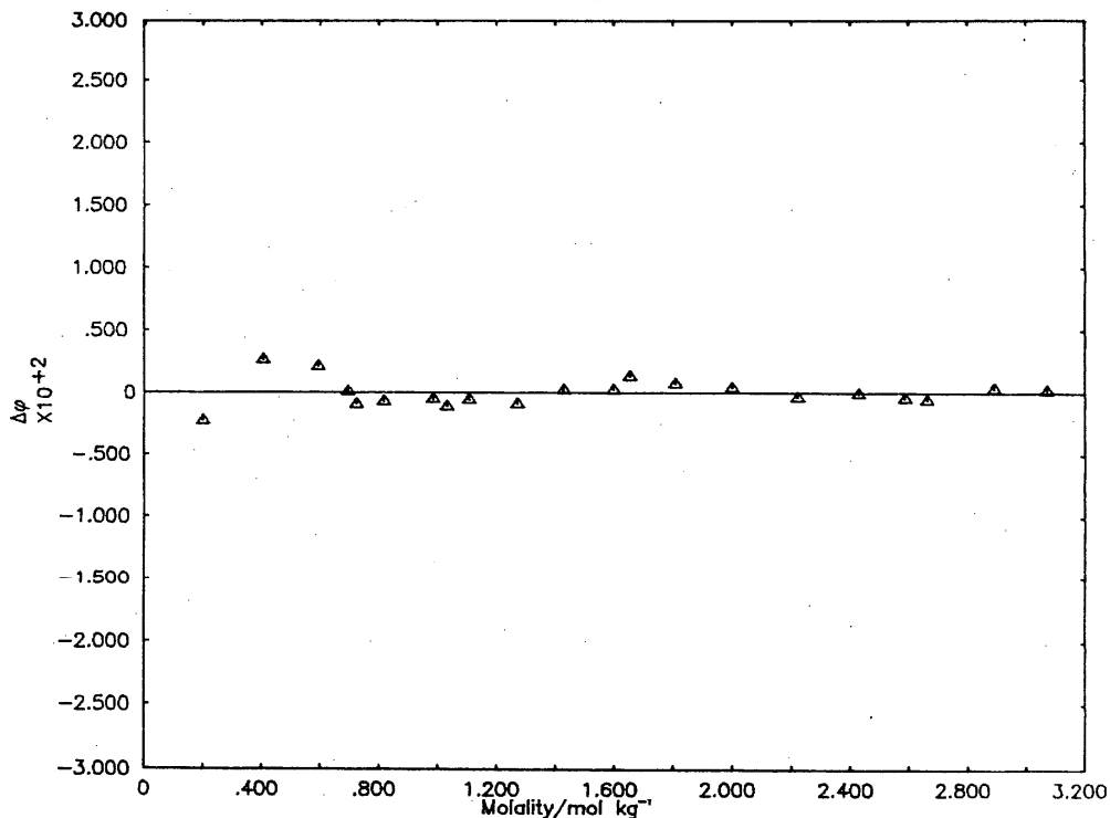
Deviation Plot for \text{K}_2\text{H}_2\text{P}_2\text{O}_7 : \Delta\phi vs molality
