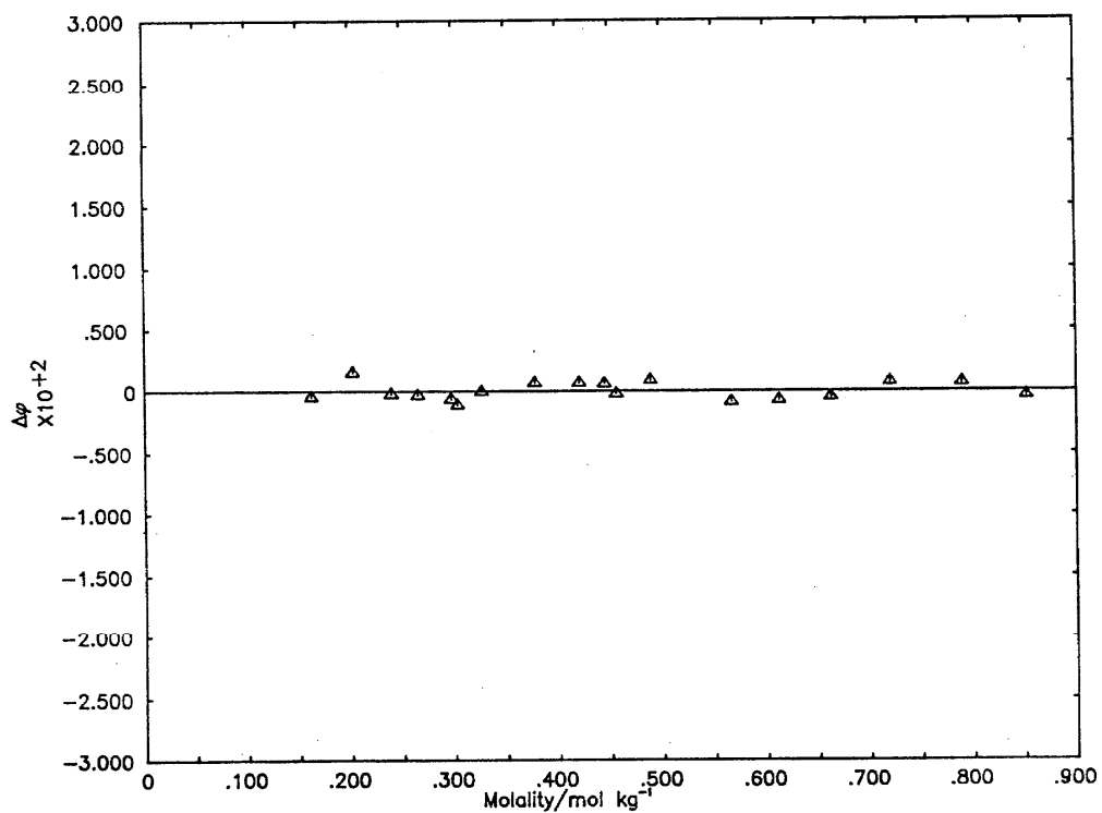
Deviation Plot for \text{Na}_2\text{S}_2\text{O}_6 : \Delta\phi vs molality
