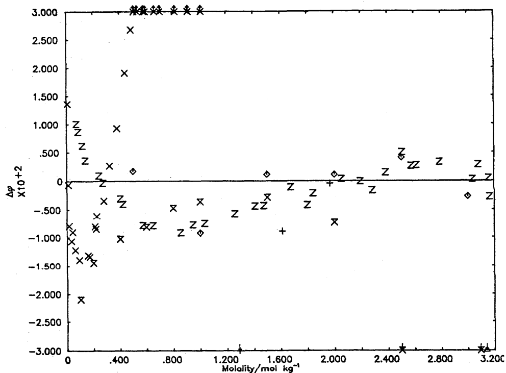
Deviation Plot for \text{Li}_2\text{SO}_4 : \Delta\phi vs molality
