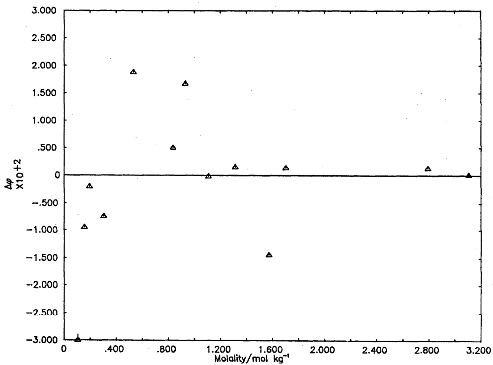
Deviation Plot for (\text{NH}_4)_2\text{HPO}_4 : \Delta\phi vs molality
