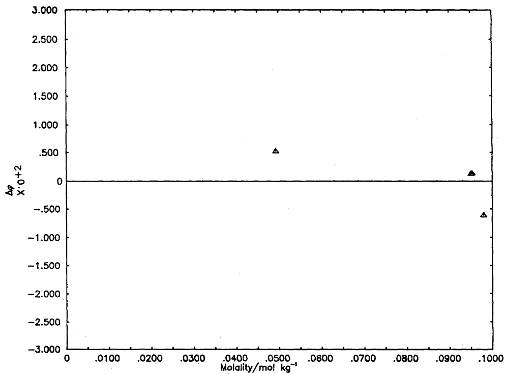
Deviation Plot for Na 2 S 2 O 8 : \Delta p vs molality
