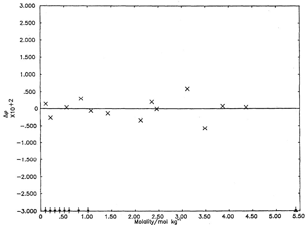
Deviation Plot for \text{Na}_2\text{CrO}_4 : \Delta\phi vs molality
