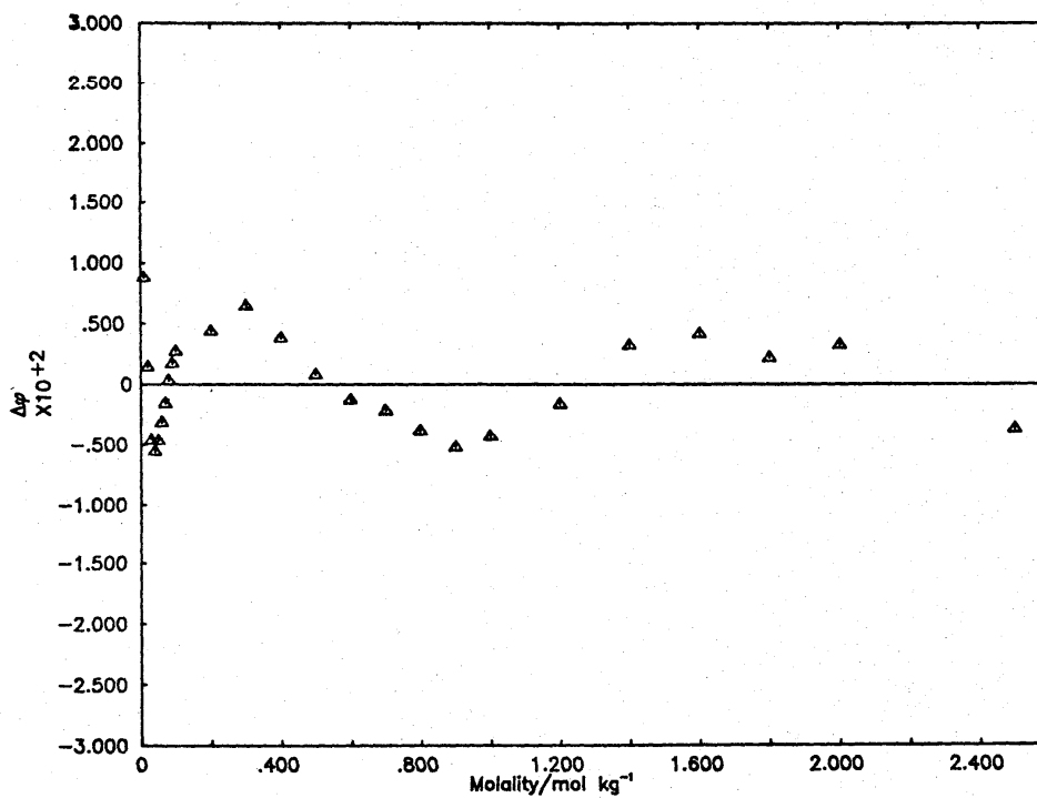
Deviation Plot for \text{Li}_2\text{C}_6\text{H}_4\text{S}_2\text{O}_6 : \Delta\delta vs molality
