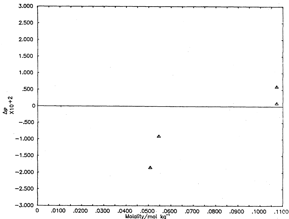
Deviation Plot for Cs 2 S 2 O 8 : Δφ vs molality
