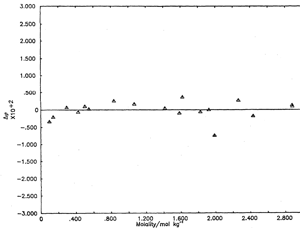
Deviations Plot for sodium maleate: \Delta\phi vs molality
