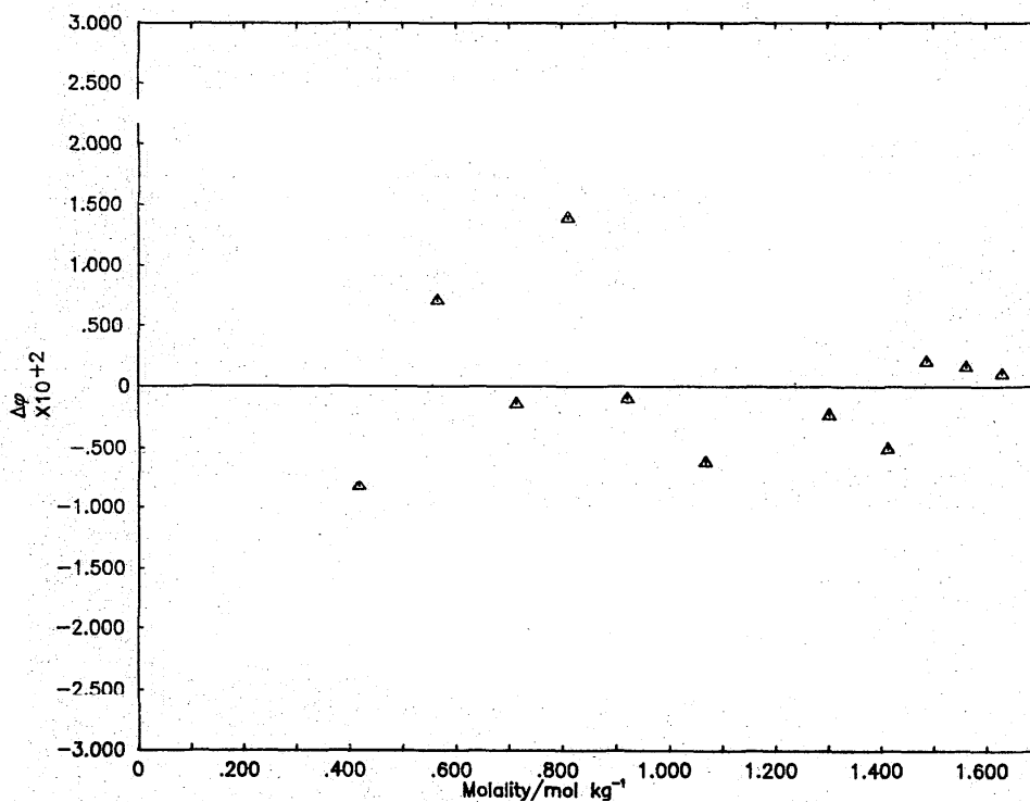
Deviaton Plot for Cs 2 SO 4 : \Delta\phi vs molality
