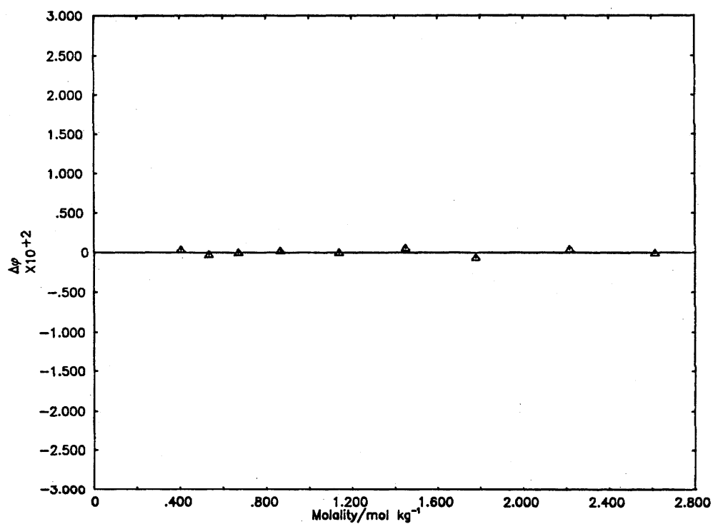
Deviation Plot for (\text{CH}_3\text{H}_6)_2\text{CO}_3 : \Delta\phi vs molality
