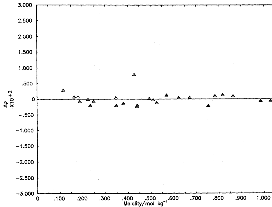
Deviation Plot for \text{Na}_2\text{HAsO}_4 : \Delta\phi vs molality
