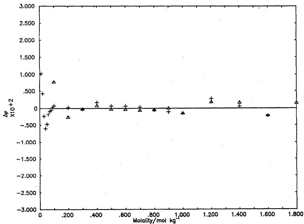
Deviation Plot for \text{C}_6\text{H}_6\text{S}_2\text{O}_6 : \Delta\phi vs molality
