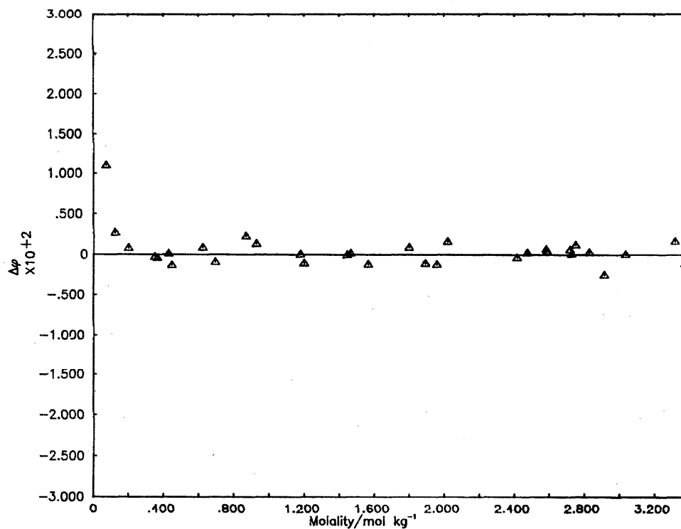
Deviation Plot for \text{K}_2\text{CrO}_4 : \Delta\phi vs molality
