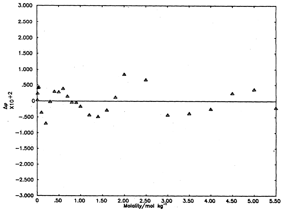
Deviation Plot for C_2H_6S_2O_6 : \Delta p vs molality
