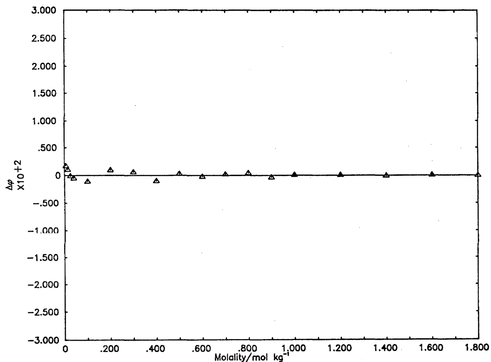
Deviation Plot for \text{Na}_2\text{C}_2\text{H}_4\text{S}_2\text{O}_6 : \Delta\phi vs molality
