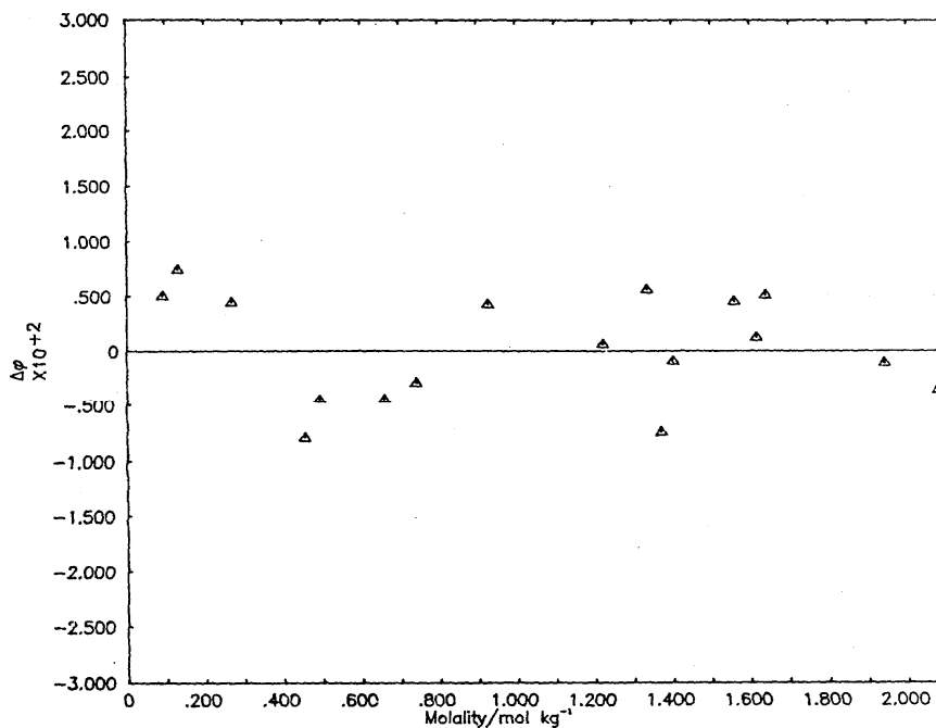
Deviation Plot for sodium fumarate: \Delta\delta vs molality
