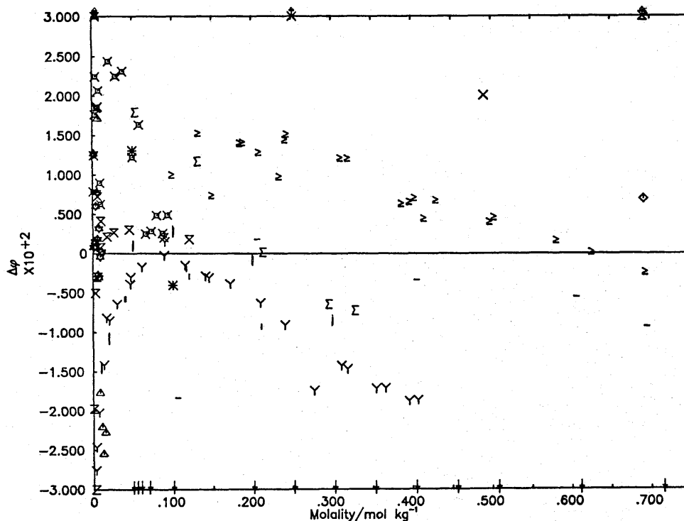
Deviation Plot for K_2SO_4 : \Delta\theta vs molality
