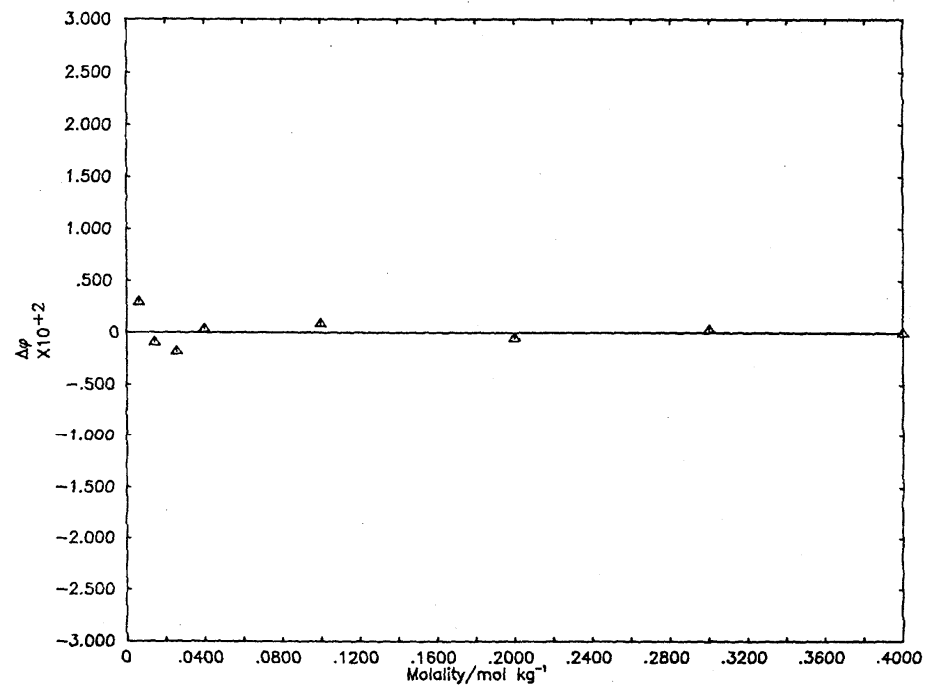
Deviation Plot for \text{Na}_2\text{C}_{14}\text{H}_{10}\text{S}_2\text{O}_8 : \Delta\phi vs molality
