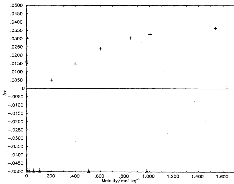
Deviation Plot for Na 2 CO 3 : Δγ vs molality
