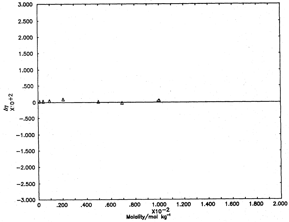
Deviation Plot for \text{Cs}_2\text{SO}_4 : \Delta\gamma vs molality
