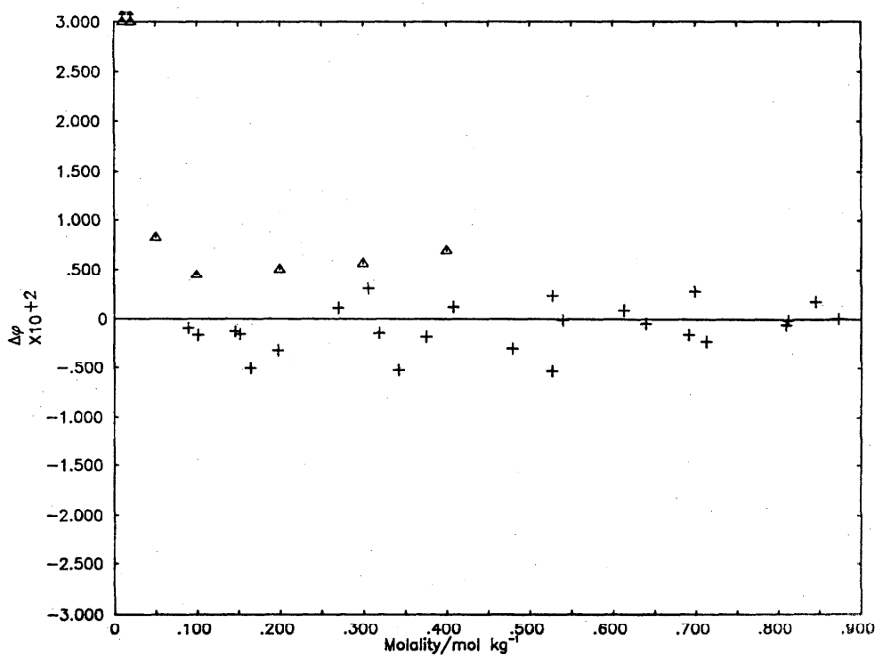
Deviation Plot for K_2HPO_4 : \Delta\phi vs molality
