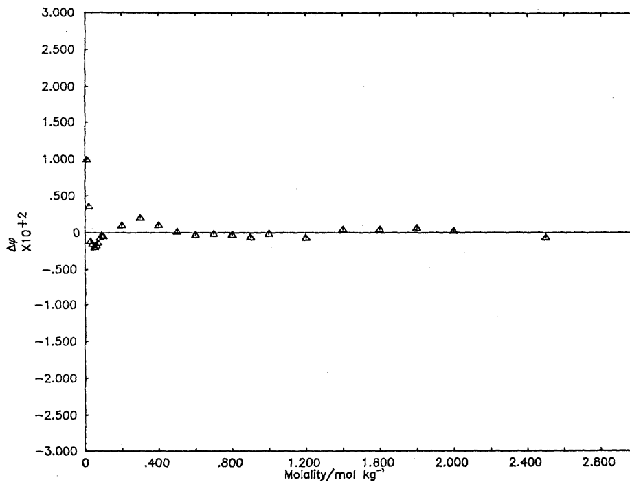
Deviation Plot for \text{Na}_2\text{C}_6\text{H}_4\text{S}_2\text{O}_6 : \Delta\phi vs molality
