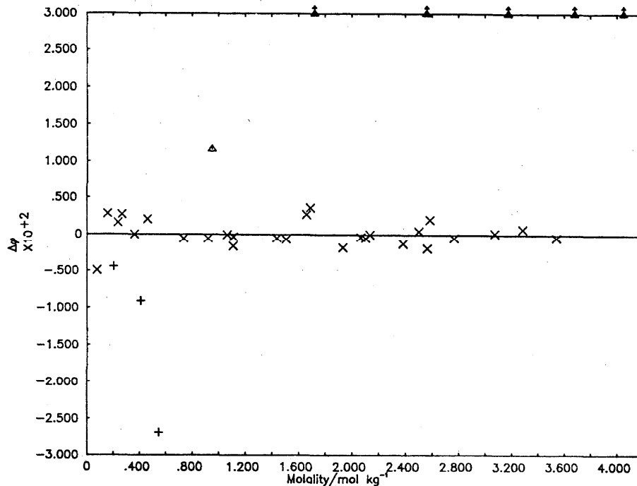
Deviation Plot for Na 2 S 2 O 3 : \Delta\phi vs molality
