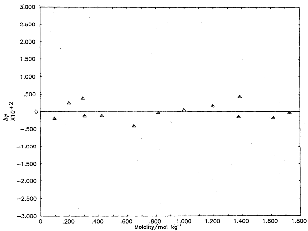
Deviation Plot for \text{Na}_2\text{B}_{12}\text{H}_{12} : \Delta\phi vs molality
