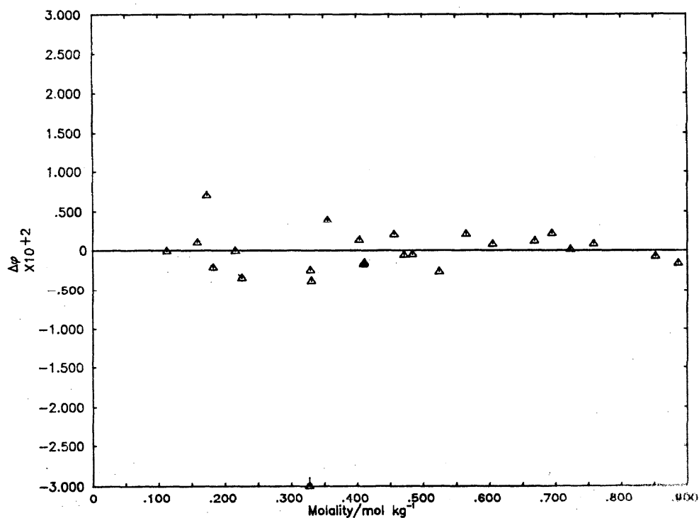
Deviation Plot for \text{K}_2\text{HAsO}_4 : \Delta\phi vs molality
