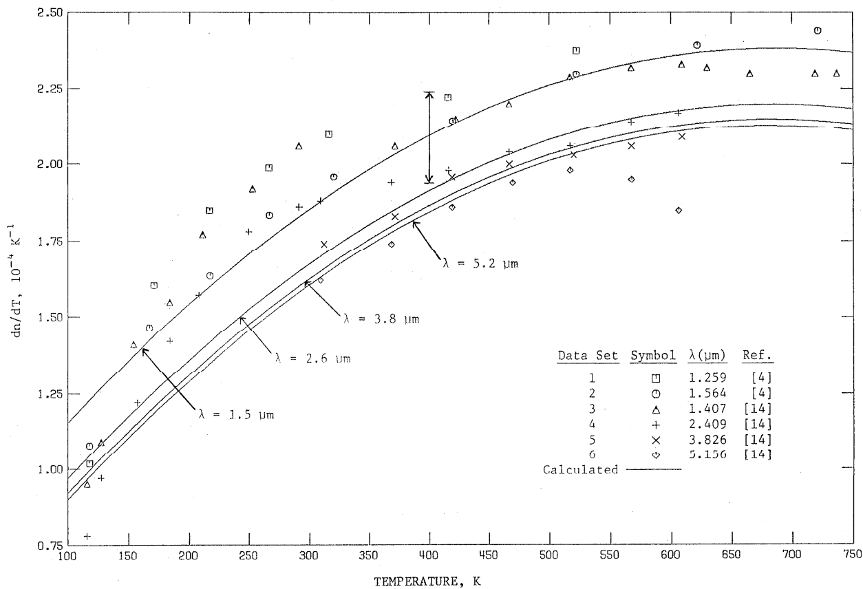
FIGURE 5. AVAILABLE EXPERIMENTAL dn/dT OF SILICON (Temperature Dependence)
