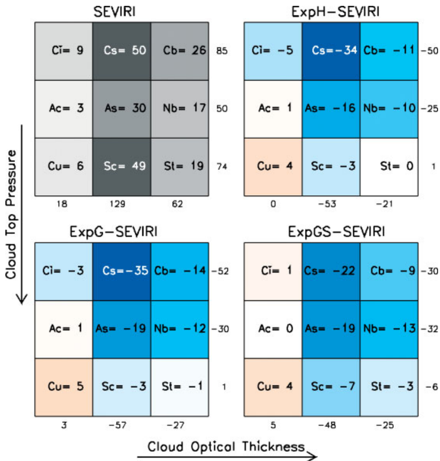
Figure 7. As in Figure 4, but for the convective composite.
