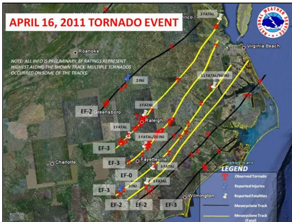
Figure 2: April 16, 2011, tornado tracks with associated EF Scale rating and location of injuries and fatalities, where available
