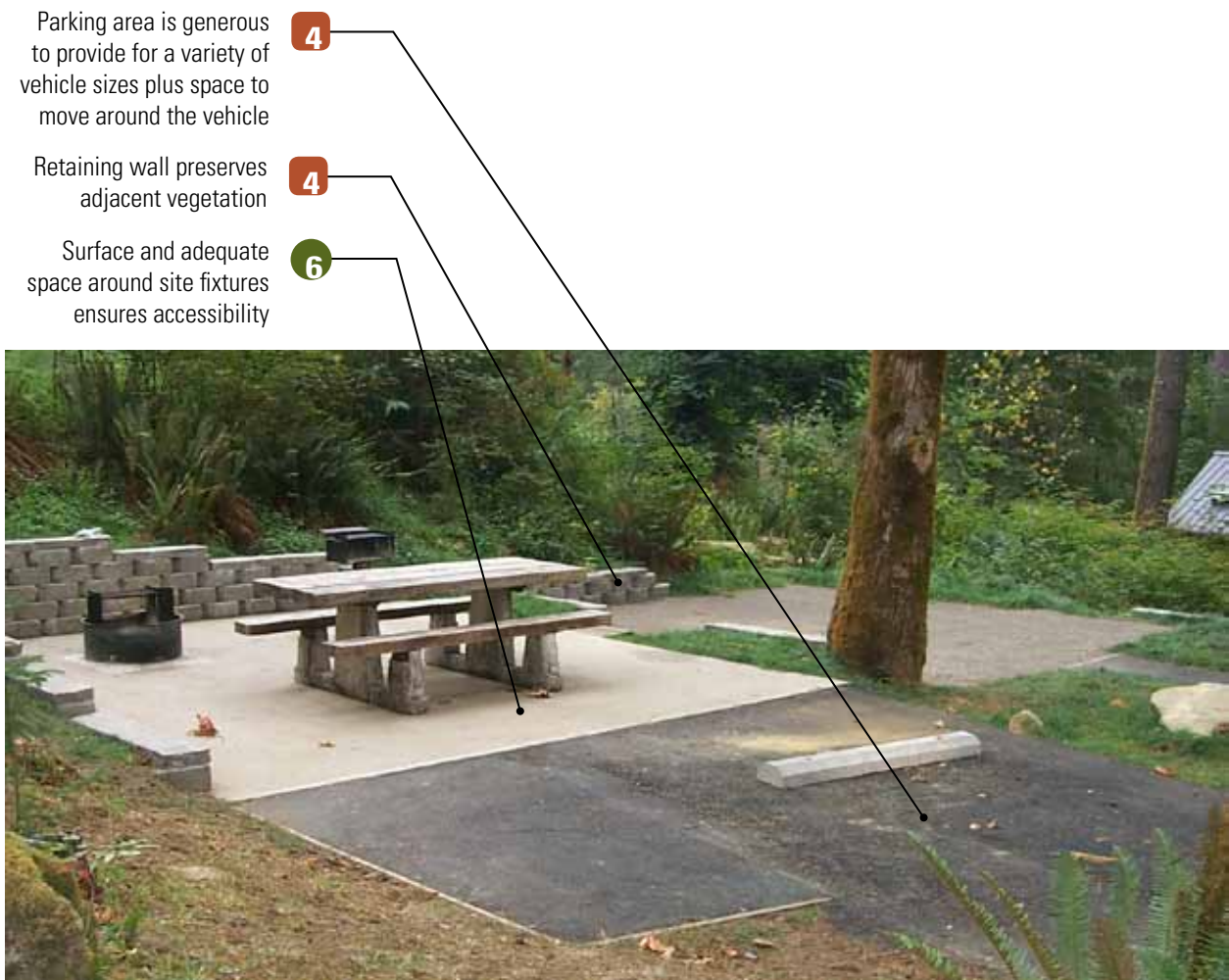
Loon Lake Campground, Oregon
