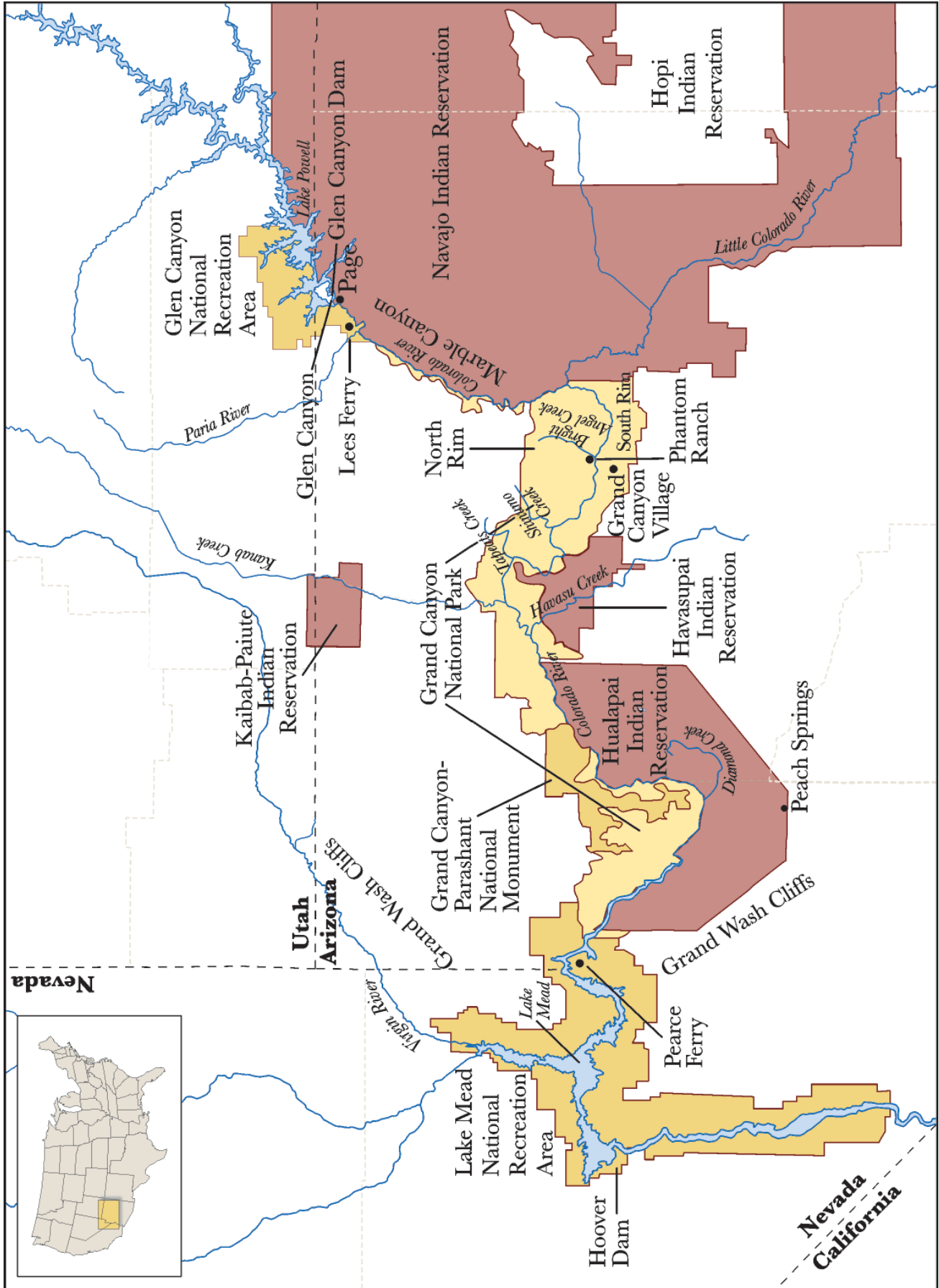
Figure 1. Study area.
