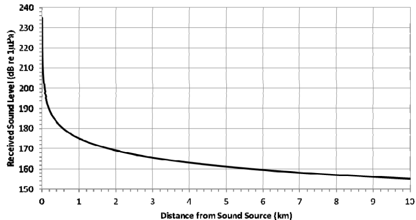
Figure 6-7. Estimate of Spreading Loss for a 235 dB re 1 μPa Sound Source Assuming Simple Spherical Spreading Loss
