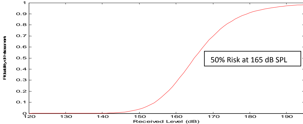
Figure 6-6. Behavioral Response Function Applied to Mysticetes (BRF 2 )
