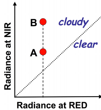
Figure 4. A schematic illustration of the REDvsNIR method for retrieving cloud optical depth and cloud fraction.
