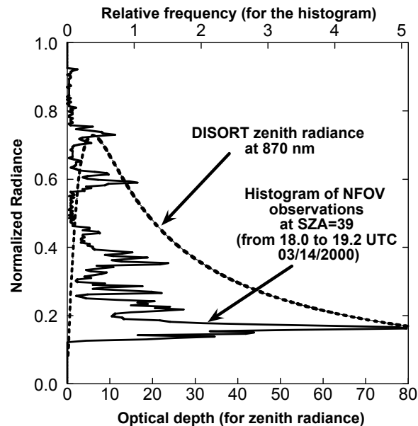
Figure 1. Downward 870-nm radiances vs. cloud optical depth (lower x-axis) calculated by the 1D radiative transfer model DISORT (Stamnes et al., 1988) with a surface albedo of 0.271. Co-plotted solid curve is a histogram (upper x-axis) of NFOV 870-nm radiances measured at the ACRF Oklahoma site from 18 to 19.2 UTC, March 14, 2000.
