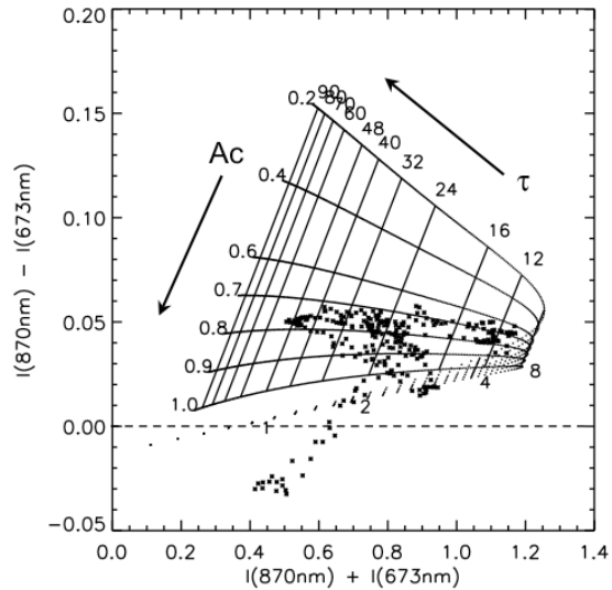
Figure 5. A lookup table (lines) constructed for SZA = 52^\circ , effective radius of 8 \mu\text{m} , and surface albedo values of 0.13 and 0.28 for RED and NIR channels, respectively. Dots are normalized zenith radiance measurements from the ACRF NFOV2 radiometer at the SGP site during 17.2 and 17.28 UTC on October 28, 2004. \tau is cloud optical depth and A_c is effective cloud fraction.
