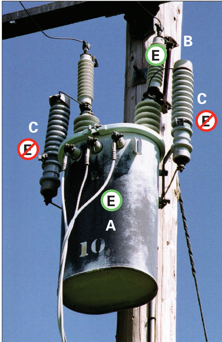
Figure 2-25 Transformer Mounted Lightning Arrester
