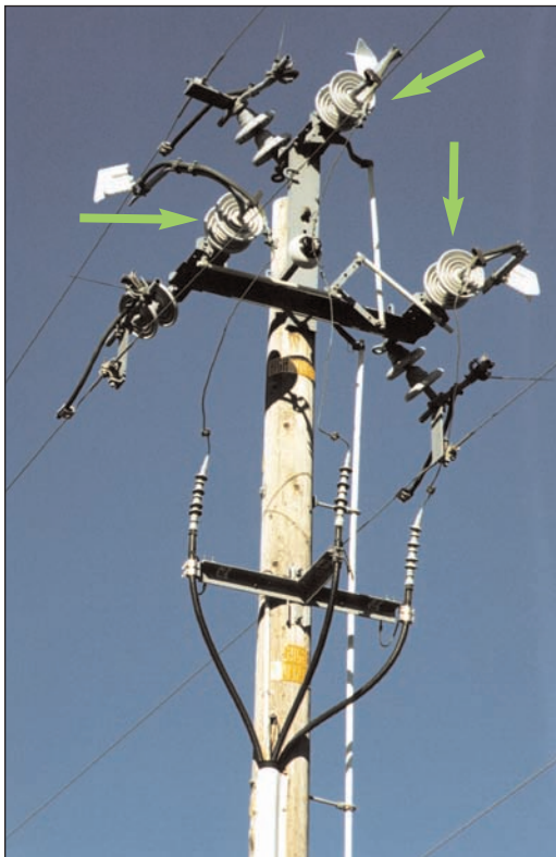
Figure 3-21 600 Amp KPF Air Switch, Triangular Construction (open position)
