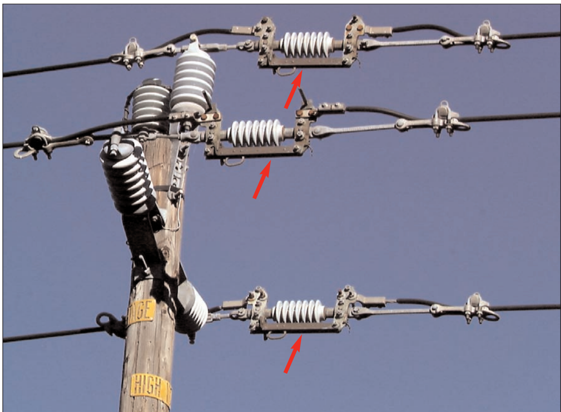
Figure 2-16 In-Line Disconnects (closed position)
