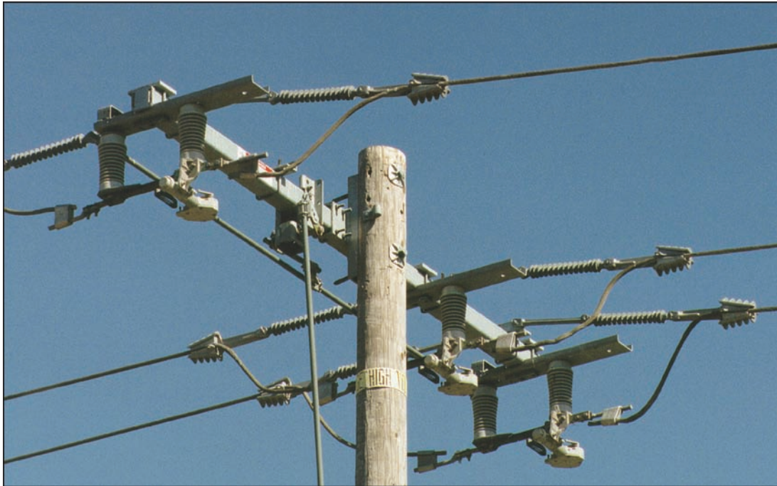
Figure 3-28 S&C 600 Amp Underarm Side-Break Switch (closed position)
