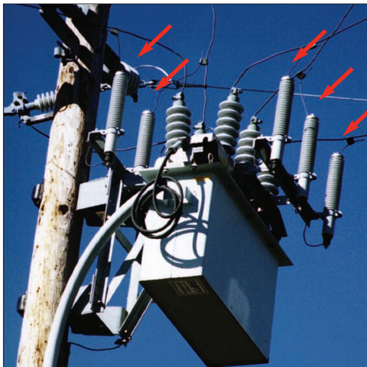
Figure 2-20 Lightning Arrester (with Recloser)
