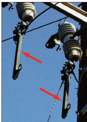
Figure 2-13 Solid Blade Disconnects
