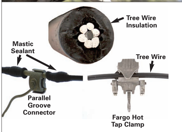
Figure 3-55 Tree Wire Detail
