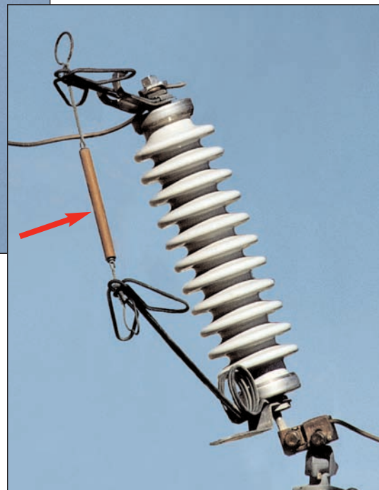
Figure 2-7 Close up of Open Link Fuses
