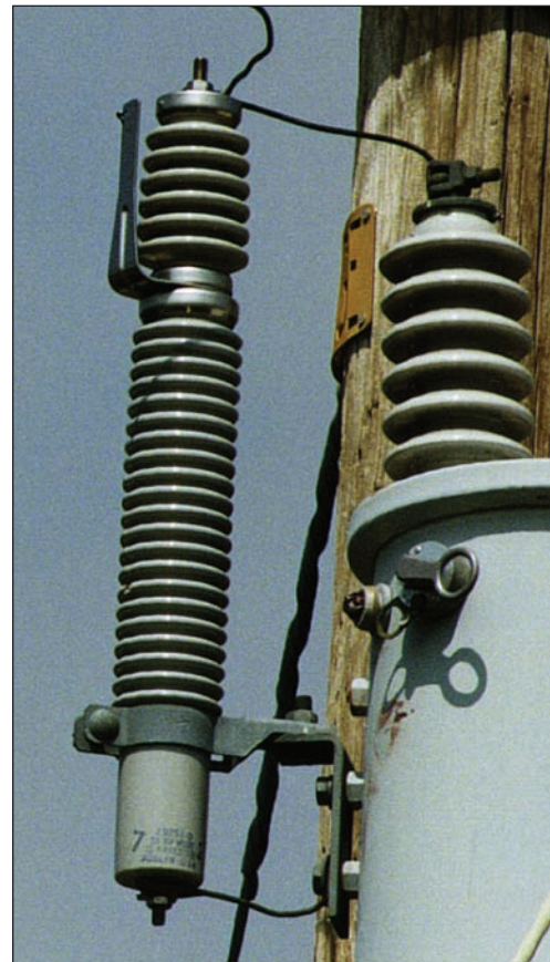
Figure 2-26 Gapped Lightning Arrester
