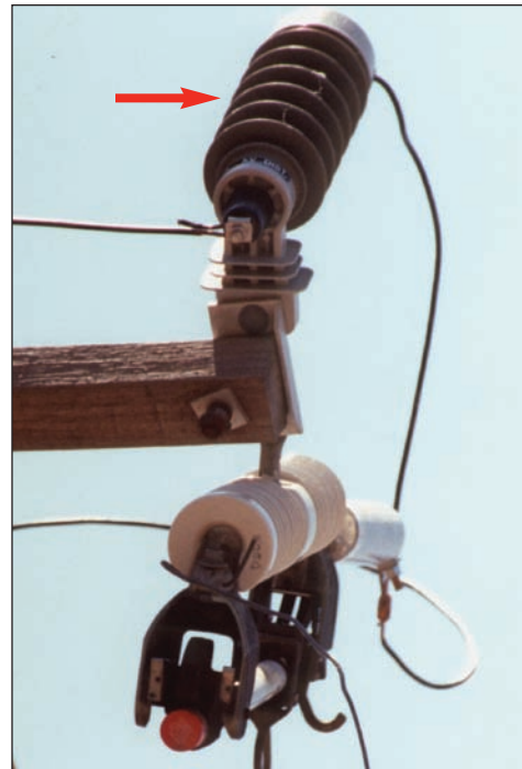
Figure 2-23 Non-Porcelain Lightning Arrester
