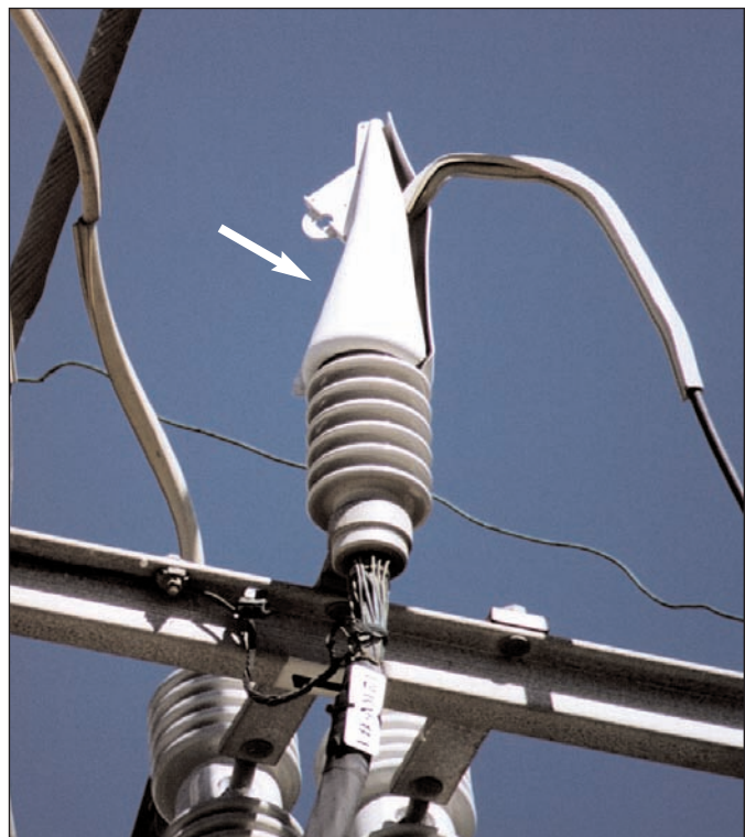
Figure 4-21 Close up of Squirrel Guard
