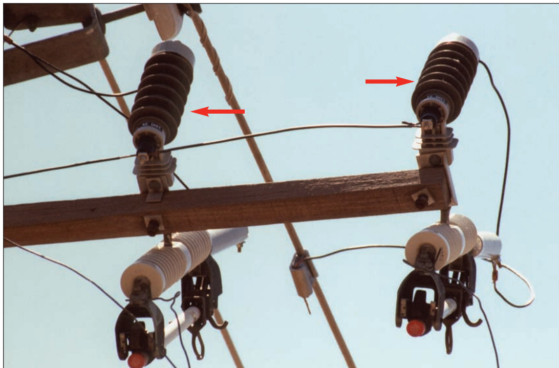
Figure 2-24 Non-Porcelain Lightning Arrester
