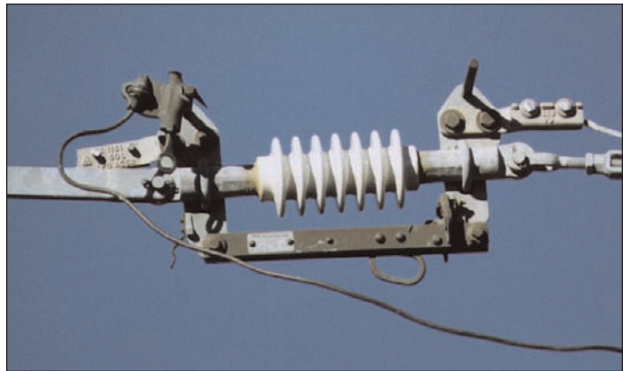
Figure 2-15 In-Line Disconnect (closed position)
