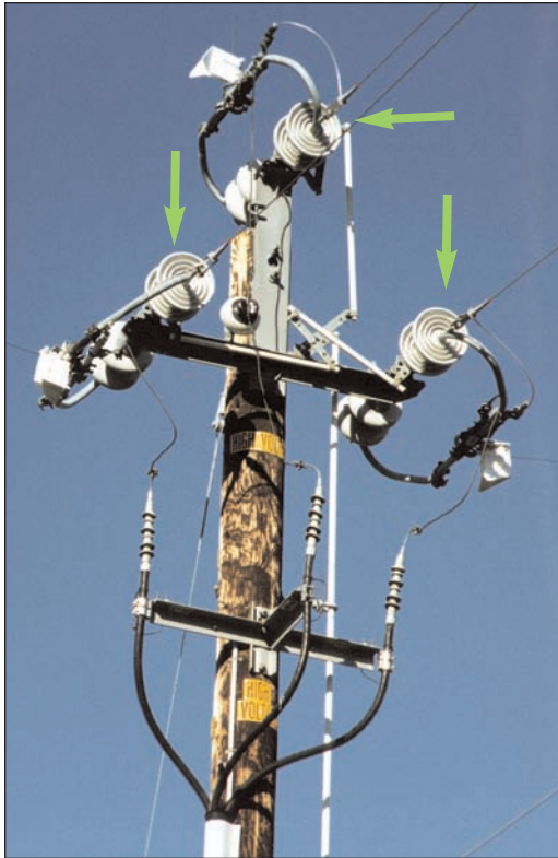
Figure 3-20 600 Amp KPF Air Switch, Triangular Construction (closed position)
