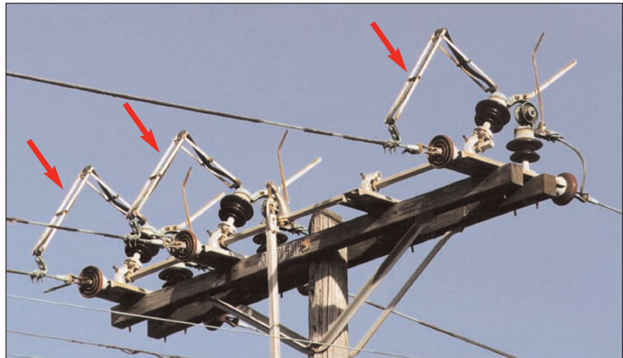
Figure 2-38 Grasshopper Air Switch (closed position)
