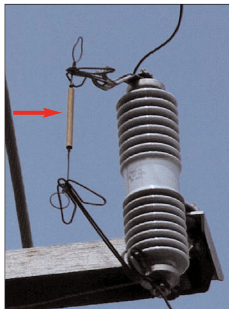
Figure 2-5 Open Link Fuse
