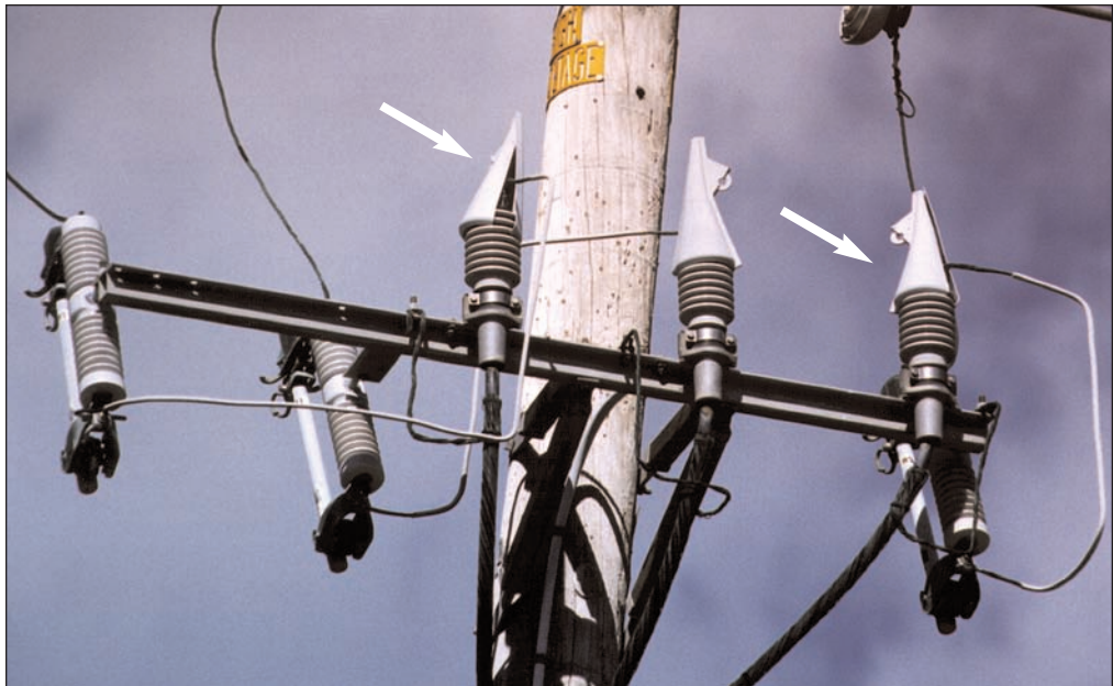
Figure 4-20 Squirrel Guard
