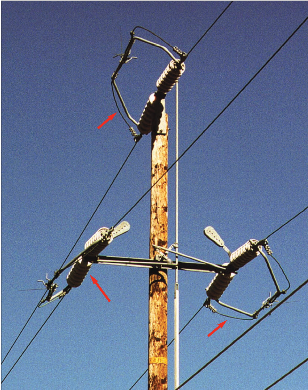
Figure 2-40 Transmission Air Switch, Pole Mounted 60kV (closed position)
