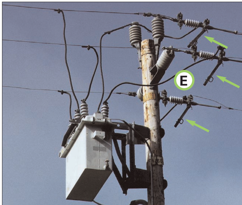
Figure 3-36 Recloser with In-Line Disconnects (open position)
