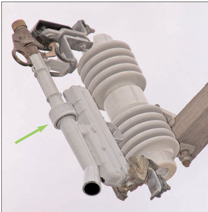
Figure 3-18 S&C Fault Tamer Fuse (Closed)
