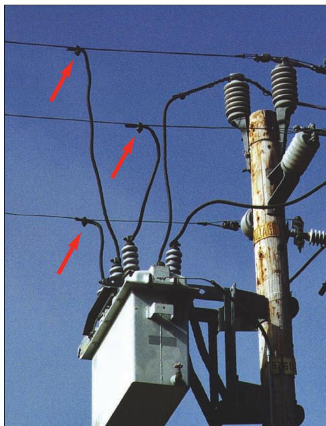
Figure 2-34 Split Bolt Connectors
