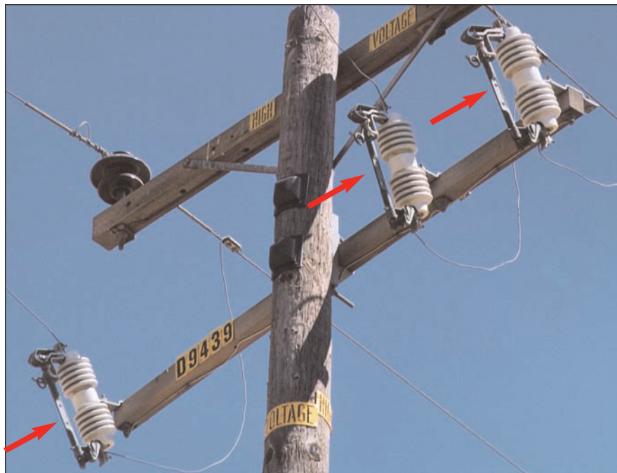
Figure 2-11 Arm Mounted Cutout with Solid Blade Disconnect (closed position)
