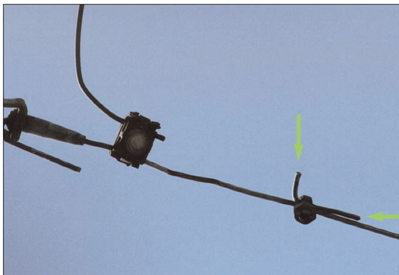
Figure 3-58 Close Up of Non-exempt Split Bolt and Copper Parallel Groove Connector
