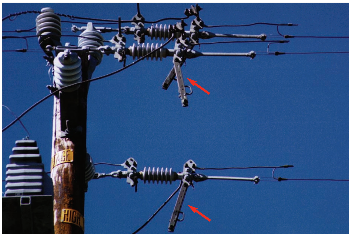
Figure 2-18 In-Line Disconnects (open position)
