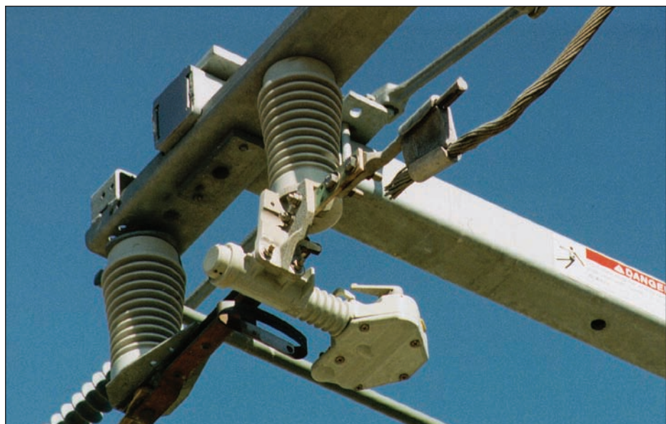
Figure 3-29 S&C 600 Amp Underarm Side-Break Switch (closed position)
