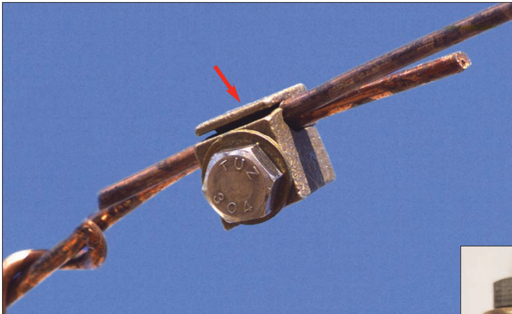
Figure 2-35 Fargo Connector
