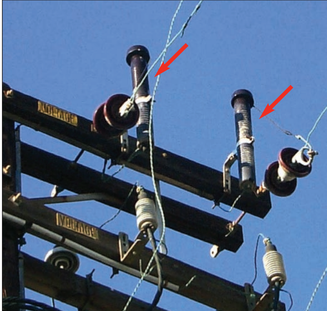
Figure 2-27 Lightning Arrester
