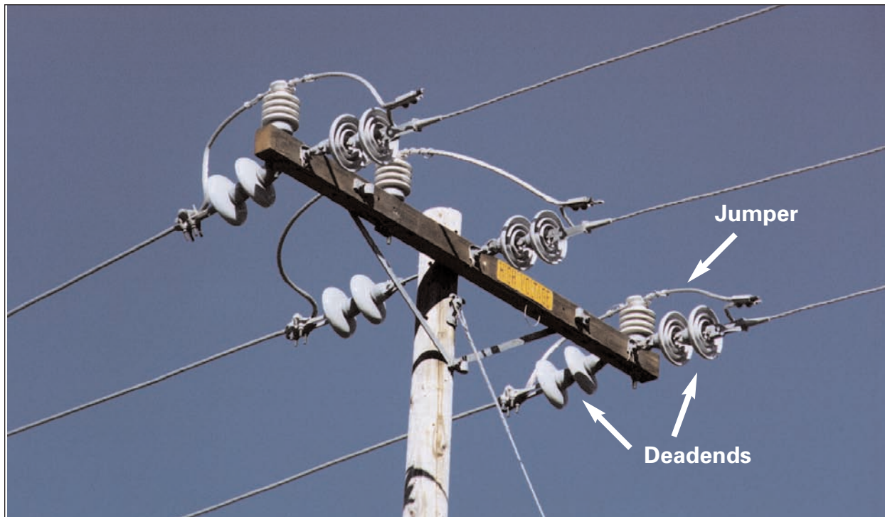
Figure 4-7 Crossarm Double Deadend
