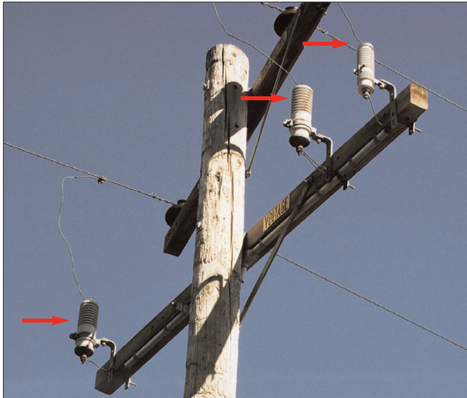
Figure 2-21 Lightning Arrester
