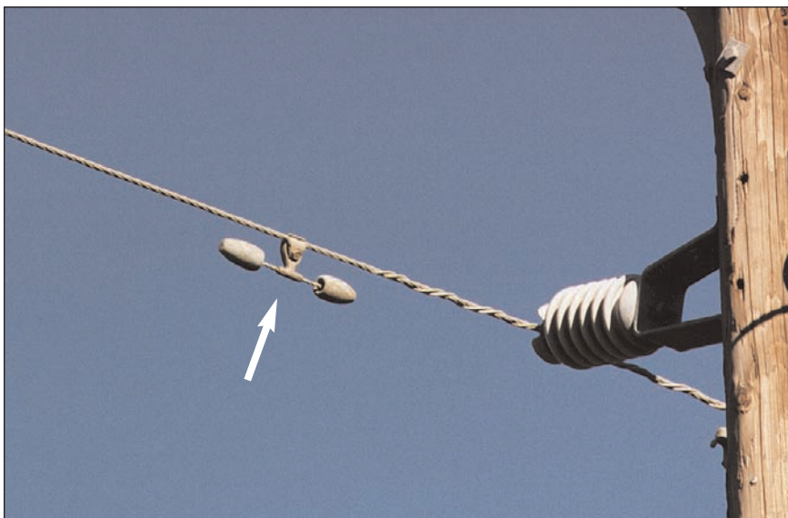
Figure 4-14 Vibration Damper
