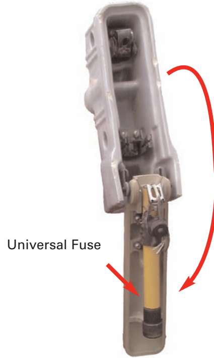
Figure 2-9 Open 4KV Cutout
