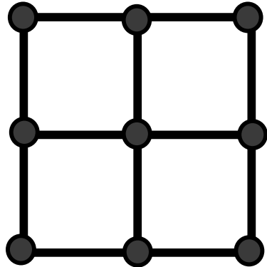
9-point stencil
