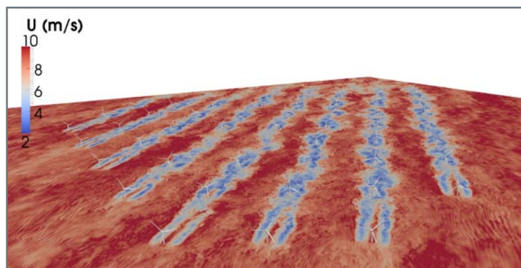
Figure 1. NREL fluid dynamics simulation of the operational 48-turbine Lillgrund wind plant. The contour plane shows velocity in a plane taken at hub height (offset to below hub height for clarity) where blue contours highlight the turbine wakes interacting with downwind turbines.
