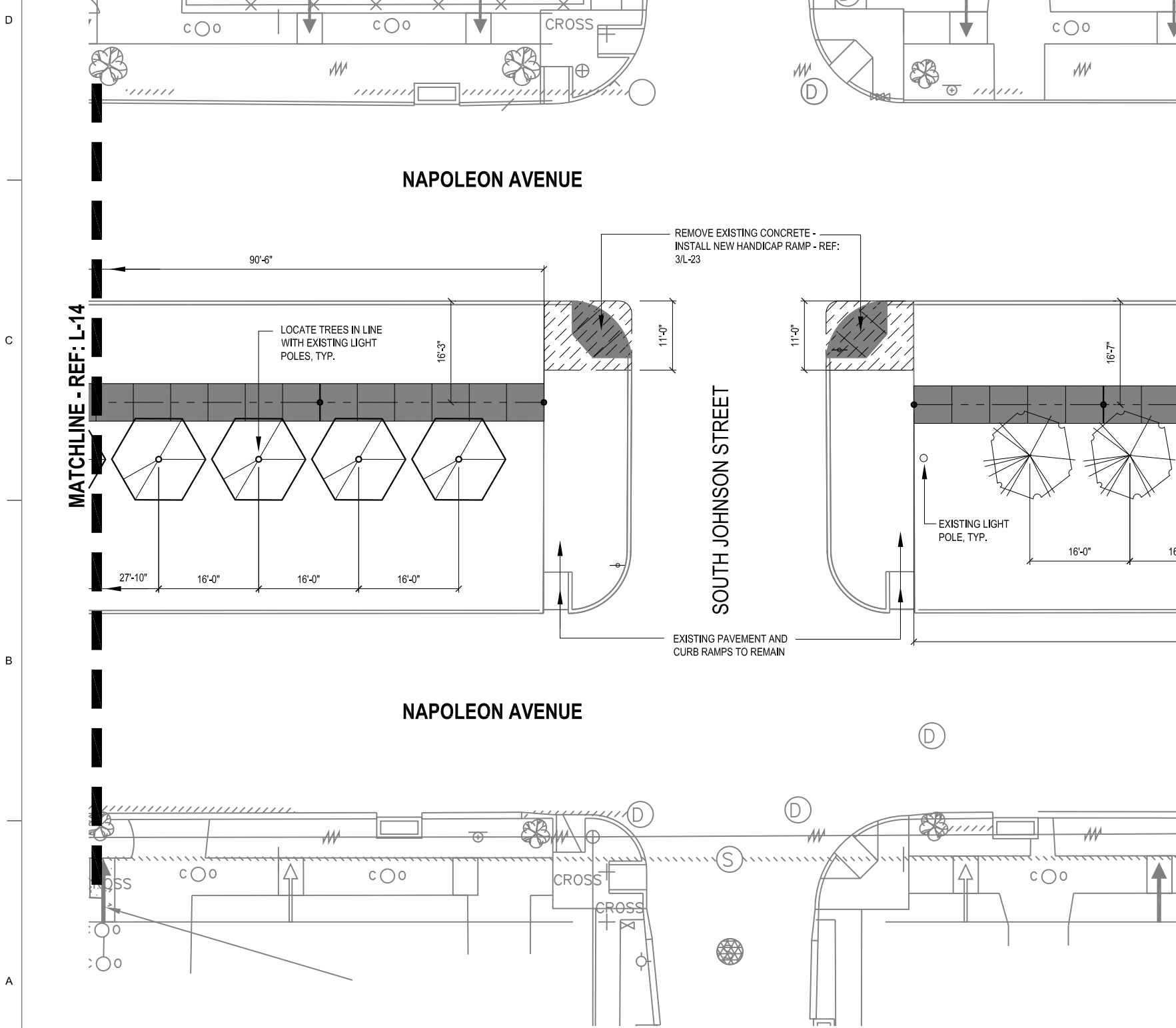
1 LAYOUT AND MATERIALS PLAN PLAN
