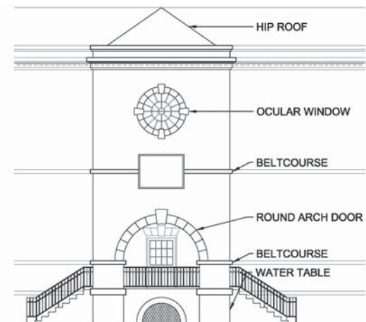
The Storehouse (1827) at Augusta Arsenal, Georgia, has the dominant tower with round-arched entrance. Apart from the window hoods, the features of the tower are shown below.
