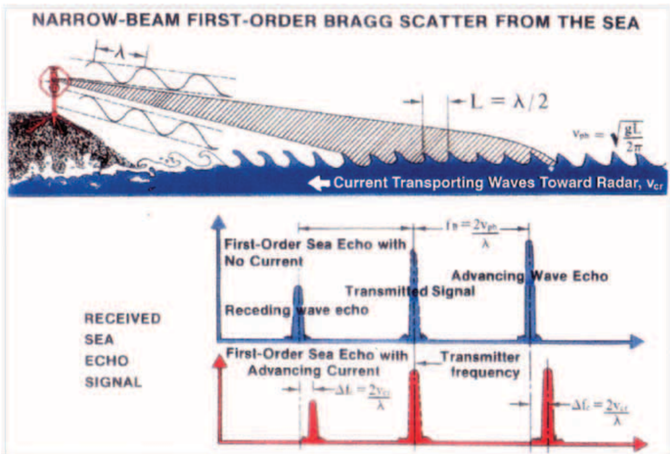
Figure A-1: HFR Backscattering from Ocean Waves for Current Velocity Measurement.
