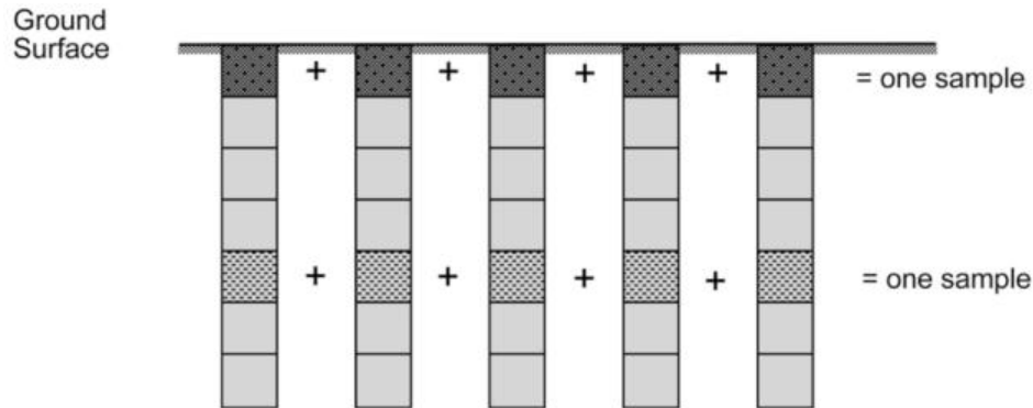
Figure 29. Schematic of procedure to collect multiple-increment profile samples where transport and deposition of energetic materials is suspected.
