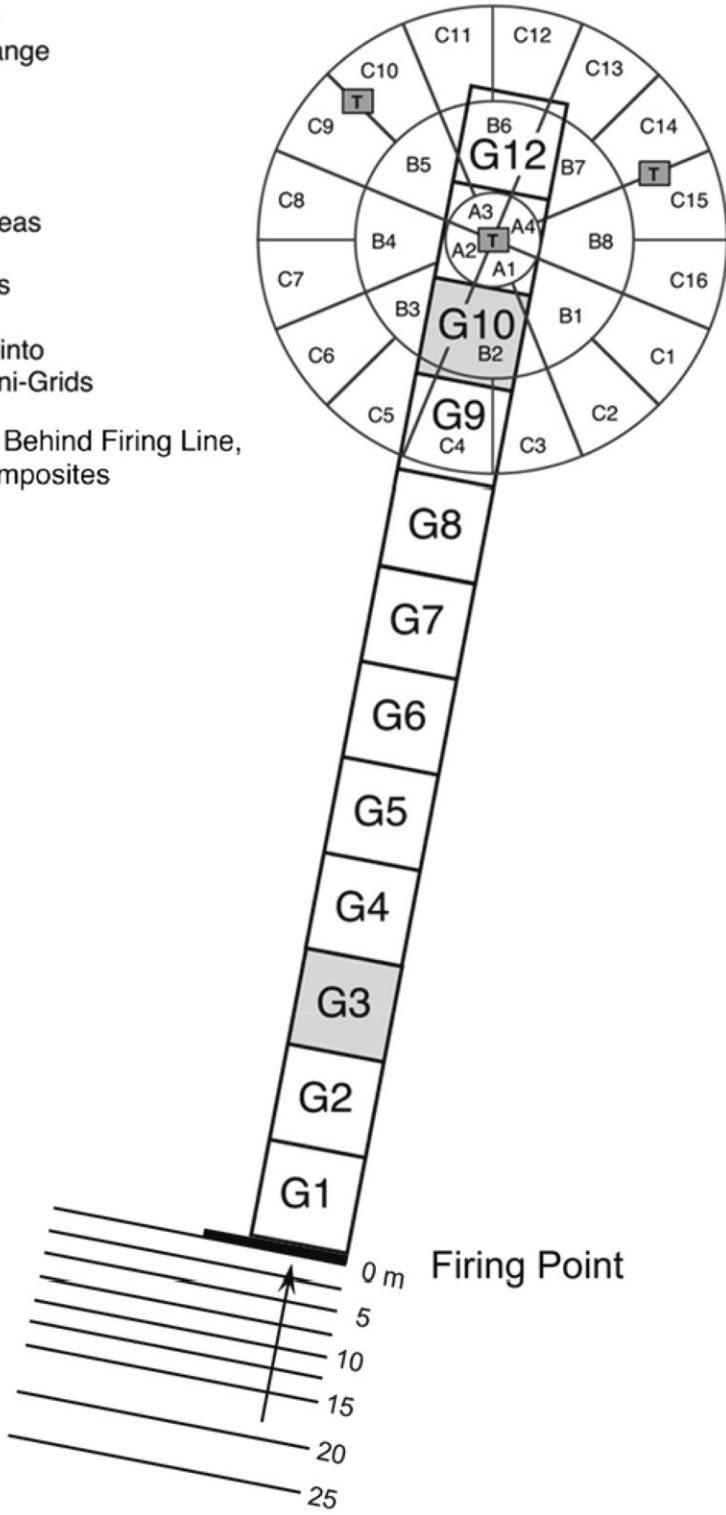
Figure A3-5. Twelve 10-m x 10-m grids located in a direct line from the firing point to and beyond the center target and halo sampling areas around target. Also shown are the positions of lines where composite samples were collected behind the firing line (Jenkins et al. 2004).
