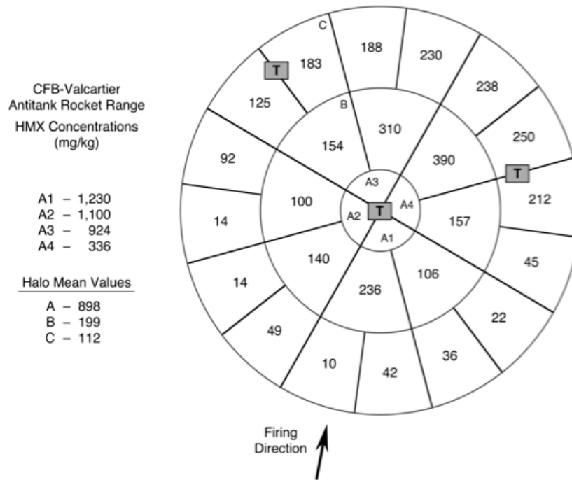
Figure 10. Distribution of HMX residues surrounding target vehicles at Valcartier, using an older-style sampling design. Target positions are indicated by gray-shaded rectangles marked with a “T.” Sampling halos were divided at radii of 5 m (A), 5 –15 m (B), and 15 –25 m (C).
