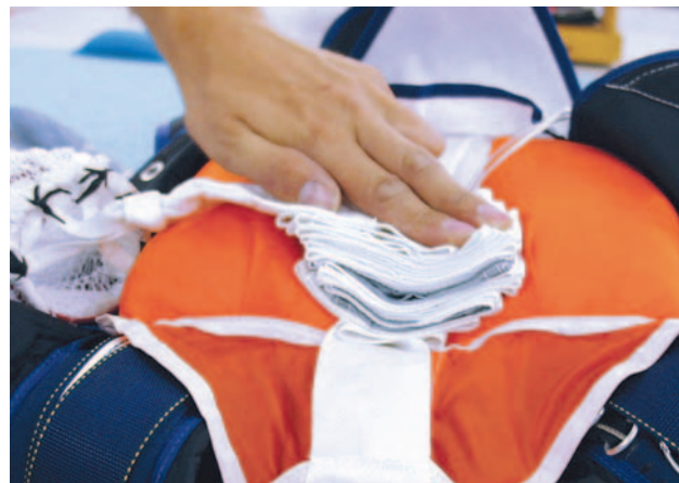
Figure 5-105. "S" fold the bridle on bag.
