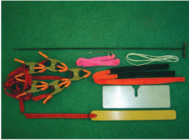
Figure 5-69. Ram-air canopy packing tools.
