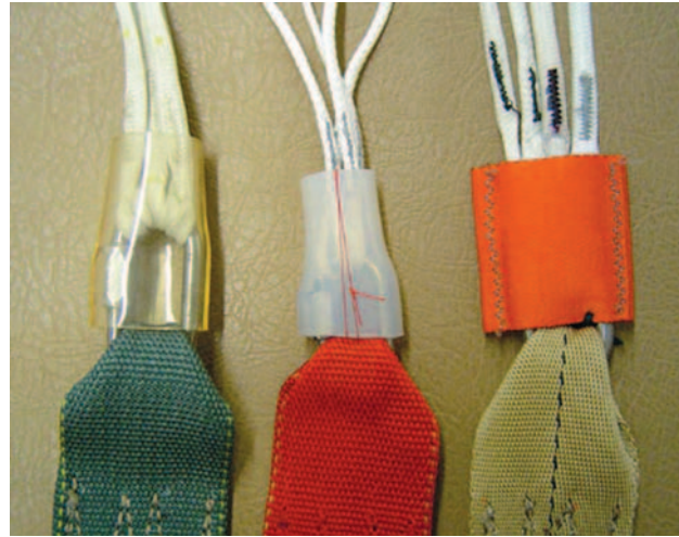
Figure 5-24. Slider bumpers.
