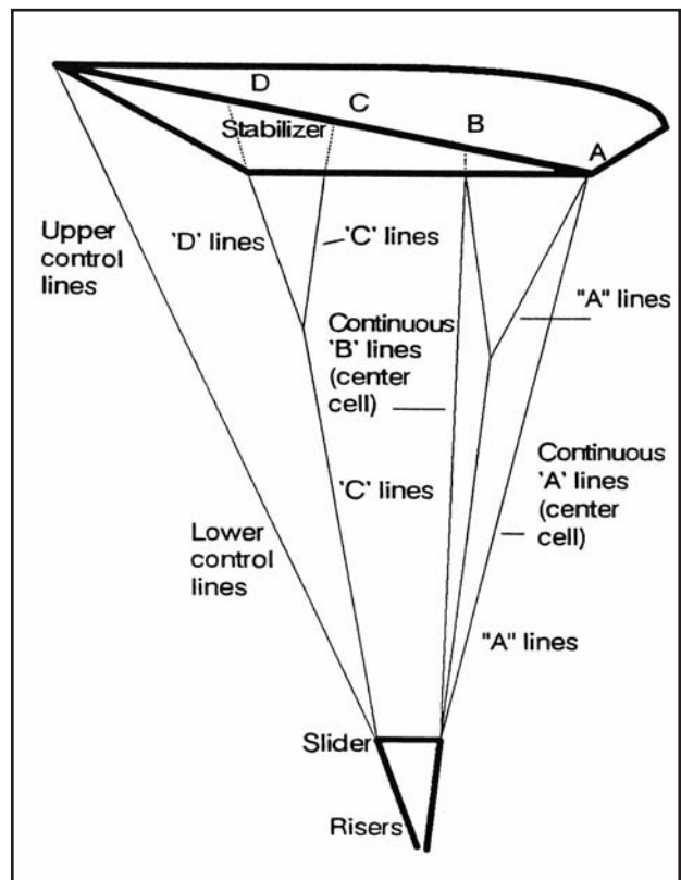
Figure 5-23. Ram-air canopy layout and nomenclature.
