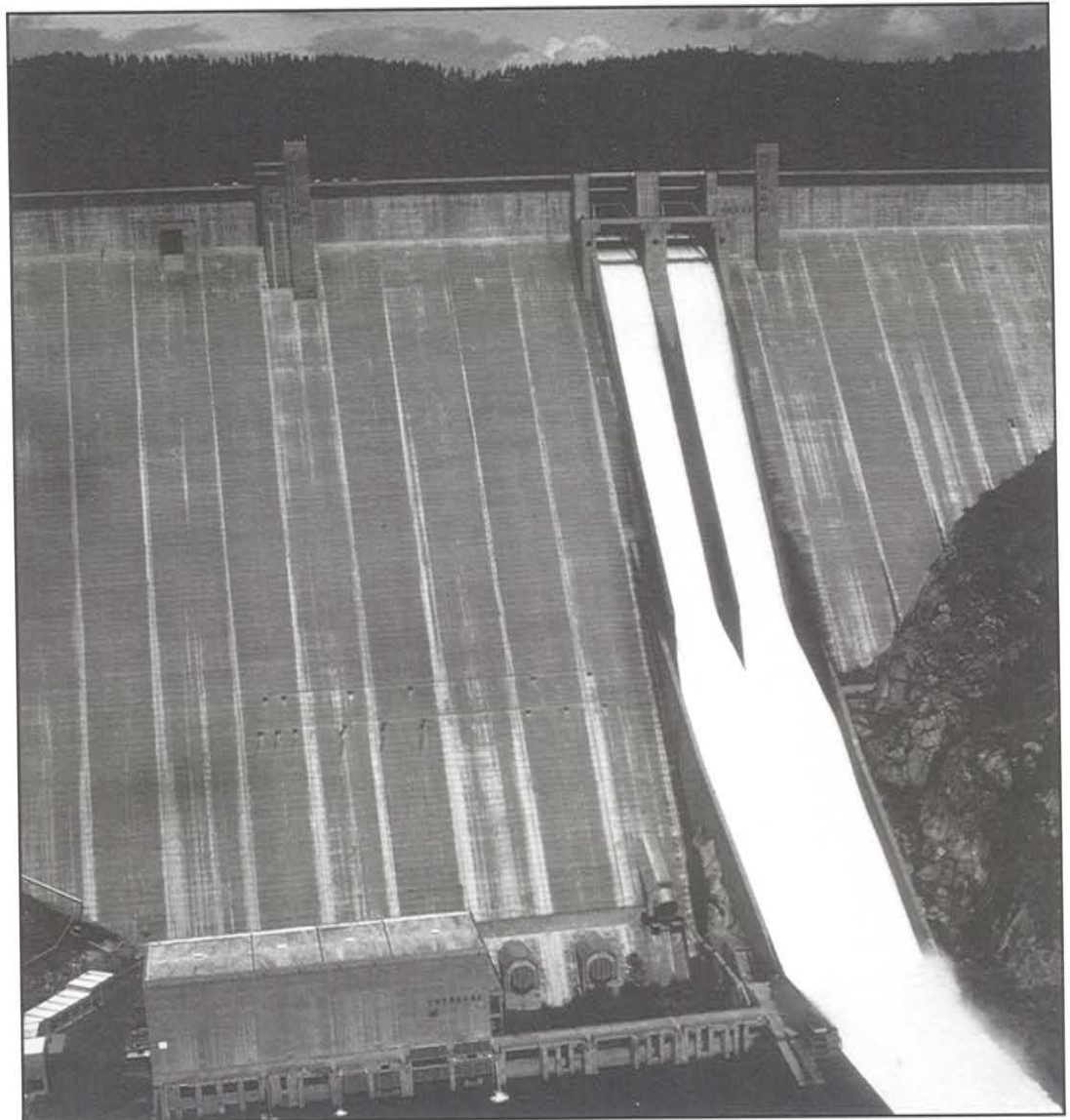
During high system loads, spill at Dworshak is sometimes needed to move water to the lower Snake River projects. This increases flows at these four projects resulting in more power to serve short-term needs.
