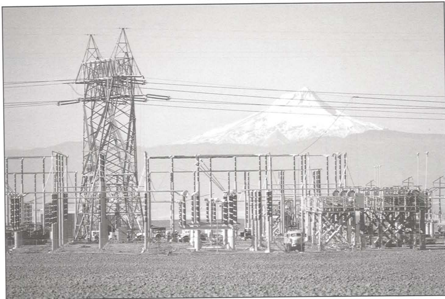
Serving electrical loads in the Pacific Northwest is frequently complicated by having most of the generation capability east of the Cascade Mountain Range while major load centers are west of this range. Transmission system overload and voltage instability are just two concerns engineers and operators worry about.
