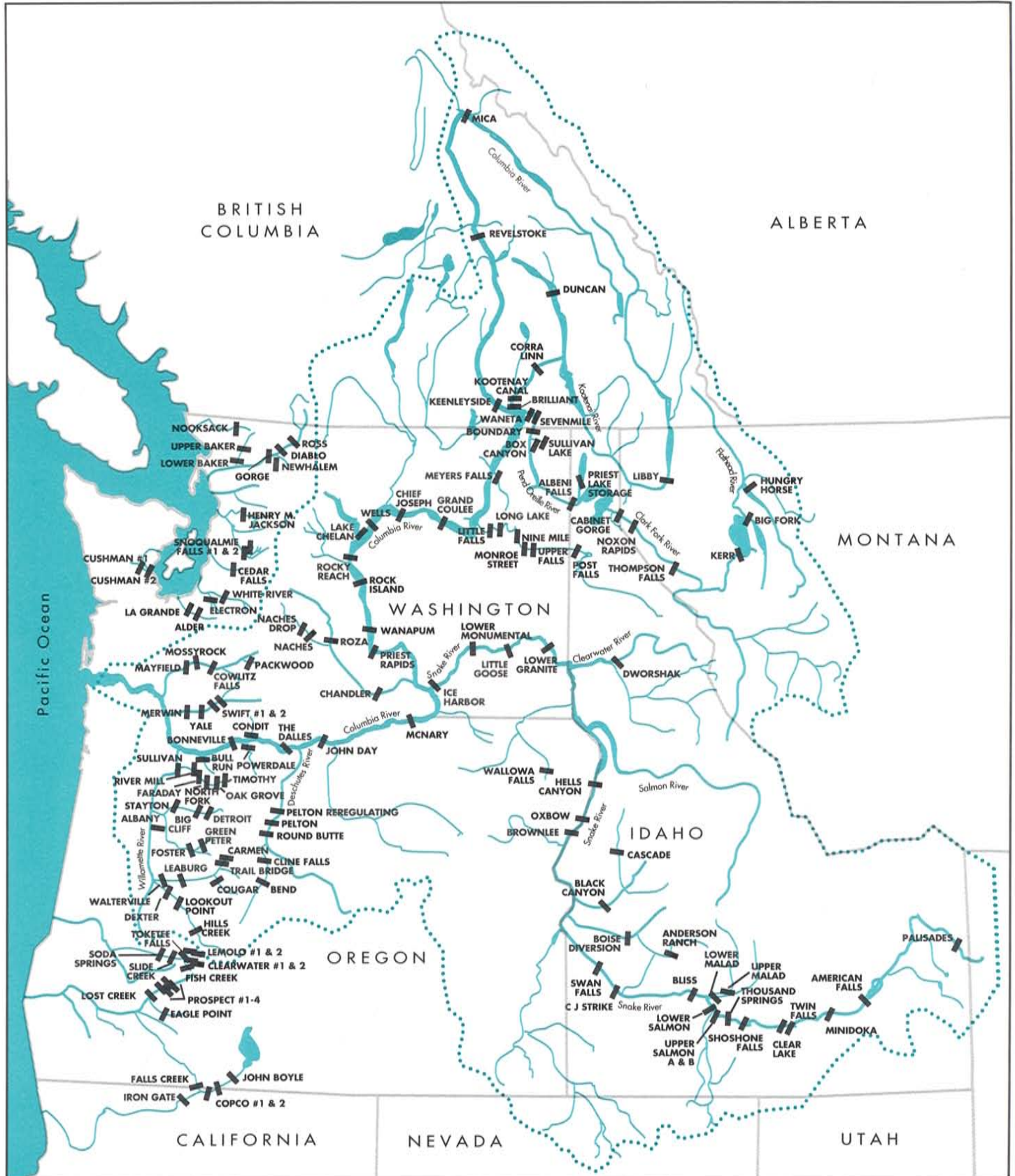
All projects store and release water to regulate the rivers' natural flow patterns to conform more closely to hourly, daily, and weekly needs for electric power and the needs of other short-term uses. This map shows the major hydroelectric dams in the Pacific Northwest.
