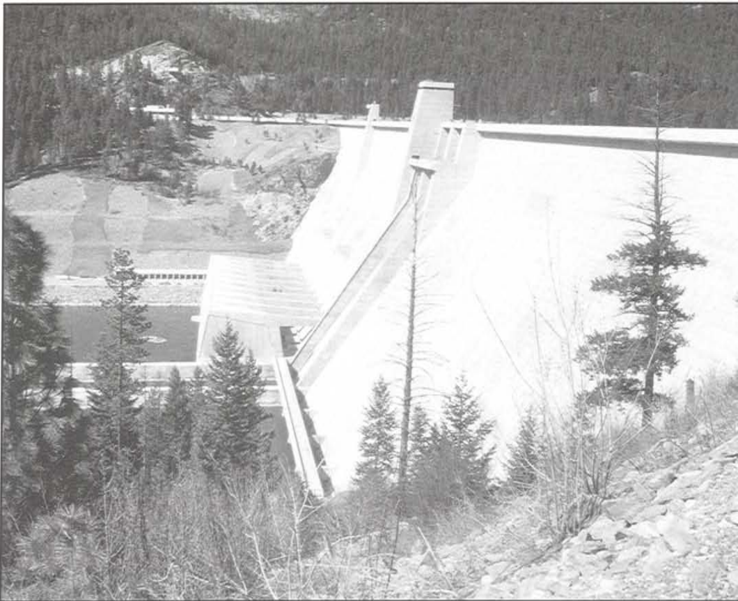
Libby project in Northwest Montana is a large headwater dam whose operation reflects U.S. and Canadian cooperation on power generation, flood control, and other uses. It was one of four projects allowed under the Columbia River Treaty and backs up water in the Kootenai (U.S. spelling) or Kootenay (Canadian spelling) River from Montana into Canada.
