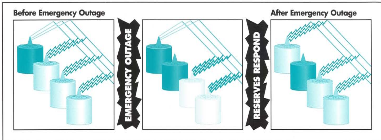
During normal circumstances, some turbines are kept at the ready for emergency use. If a generator goes out of service suddenly, spinning reserves are called into action to quickly meet the load the failed generator was carrying.
