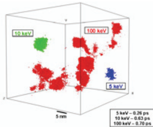
Molecular dynamics simulation of radiation damage cascades in iron
