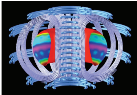
3-D ITER equilibrium
