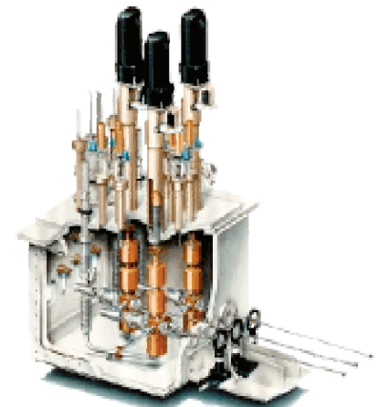
High-speed hydrogen pellet injector for fueling fusion devices
