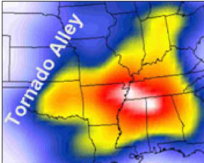
Figure 8. Relative frequency of killer tornado events, 1950-2004. White area indicates area with greatest frequency of tornado-related fatalities during the period. Red area had the second greatest frequency of tornado-related fatalities. © Copyright [2007] American Meteorological Society (AMS).
