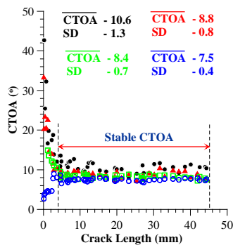
Effect of image analysis on CTOA
