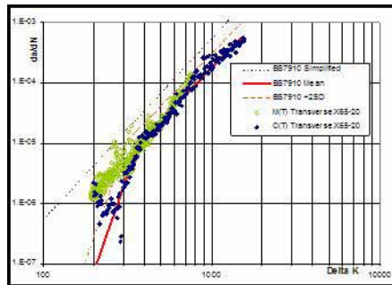
Comparison of C(T) and M(T) FCGR results for X65 steel to BS 7910 design standard.
