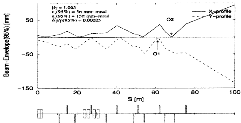
Figure 2.6.3 Beam envelope.
