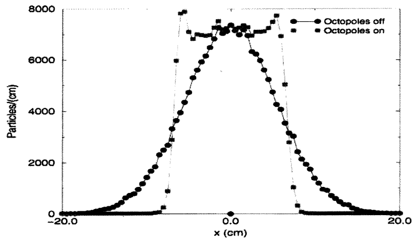
Figure 2.6.4a. Horizontal beam profile at target
