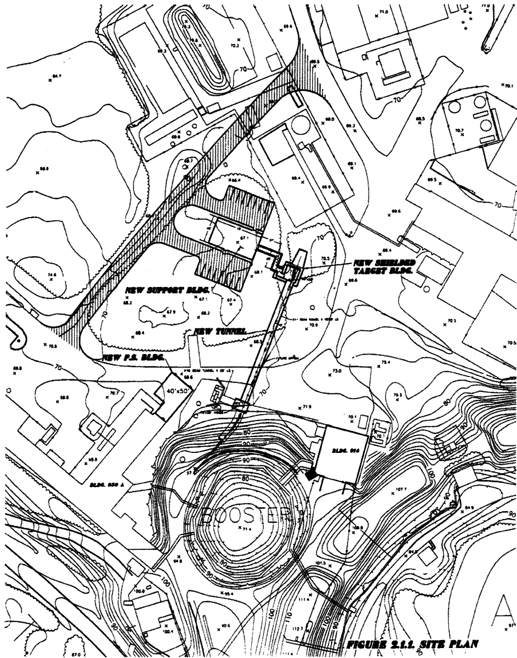
FIGURE - 2.1.1 - SITE PLAN
