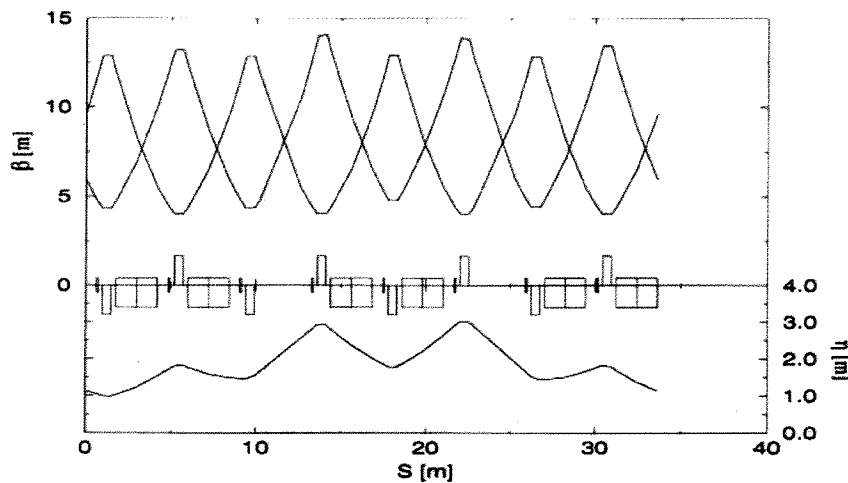
Figure - 2.3.2 AGS Booster lattice functions
