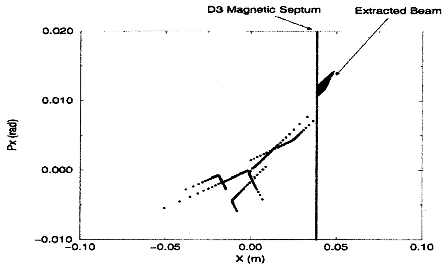
Figure - 2.3.3a Phase space at D6.
