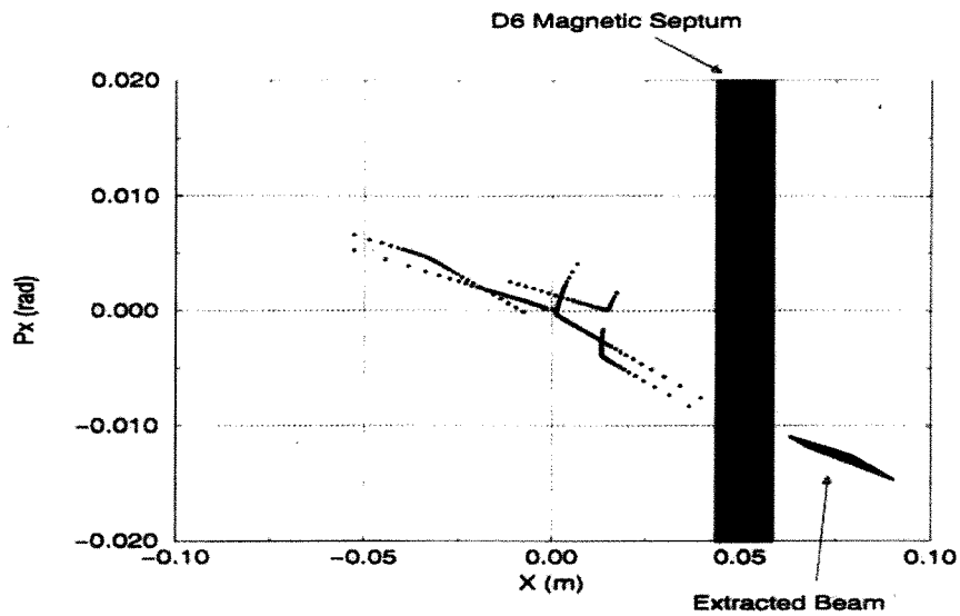
Figure - 2.3.3b Phase space at D6.
