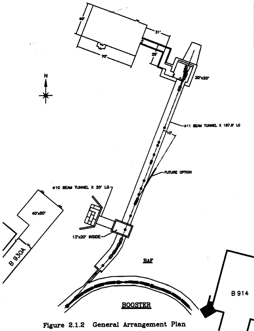
FIGURE - 2.1.2 - GENERAL ARRANGEMENT PLAN
