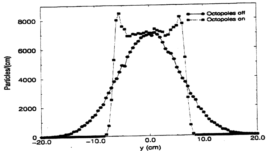
Figure 2.6.4b. Vertical beam profile at target
