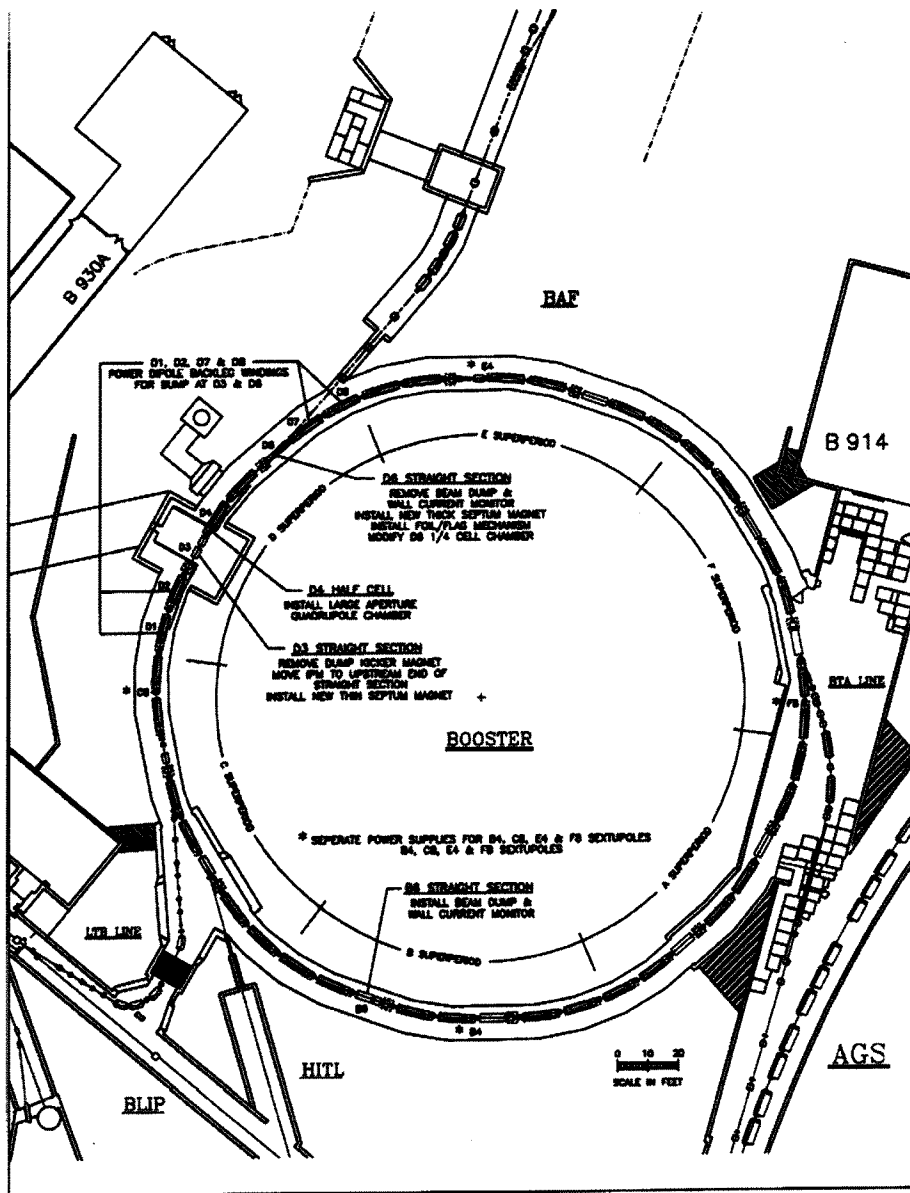
FIGURE 2.3.1 - BOOSTER MODIFICATION FOR SLOW EXTRACTED BEAM
