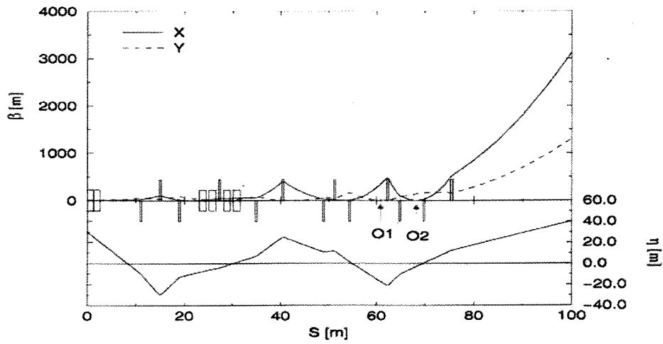
Figure 2.6.2 Optics of the beam transport line.
