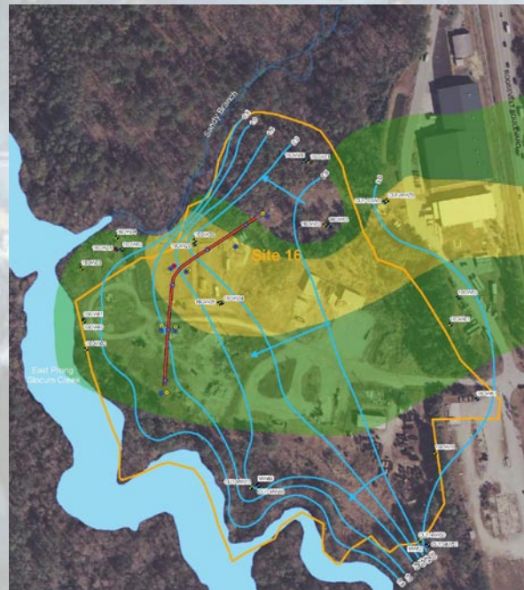
Site location and orientation of the PRB to intercept migrating groundwater prior to discharge to Slocum Creek.
