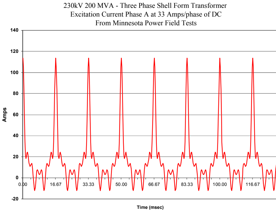
Figure A4-13. Excitation current from 230kV 3-phase shell form transformer with GIC present.
