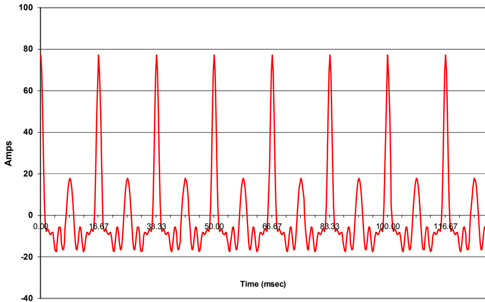
Figure A4-16. Measured neutral current for 3-phase shell form transformer with GIC present.
