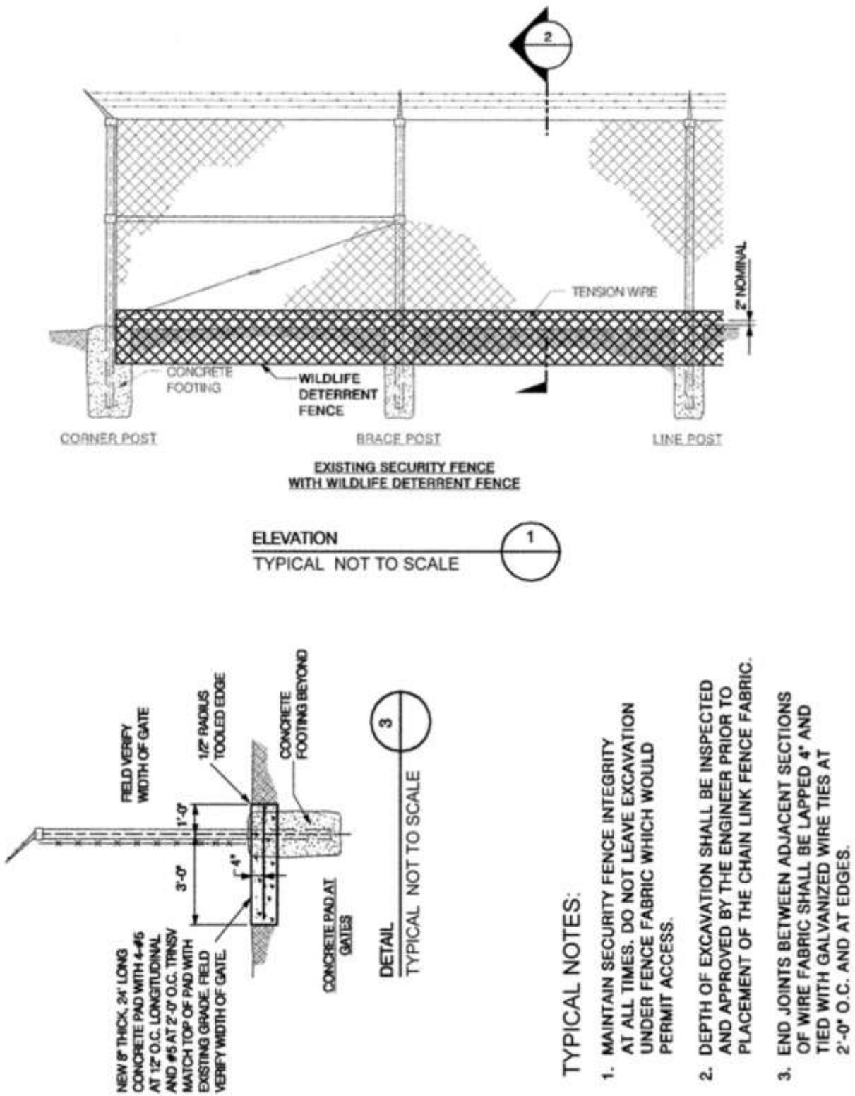
Figure 1 Example of Wildlife Deterrent Fence Details
