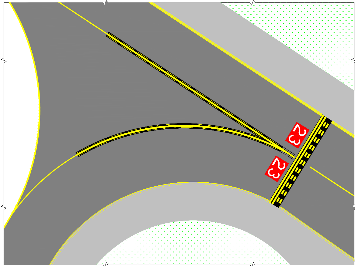
Figure C - 10. Intersection of Two Taxiways at Runway End
