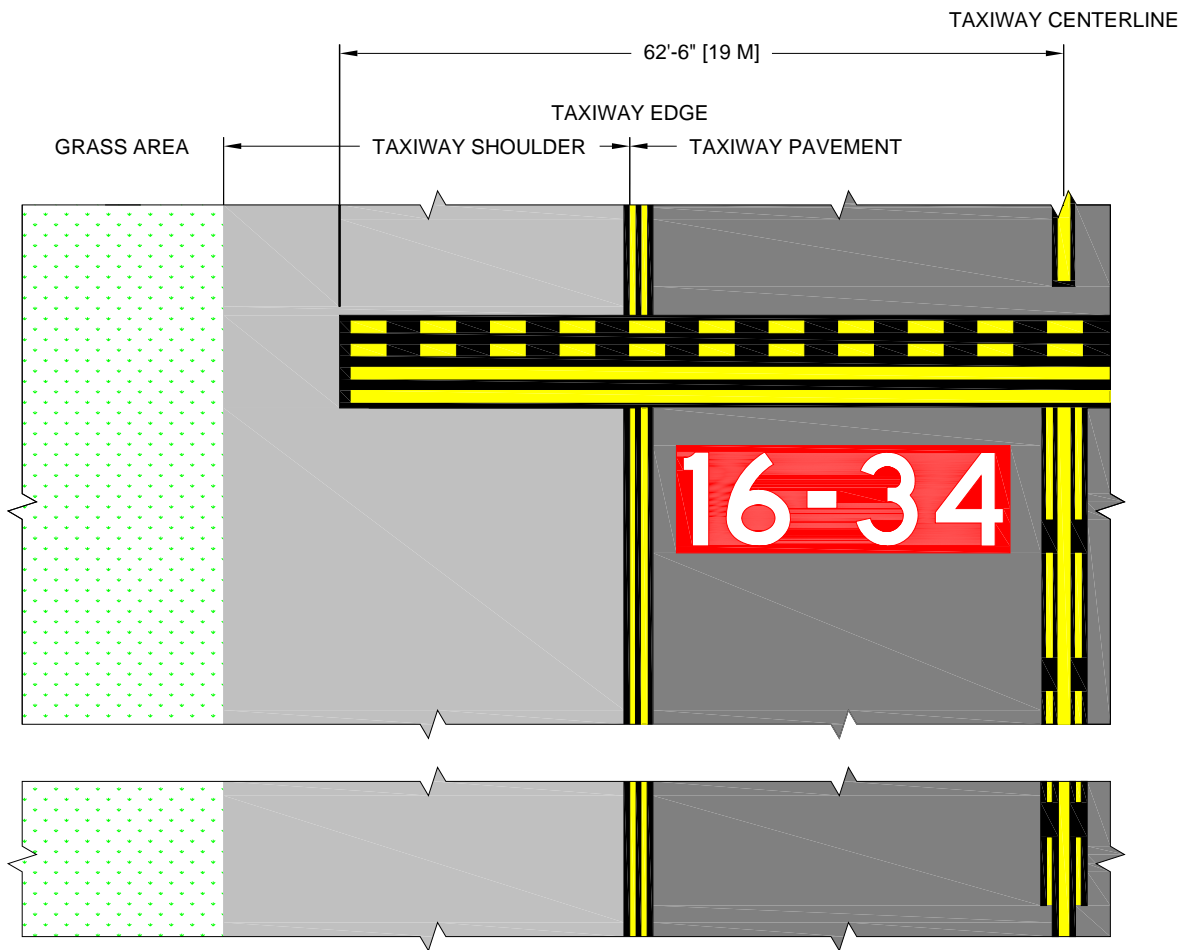
Figure C - 4. Enhanced Runway Holding Position Markings on Taxiways
