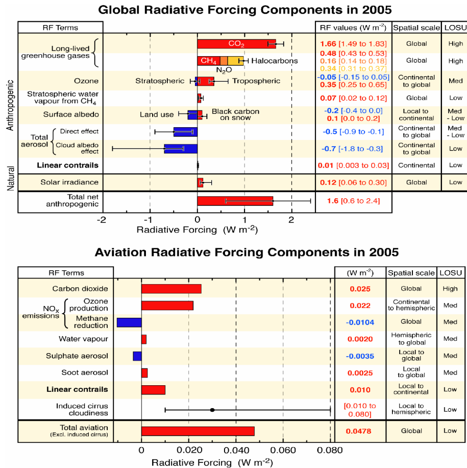
Figure 1.1: (Top panel) Global mean radiative forcing (RF) components for the period 1750 to 2005 from Forster et al. (2007). The components implicitly include all aviation emissions and effects except linear contrails, which are shown as a separate term. (Bottom panel) Global mean RF components for aviation emissions and effects as evaluated for 2005, based on Sausen et al. (2005). Note that the linear contrail components in the two panels are equal. In each panel the columns display the RF spatial scales and the levels of scientific understanding. Note that the total aviation induced radiative forcing does not include radiative forcing due to induced cirrus cloudiness due to low level of scientific confidence.
