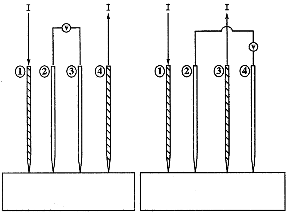
Standard Probe Configuration (ASTM F-84)
