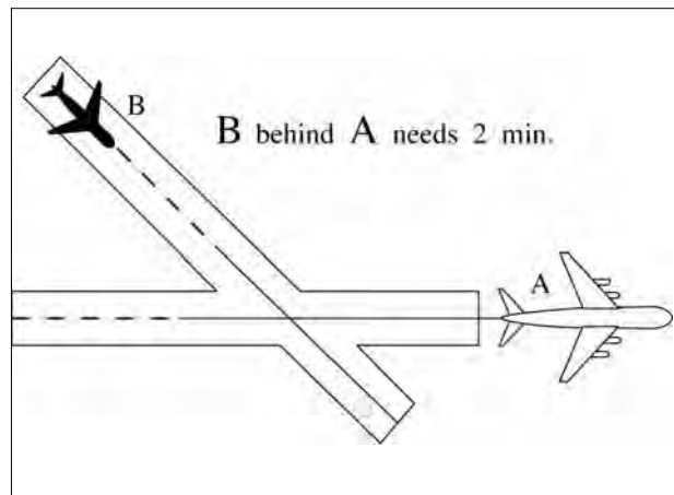
FIG 3-9-9 Crossing Runways
