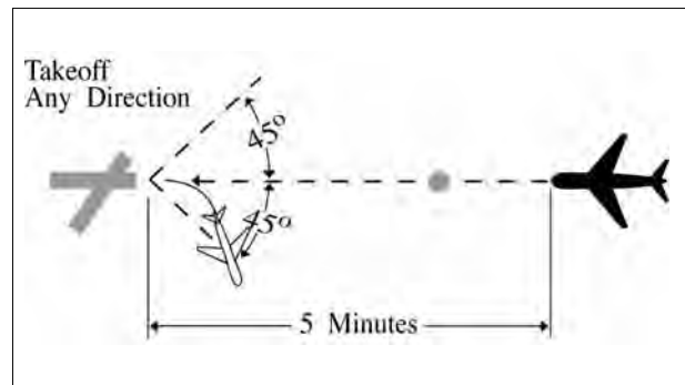
FIG 6-3-2 Separation Minima
