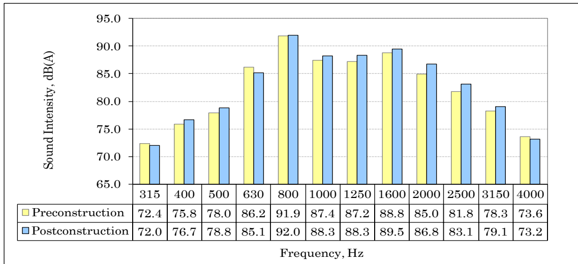
Figure 15. Mean A-weighted sound intensity frequency spectra.
