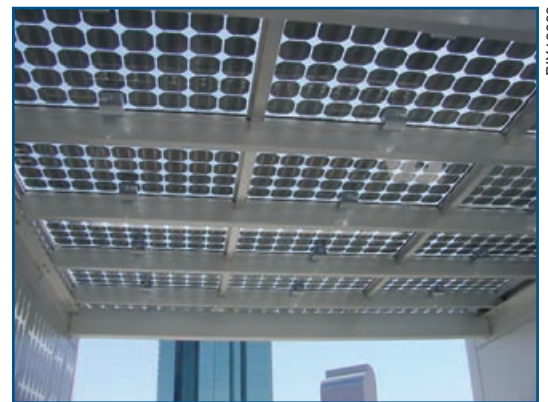
Building-integrated PV is located along the roof of the building. The PV cells are sandwiched in translucent glass panels and mounted horizontally to form seven shaded bays at the penthouse level.
