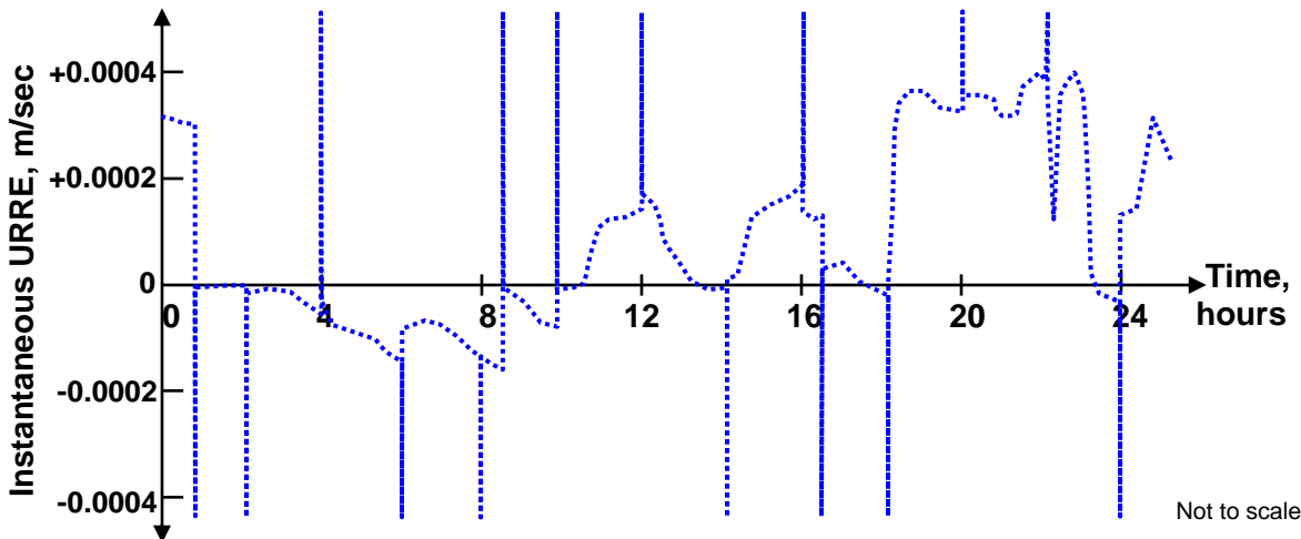
Figure A.4-5b. Instantaneous SPS SIS URRE as a Function of Time
