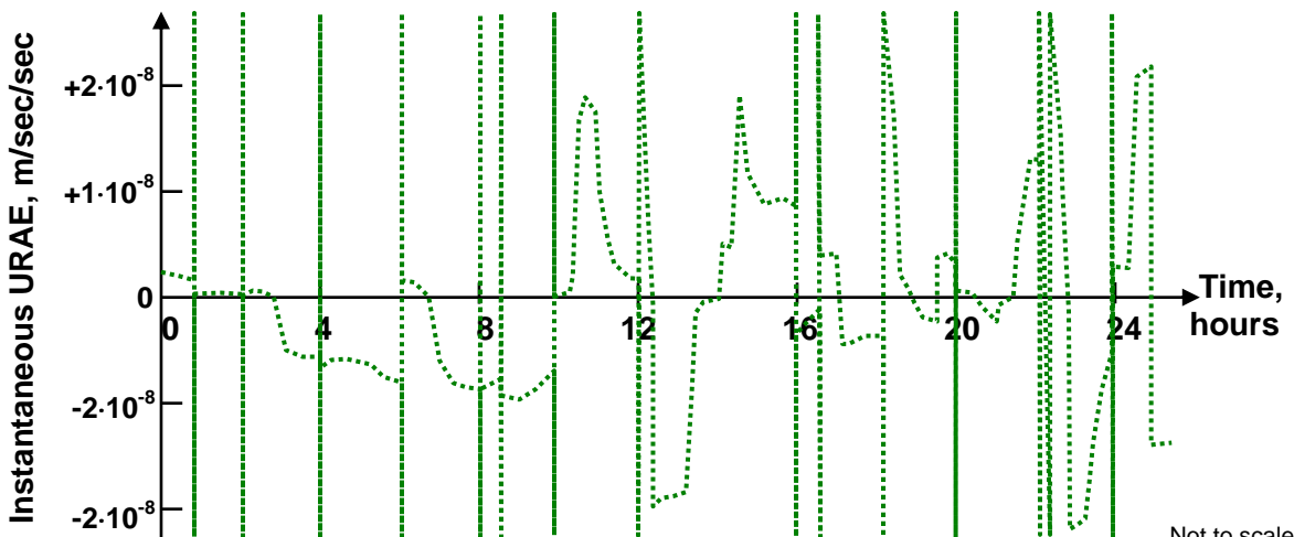
Figure A.4-5c. Instantaneous SPS SIS URAE as a Function of Time
